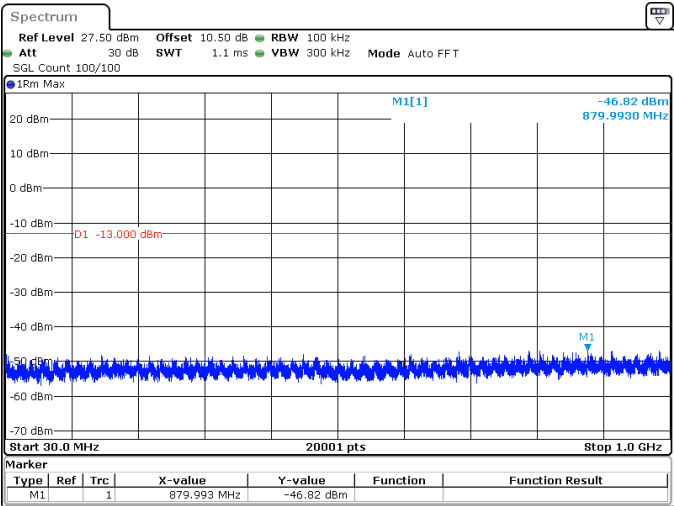
25MHz_15kHz_1722.5MHz_DFT-s-OFDM QPSK_RB128@0 -46.82 dBm
