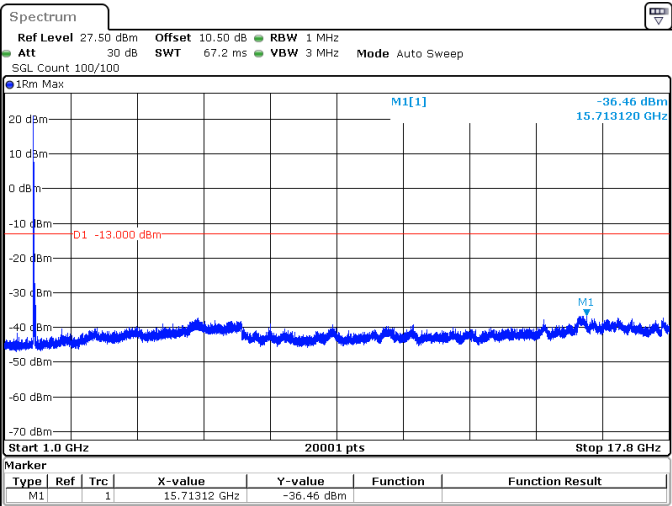
25MHz_15kHz_1745MHz_DFT-s-OFDM QPSK_RB1@0 -36.46 dBm
