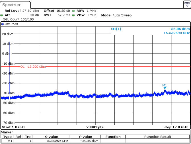
20MHz_15kHz_1745MHz_DFT-s-OFDM QPSK_RB100@0 -36.06 dBm
