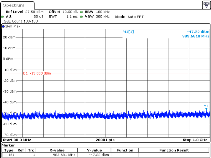
25MHz_15kHz_1722.5MHz_DFT-s-OFDM QPSK_RB1@0 -47.22 dBm
