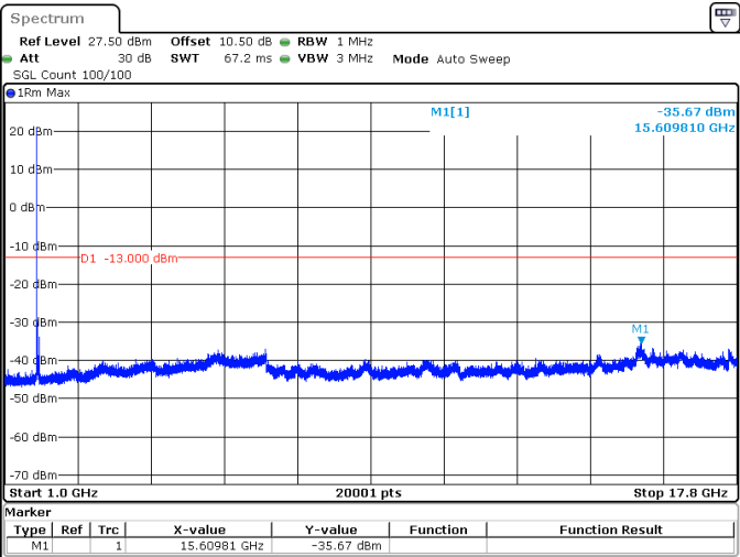
30MHz_15kHz_1745MHz_DFT-s-OFDM QPSK_RB1@0 -35.67 dBm
