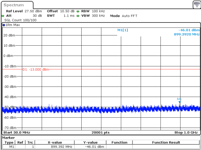
25MHz_15kHz_1767.5MHz_DFT-s-OFDM QPSK_RB128@0 -46.01 dBm
