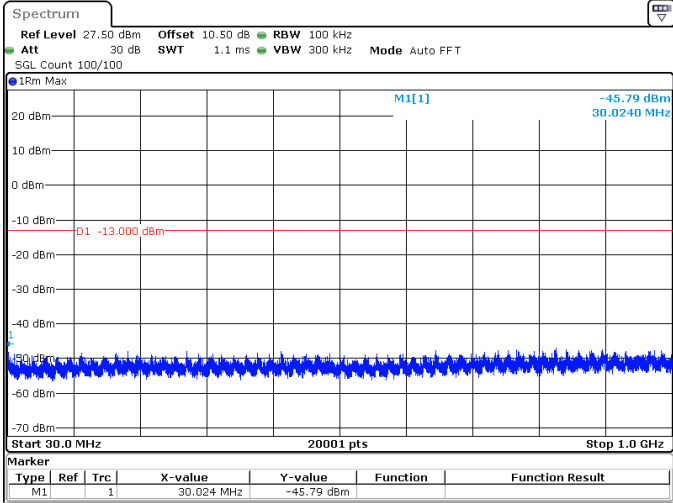
40MHz_15kHz_1760MHz_DFT-s-OFDM QPSK_RB216@0 -45.79 dBm
