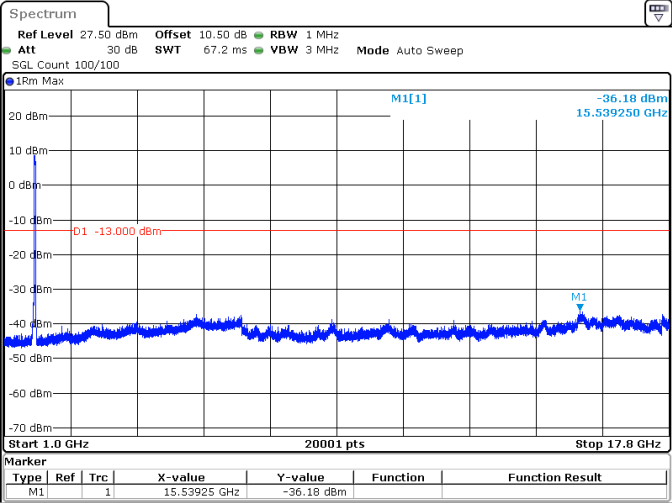
40MHz_15kHz_1760MHz_DFT-s-OFDM QPSK_RB216@0 -36.18 dBm
