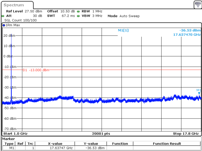
25MHz_15kHz_1767.5MHz_DFT-s-OFDM QPSK_RB1@0 -36.53 dBm
