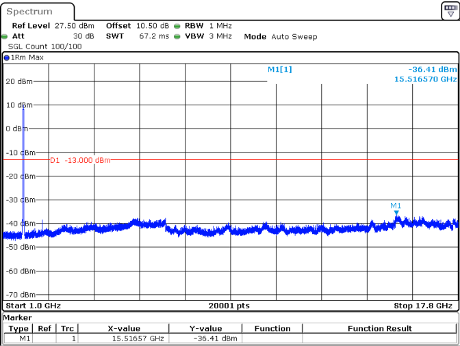
25MHz_15kHz_1745MHz_DFT-s-OFDM QPSK_RB128@0 -36.41 dBm
