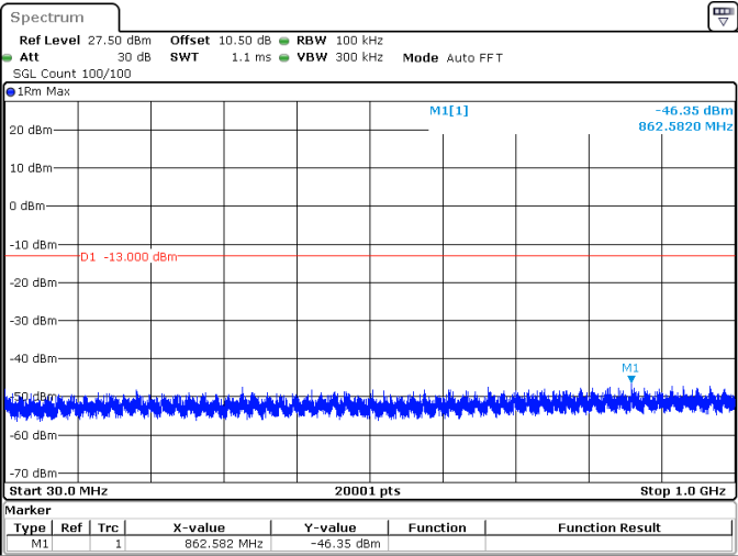
30MHz_15kHz_1725MHz_DFT-s-OFDM QPSK_RB1@159 -46.35 dBm
