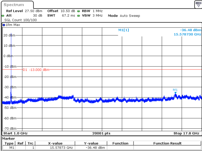
30MHz_15kHz_1725MHz_DFT-s-OFDM QPSK_RB1@159 -36.48 dBm
