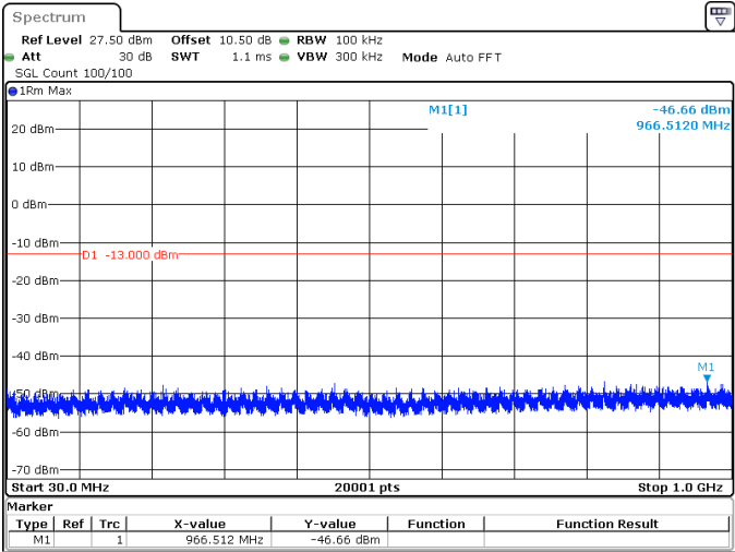
25MHz_15kHz_1767.5MHz_DFT-s-OFDM QPSK_RB1@132 -46.66 dBm
