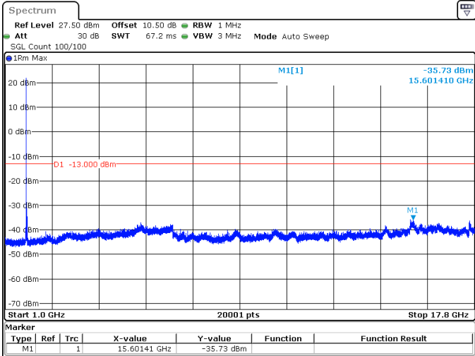
40MHz_15kHz_1760MHz_DFT-s-OFDM QPSK_RB1@0 -35.73 dBm
