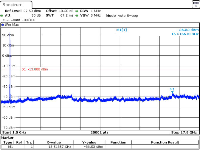
20MHz_15kHz_1745MHz_DFT-s-OFDM QPSK_RB1@105 -36.53 dBm
