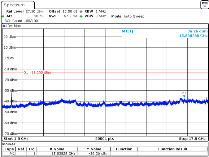
25MHz_15kHz_1767.5MHz_DFT-s-OFDM QPSK_RB1@132 -36.26 dBm
