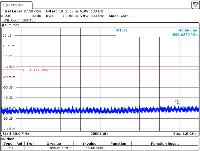
30MHz_15kHz_1745MHz_DFT-s-OFDM QPSK_RB1@0 -46.66 dBm
