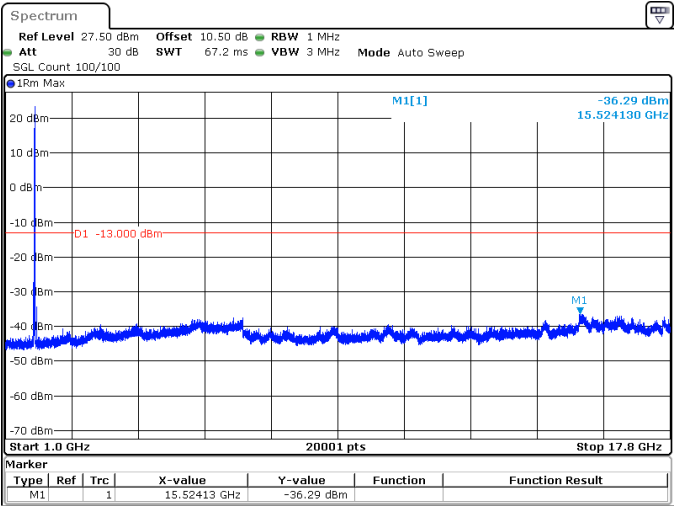
25MHz_15kHz_1722.5MHz_DFT-s-OFDM QPSK_RB1@132 -36.29 dBm
