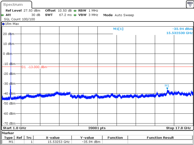
30MHz_15kHz_1765MHz_DFT-s-OFDM QPSK_RB1@159 -35.94 dBm
