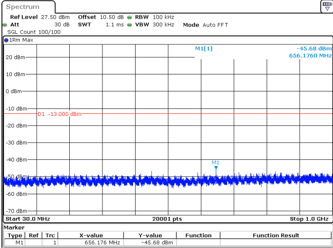
20MHz_15kHz_1720MHz_DFT-s-OFDM QPSK_RB100@0 -45.68 dBm
