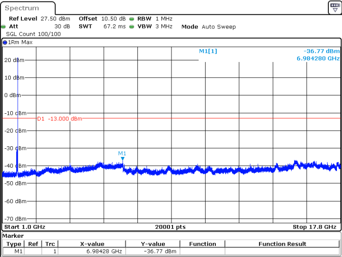
25MHz_15kHz_1745MHz_DFT-s-OFDM QPSK_RB1@132 -36.77 dBm
