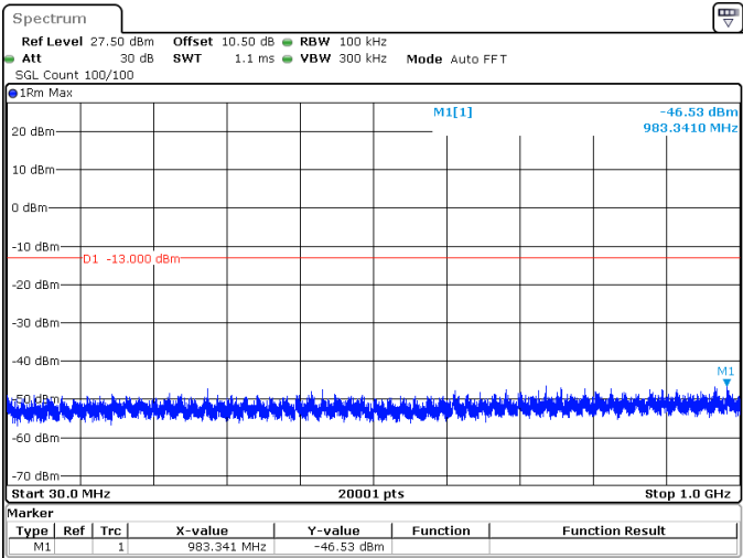
25MHz_15kHz_1767.5MHz_DFT-s-OFDM QPSK_RB1@0 -46.53 dBm
