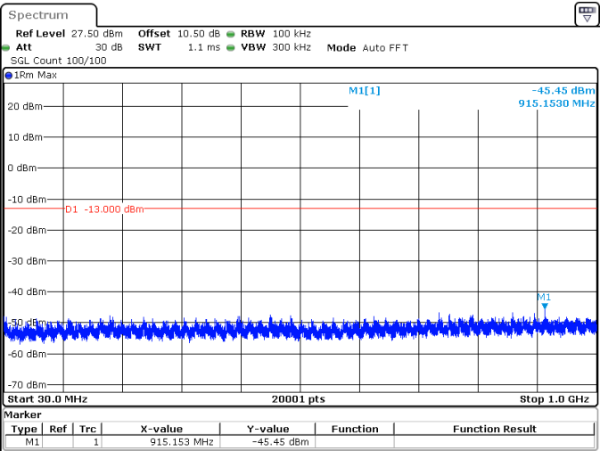
25MHz_15kHz_1745MHz_DFT-s-OFDM QPSK_RB1@0 -45.45 dBm
