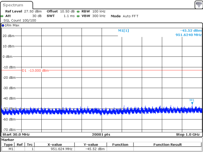
30MHz_15kHz_1725MHz_DFT-s-OFDM QPSK_RB1@0 -45.52 dBm
