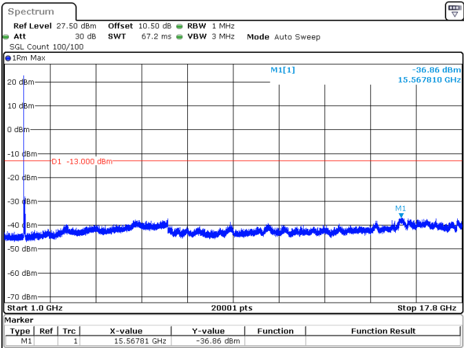
25MHz_15kHz_1722.5MHz_DFT-s-OFDM QPSK_RB1@0 -36.86 dBm
