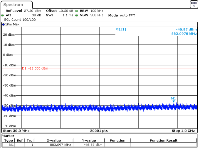
25MHz_15kHz_1722.5MHz_DFT-s-OFDM QPSK_RB1@132 -46.87 dBm
