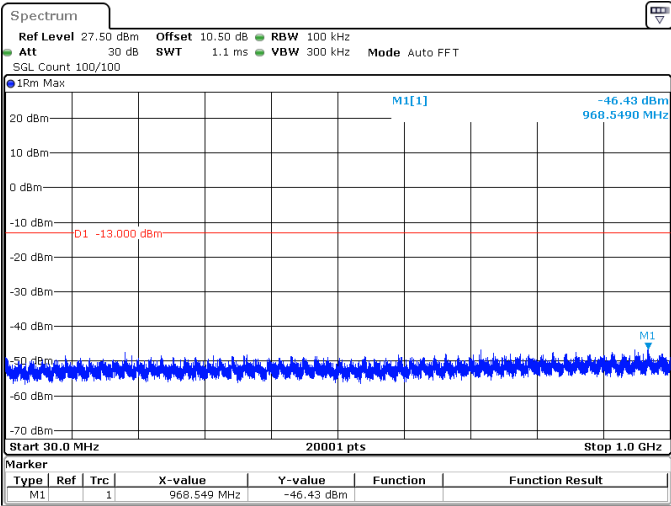
20MHz_15kHz_1745MHz_DFT-s-OFDM QPSK_RB1@105 -46.43 dBm
