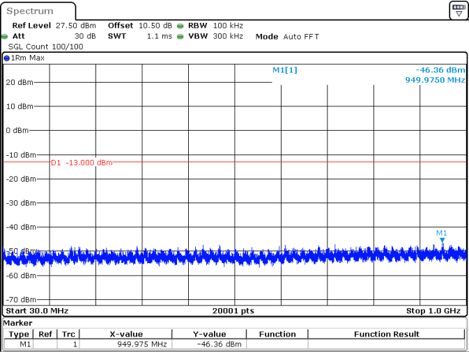
25MHz_15kHz_1745MHz_DFT-s-OFDM QPSK_RB1@132 -46.36 dBm
