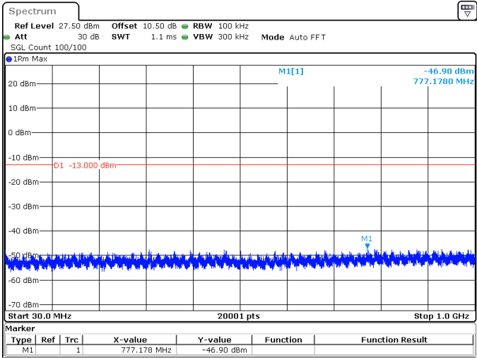
30MHz_15kHz_1765MHz_DFT-s-OFDM QPSK_RB1@159 -46.90 dBm
