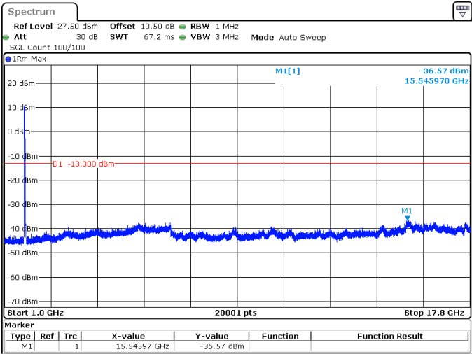
25MHz_15kHz_1722.5MHz_DFT-s-OFDM QPSK_RB128@0 -36.57 dBm
