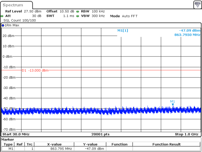
30MHz_15kHz_1745MHz_DFT-s-OFDM QPSK_RB160@0 -47.09 dBm
