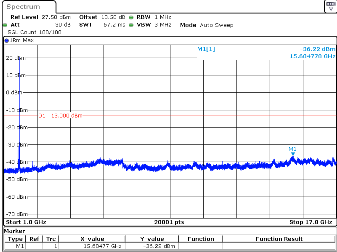
40MHz_15kHz_1760MHz_DFT-s-OFDM QPSK_RB1@215 -36.22 dBm
