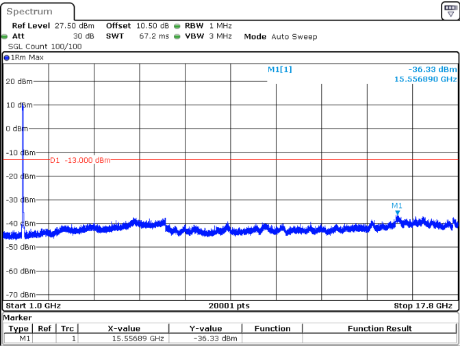
30MHz_15kHz_1725MHz_DFT-s-OFDM QPSK_RB160@0 -36.33 dBm
