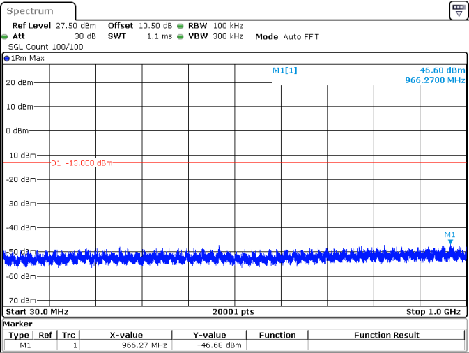
30MHz_15kHz_1745MHz_DFT-s-OFDM QPSK_RB1@159 -46.68 dBm
