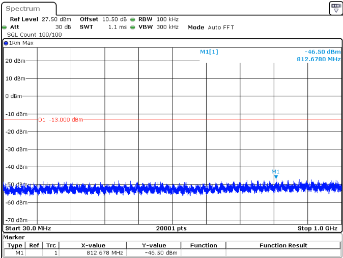
30MHz_15kHz_1765MHz_DFT-s-OFDM QPSK_RB1@0 -46.50 dBm
