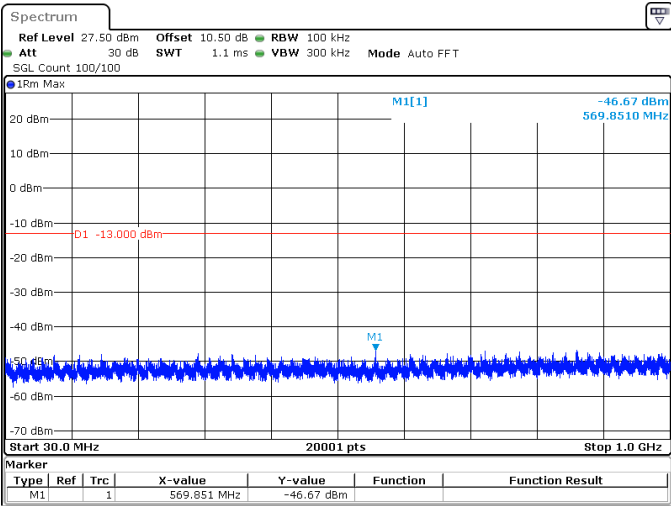
20MHz_15kHz_1745MHz_DFT-s-OFDM QPSK_RB100@0 -46.67 dBm
