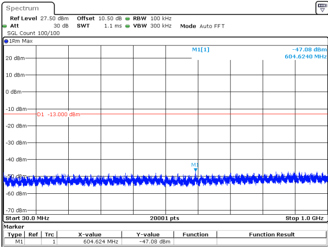
30MHz_15kHz_1725MHz_DFT-s-OFDM QPSK_RB160@0 -47.08 dBm
