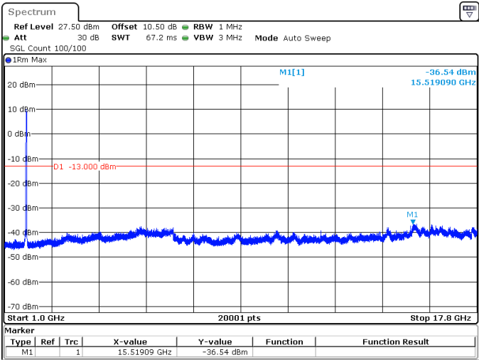
25MHz_15kHz_1767.5MHz_DFT-s-OFDM QPSK_RB128@0 -36.54 dBm
