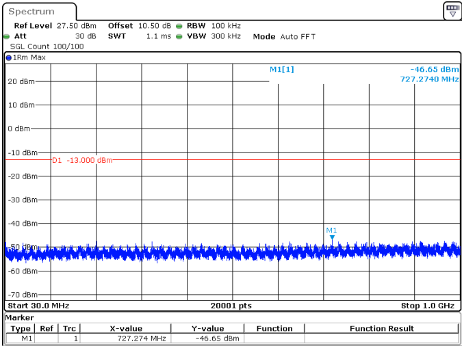
30MHz_15kHz_1765MHz_DFT-s-OFDM QPSK_RB160@0 -46.65 dBm
