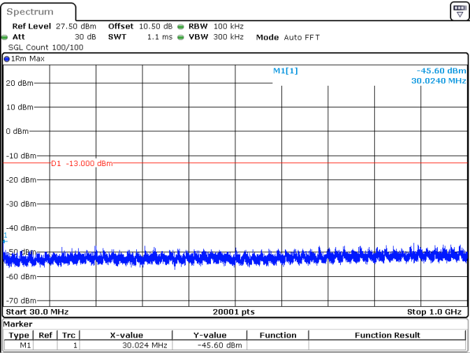
25MHz_15kHz_1745MHz_DFT-s-OFDM QPSK_RB128@0 -45.60 dBm
