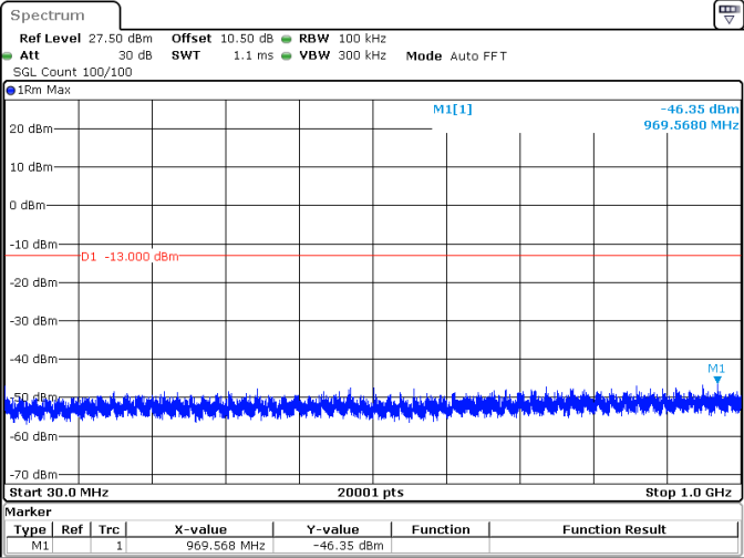
40MHz_15kHz_1760MHz_DFT-s-OFDM QPSK_RB1@215 -46.35 dBm
