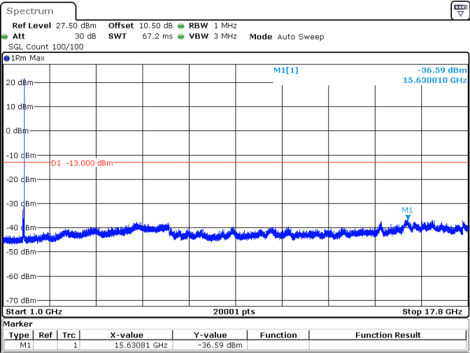
30MHz_15kHz_1745MHz_DFT-s-OFDM QPSK_RB1@159 -36.59 dBm
