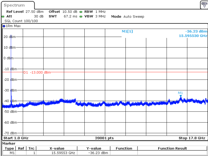
30MHz_15kHz_1725MHz_DFT-s-OFDM QPSK_RB1@0 -36.23 dBm
