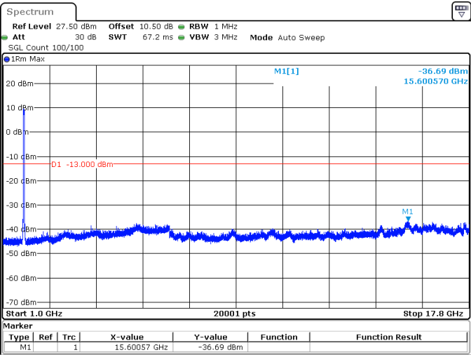
30MHz_15kHz_1745MHz_DFT-s-OFDM QPSK_RB160@0 -36.69 dBm
