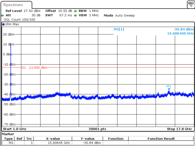
30MHz_15kHz_1765MHz_DFT-s-OFDM QPSK_RB160@0 -35.84 dBm
