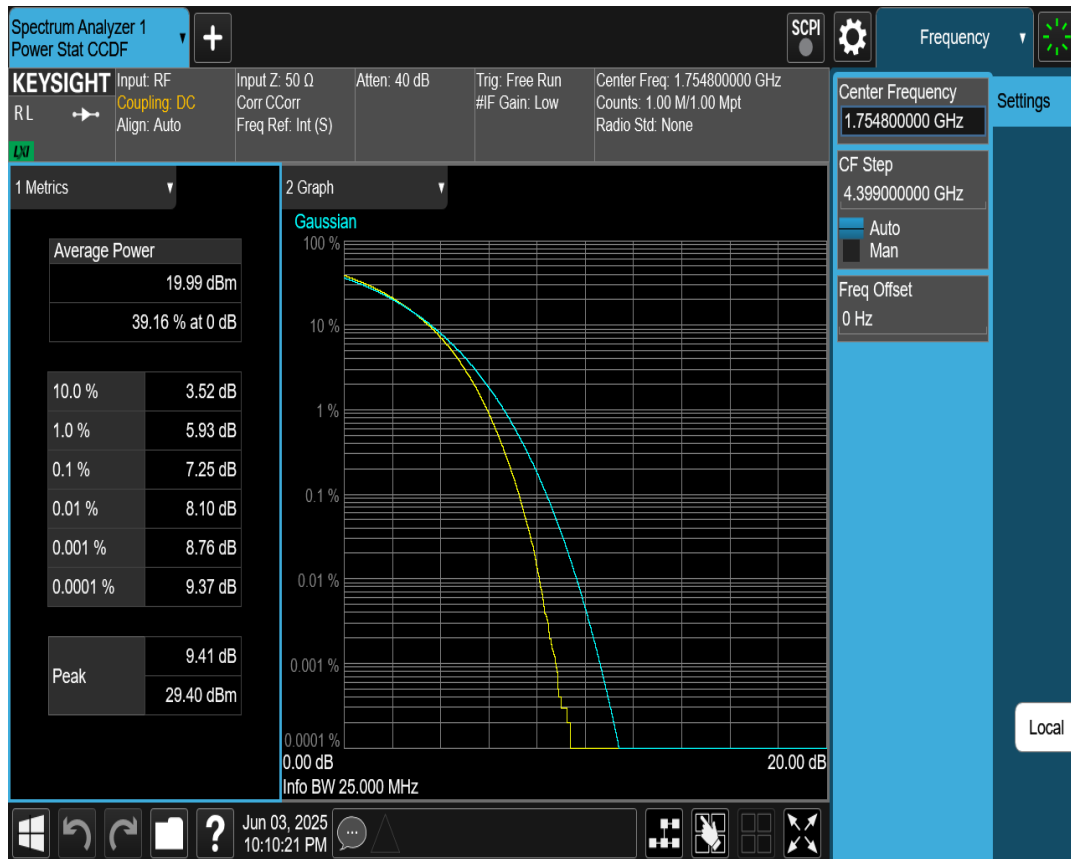
66C 16QAM PCC BW=20MHz Ch=66812 RB=100@0, SCC BW=15MHz Ch=66983 RB=75@0
