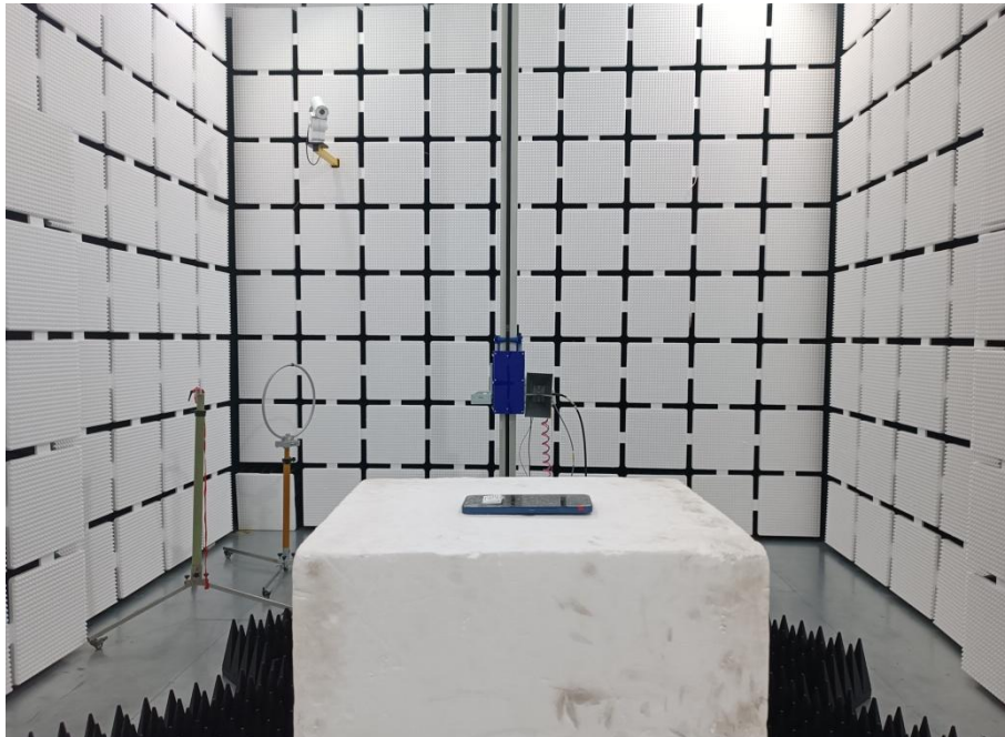
RADIATED EMISSION TEST ABOVE 1GHz
