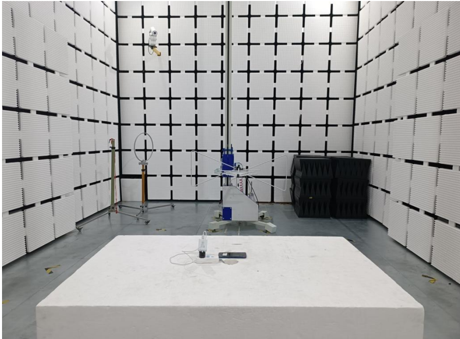
RADIATED EMISSION TEST BELOW 1GHz
