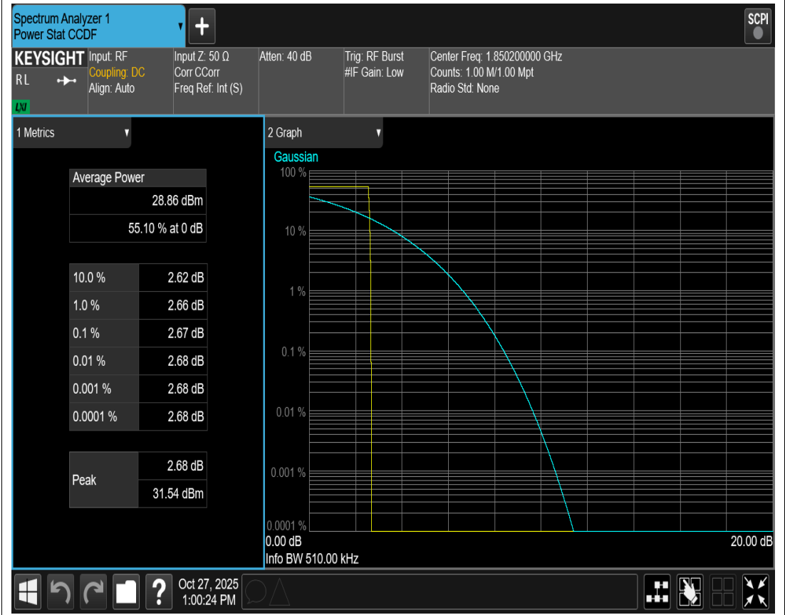
GSM1900 Channel=512
