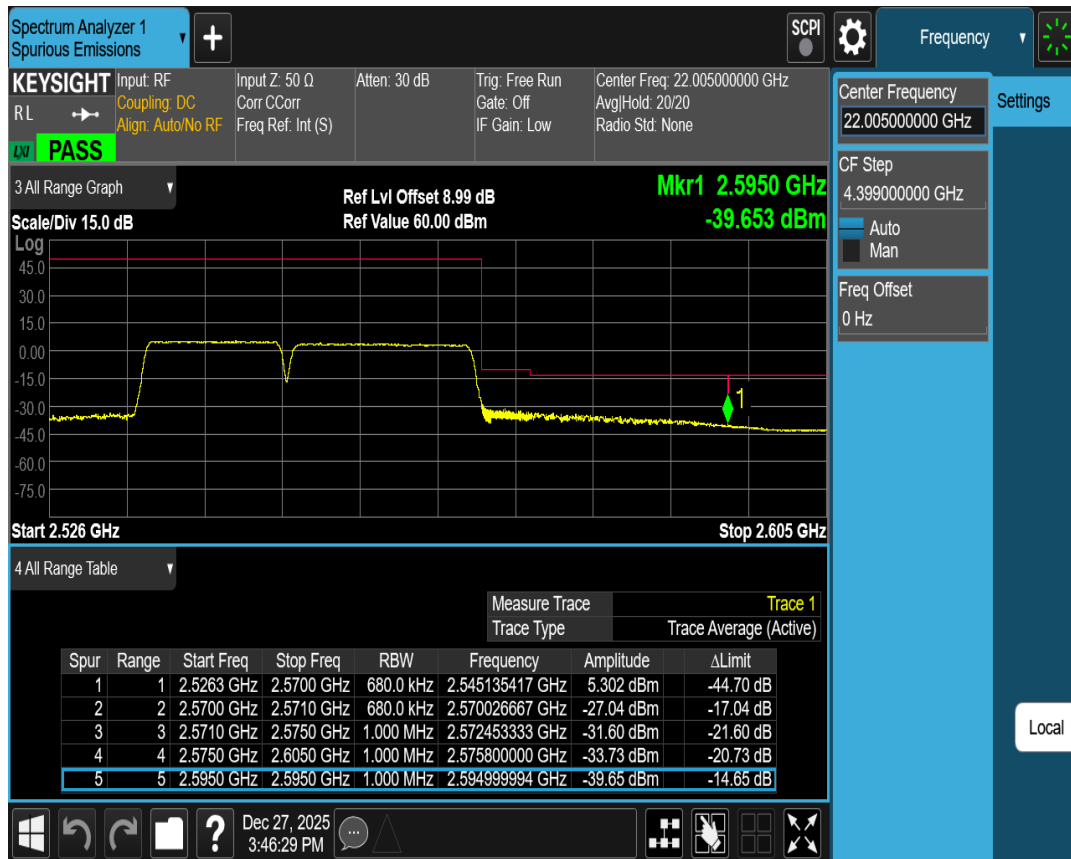
7C 16QAM PCC BW=15MHz Ch=3225 RB=1@0,SCC BW=15MHz Ch=3375 RB=1@74
