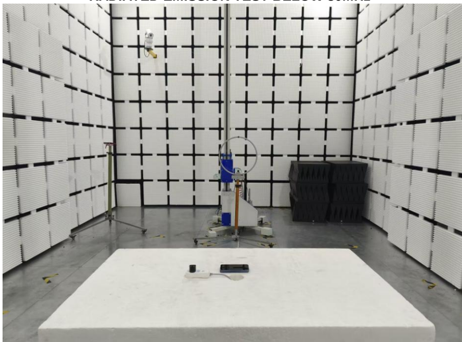
RADIATED EMISSION TEST BELOW 30MHz
