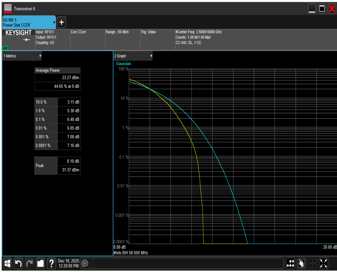
n77(3450-3550) SCS=30kHz DFT_QAM64 BW=60MHz Channel=634666 RB=162@0
