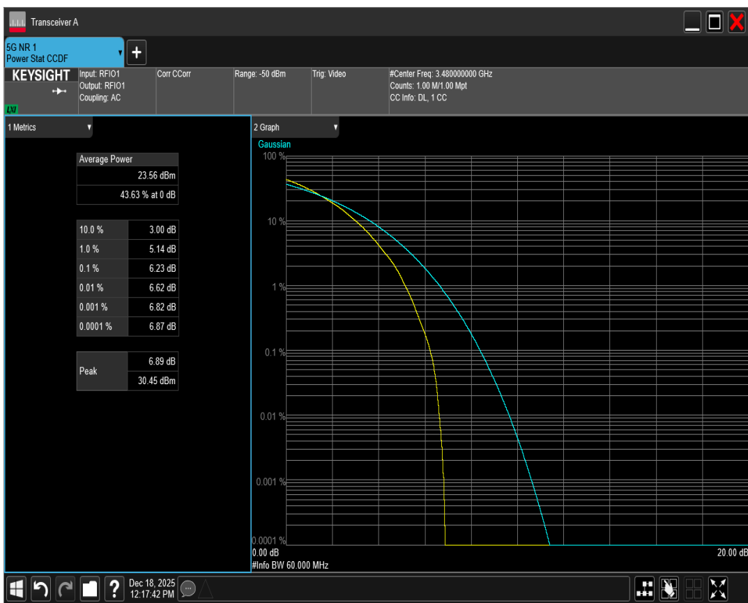
n77(3450-3550) SCS=30kHz DFT_QAM64 BW=60MHz Channel=633334 RB=162@0
