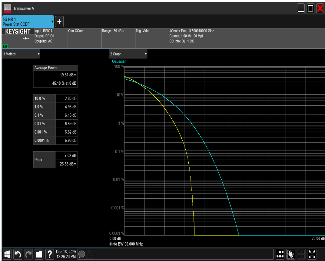
n77(3450-3550) SCS=30kHz DFT_QAM64 BW=90MHz Channel=633666 RB=240@0
