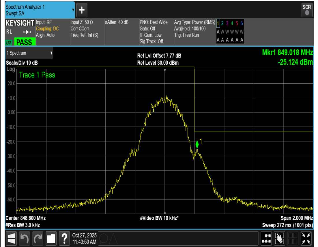
GSM850 Channel=251
