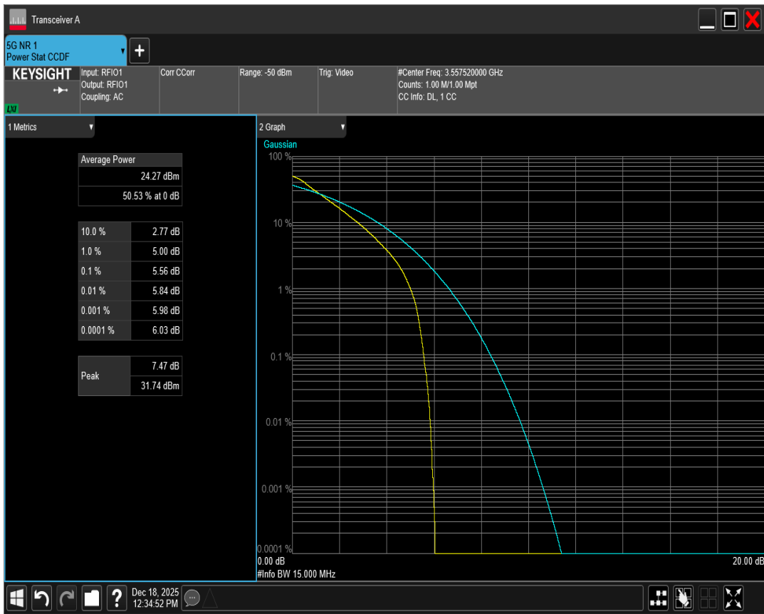
n77(3550-3700) SCS=30kHz DFT_QPSK BW=15MHz Channel=641666 RB=36@0
