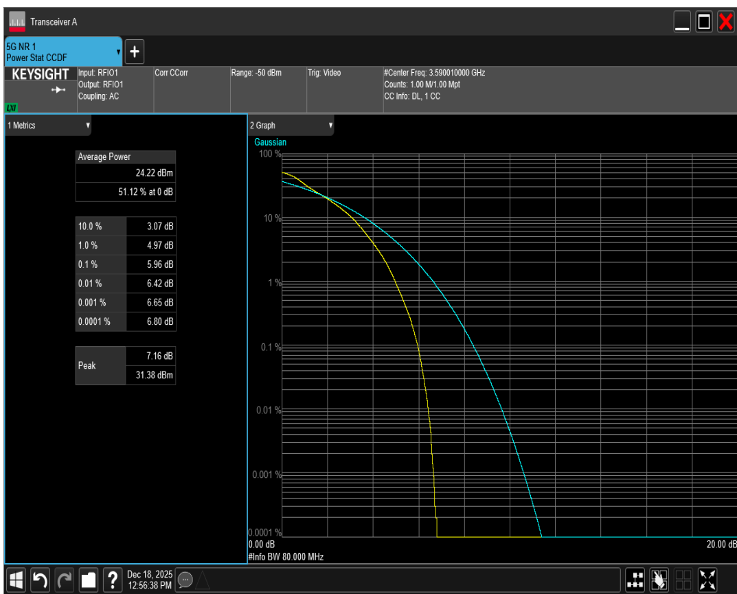
n77(3550-3700) SCS=30kHz DFT_QPSK BW=80MHz Channel=641666 RB=216@0
