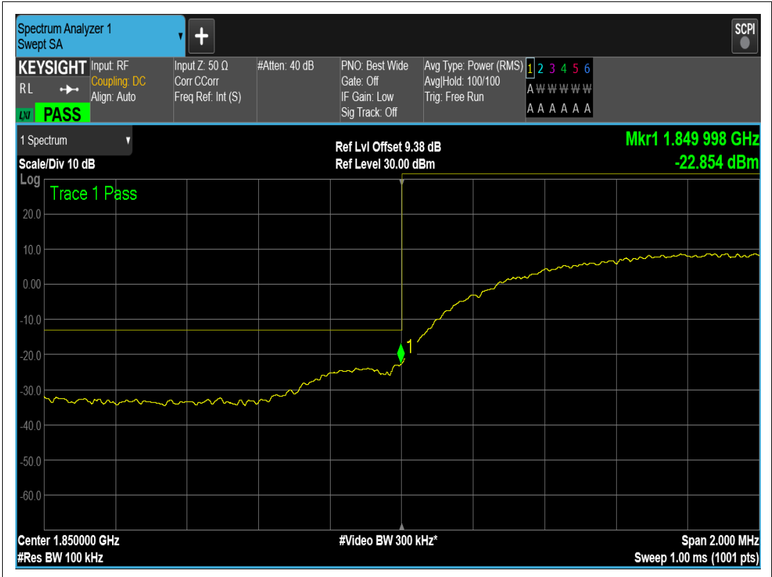
WCDMA Band2 Channel=9262
