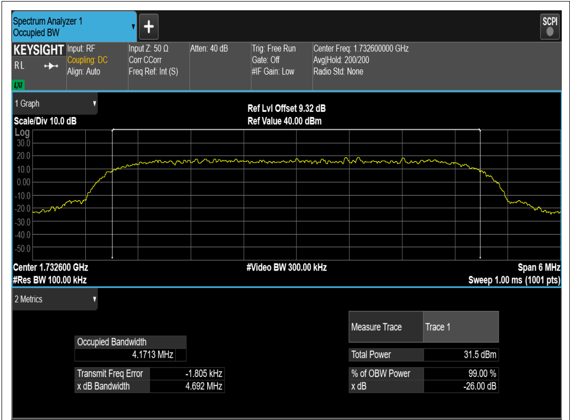
WCDMA Band4 Channel=1413
