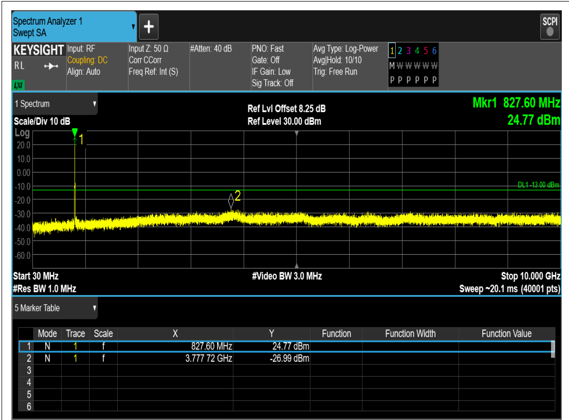
WCDMA Band5 Channel=4132
