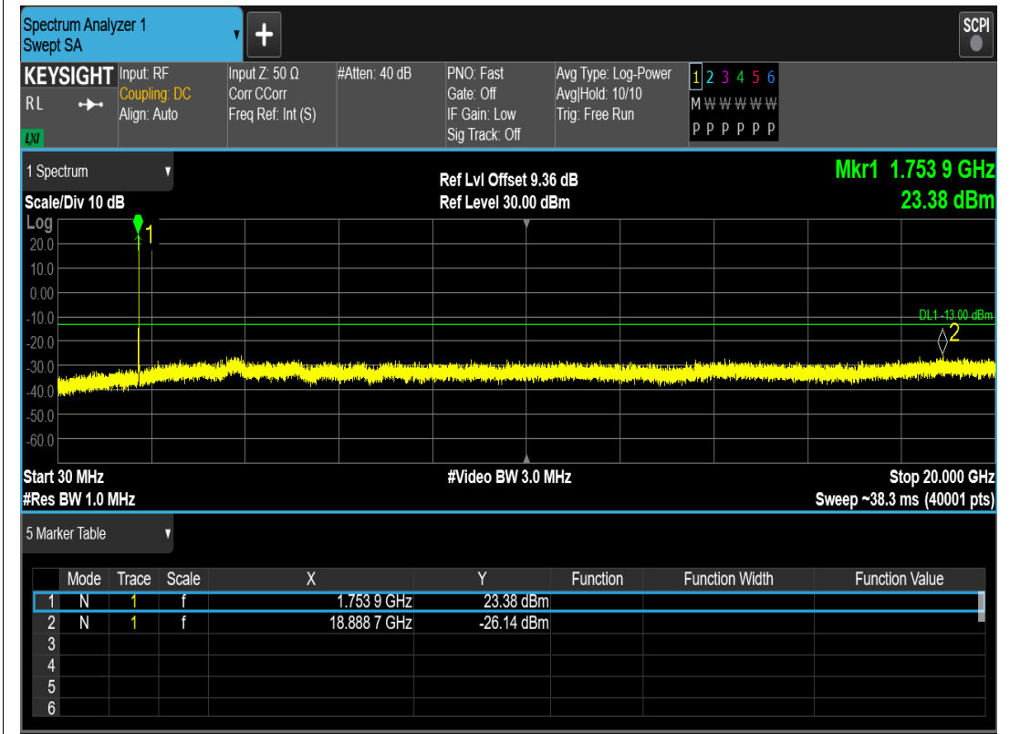
WCDMA Band4 Channel=1513
