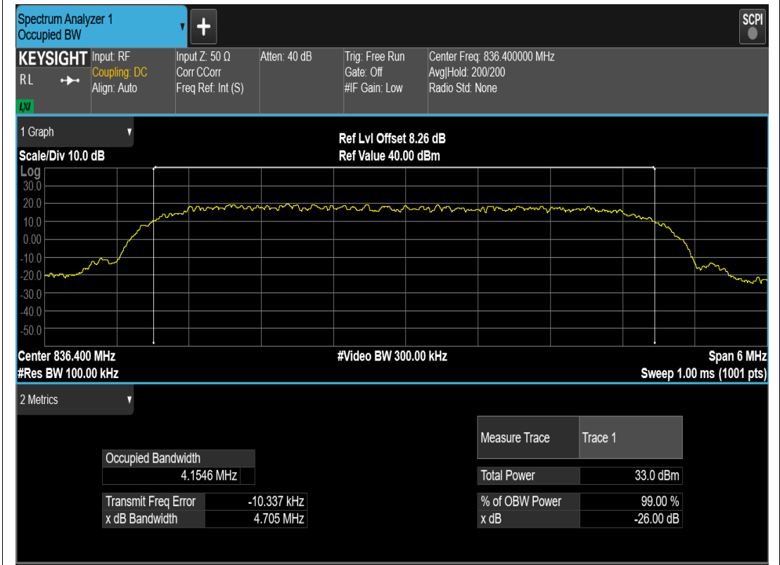
WCDMA Band5 Channel=4182
