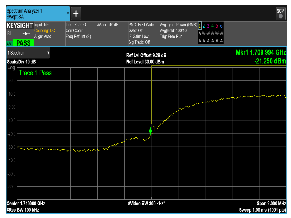
WCDMA Band4 Channel=1312
