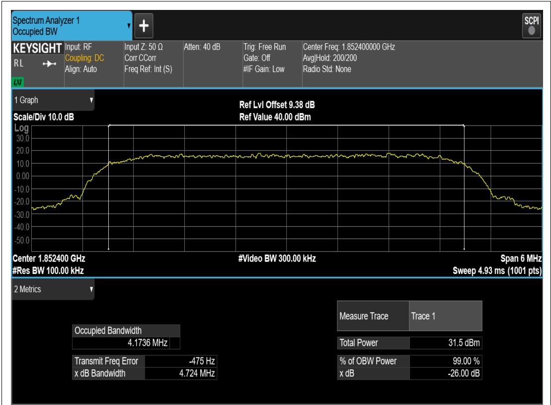
WCDMA Band2 Channel=9262
