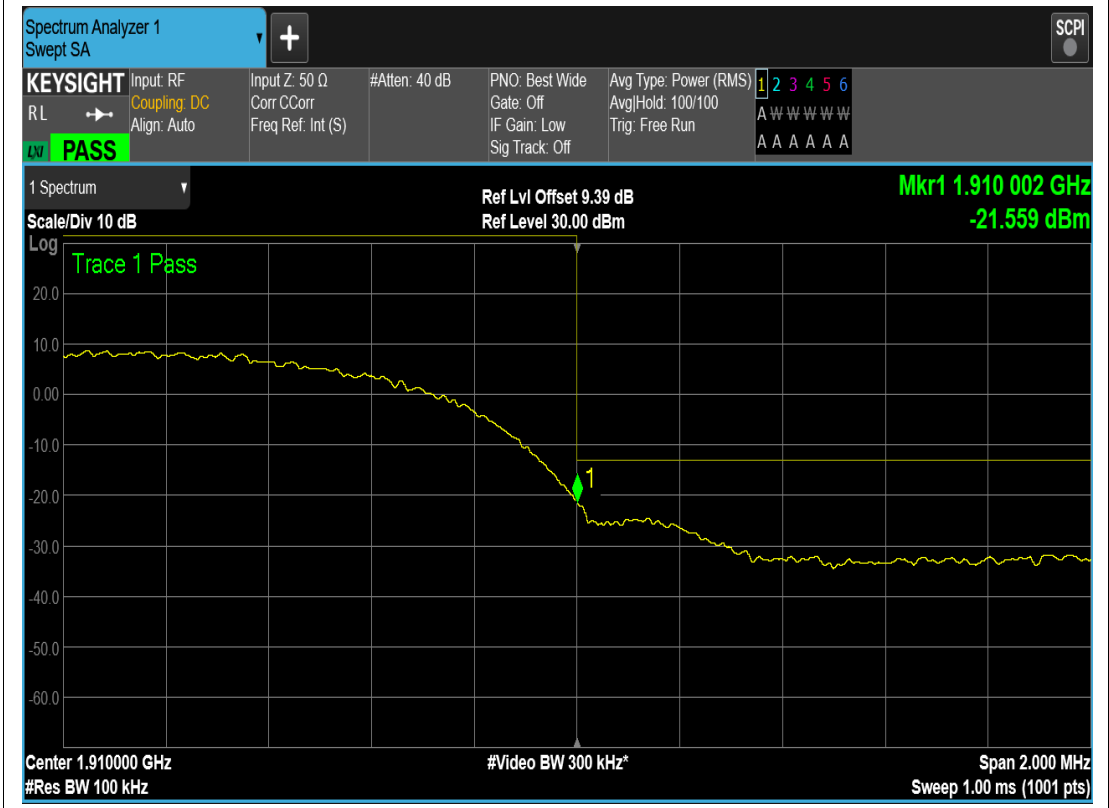
WCDMA Band2 Channel=9538
