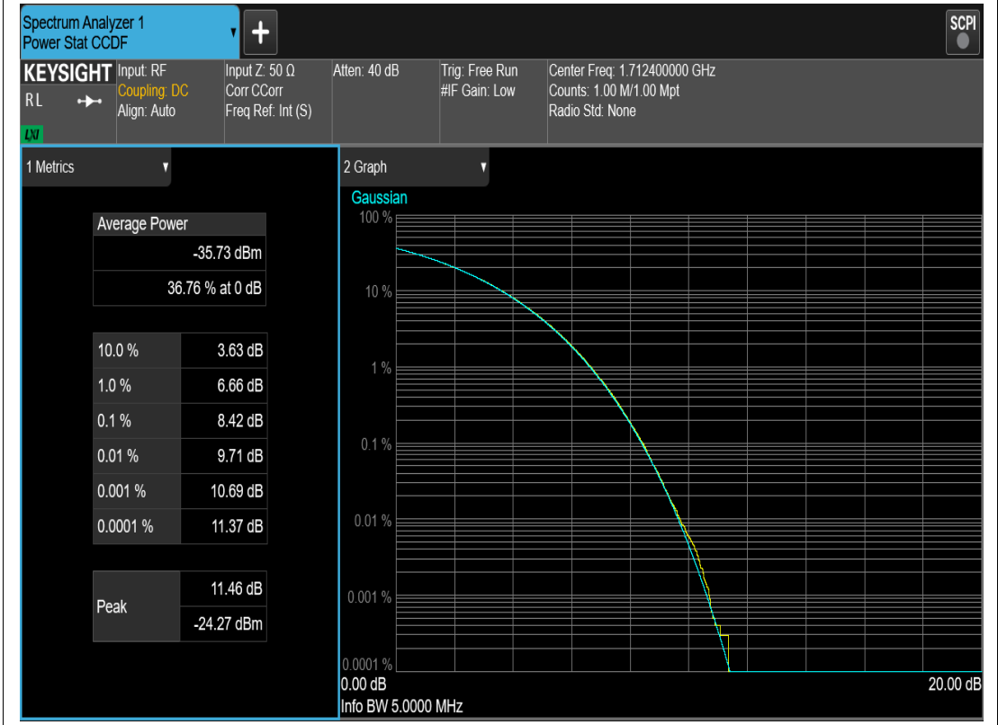
WCDMA Band4 Channel=1312
