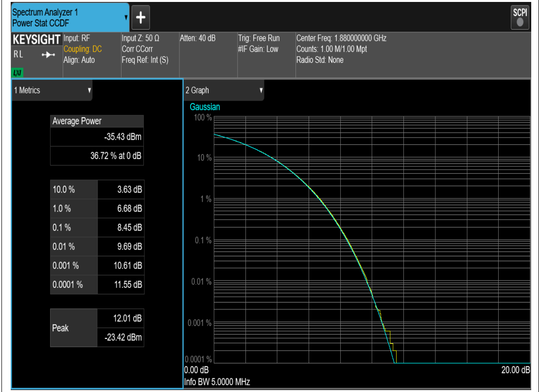
WCDMA Band2 Channel=9400
