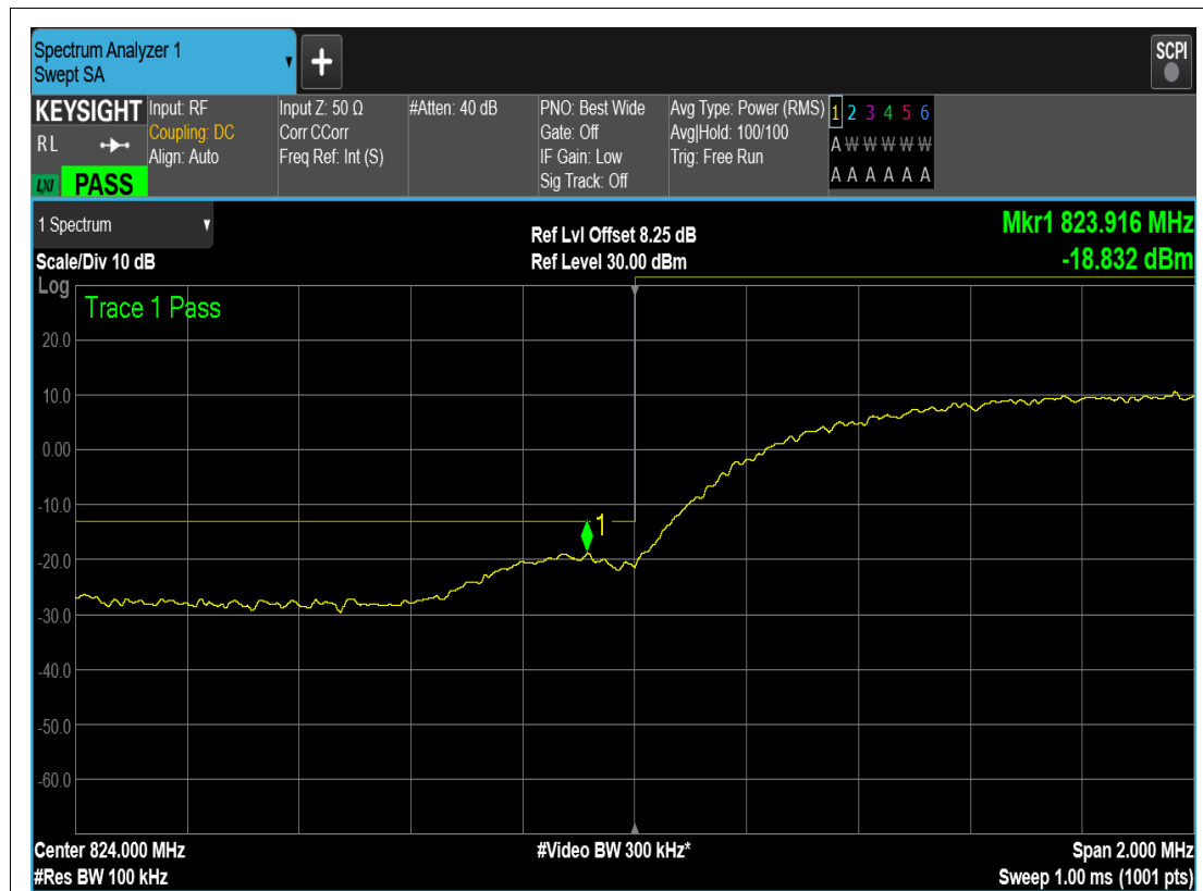
WCDMA Band5 Channel=4132
