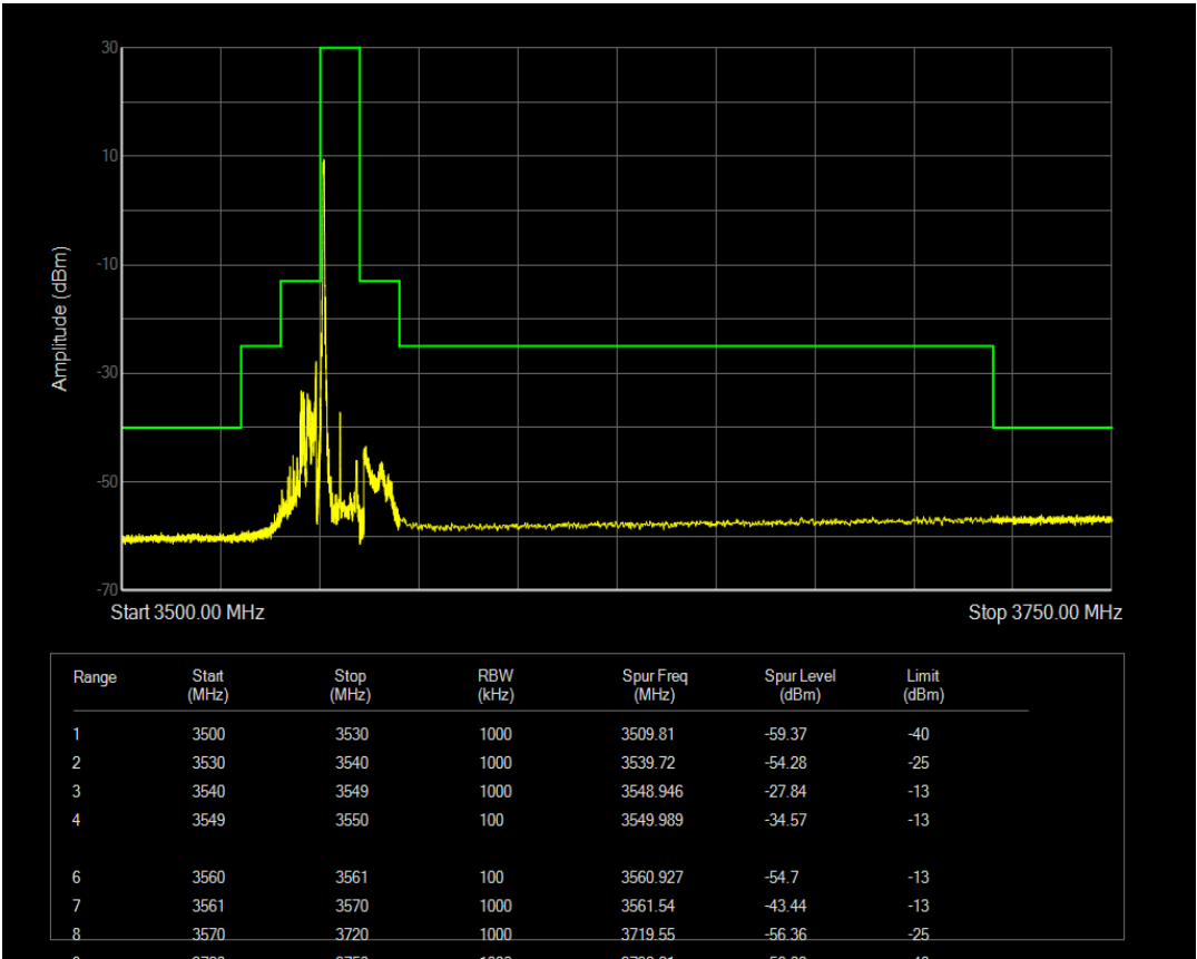
n77(3550-3700) SCS=30kHz CP_QPSK BW=10MHz Channel=637000 RB=1@23
