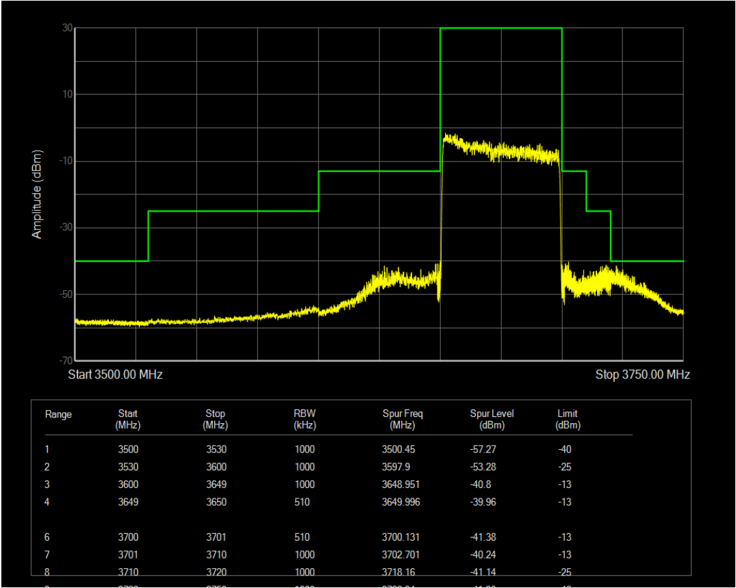
n77(3550-3700) SCS=30kHz CP_QPSK BW=50MHz Channel=645000 RB=1@0
