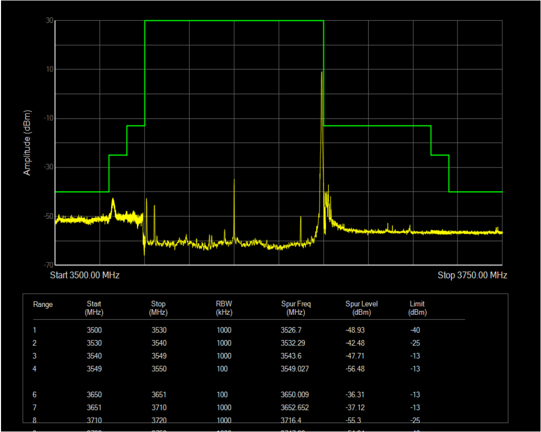
n77(3550-3700) SCS=30kHz CP_QPSK BW=100MHz Channel=640000 RB=273@0
