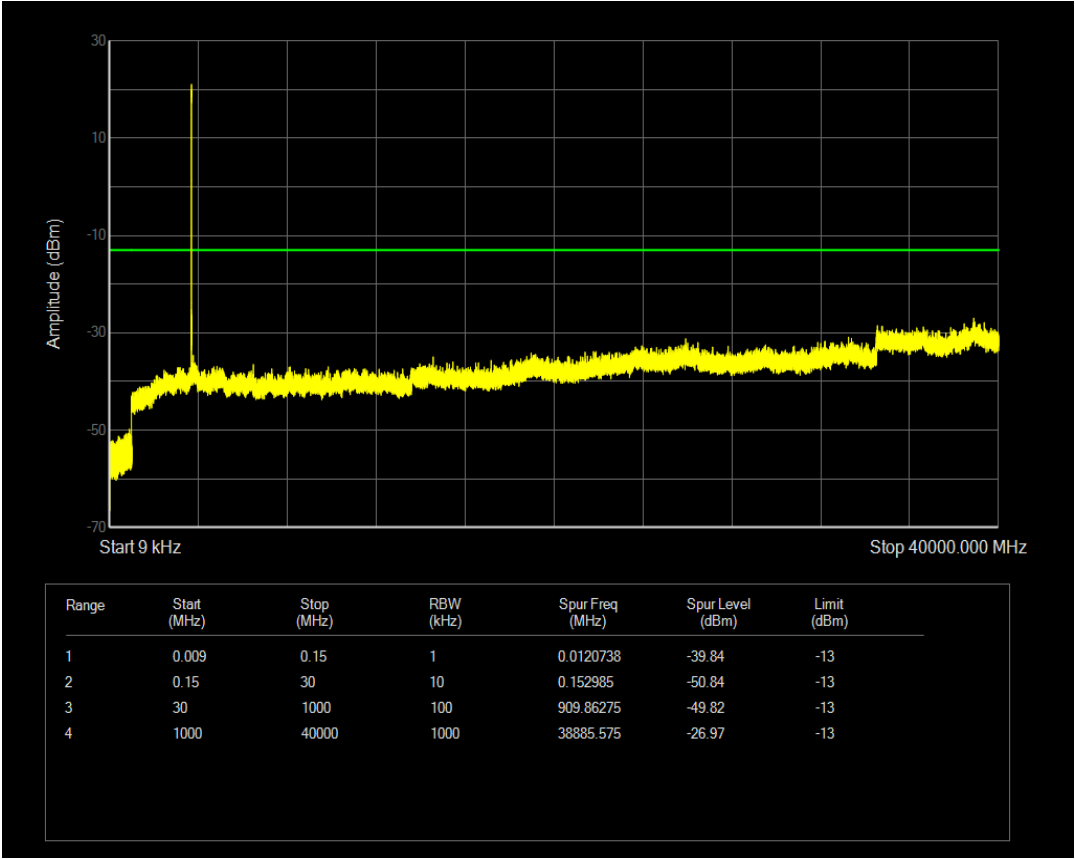
n77(3550-3700) SCS=30kHz CP_QPSK BW=50MHz Channel=638334 RB=133@0
