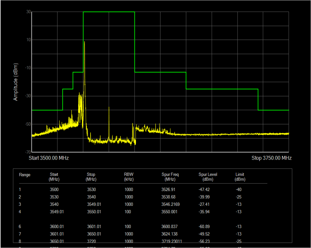
n77(3550-3700) SCS=30kHz CP_QPSK BW=50MHz Channel=638334 RB=1@132
