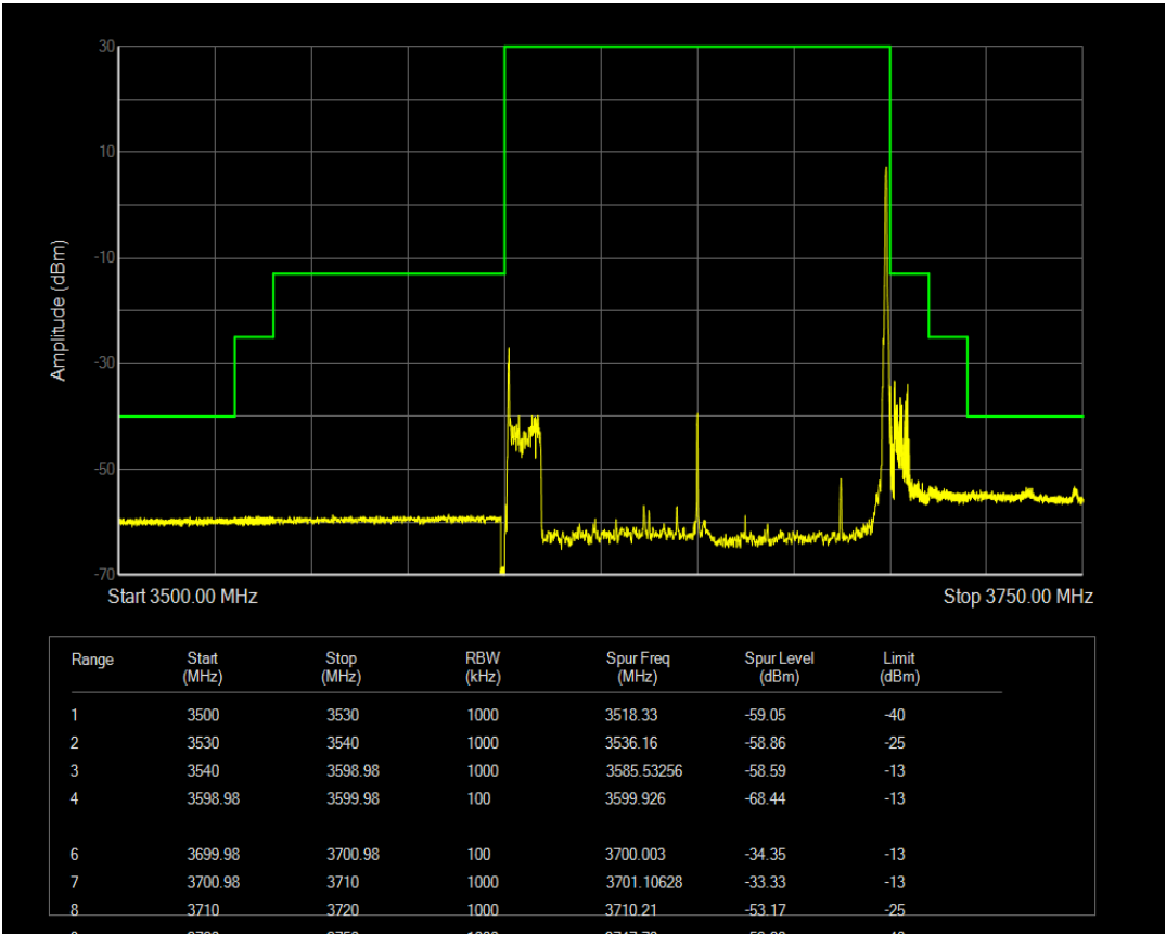
n77(3550-3700) SCS=30kHz CP_QPSK BW=100MHz Channel=643332 RB=273@0
