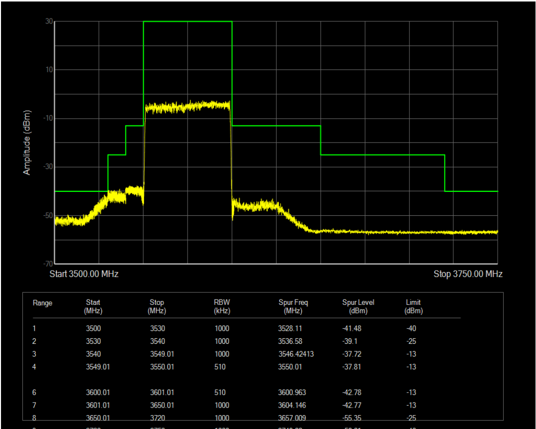
n77(3550-3700) SCS=30kHz CP_QPSK BW=50MHz Channel=638334 RB=1@0
