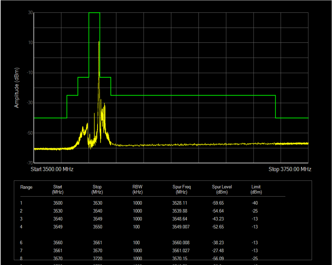
n77(3550-3700) SCS=30kHz CP_QPSK BW=10MHz Channel=637000 RB=24@0
