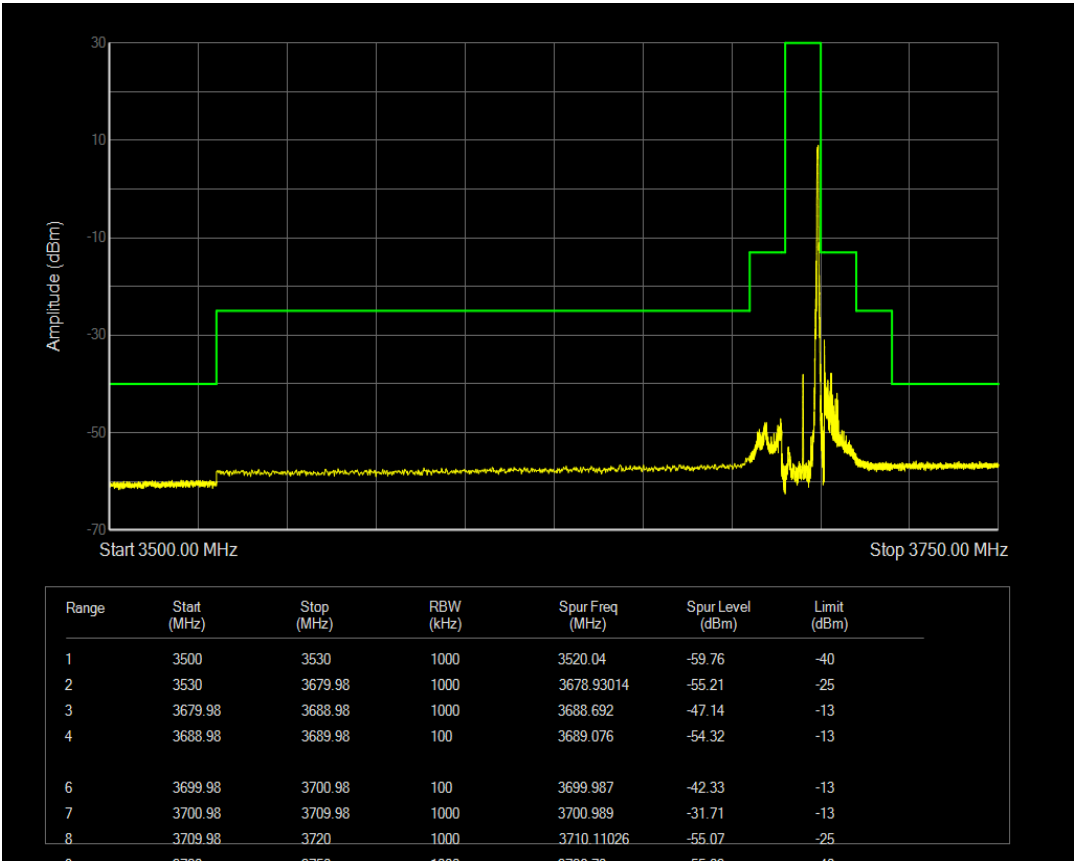
n77(3550-3700) SCS=30kHz CP_QPSK BW=10MHz Channel=646332 RB=24@0
