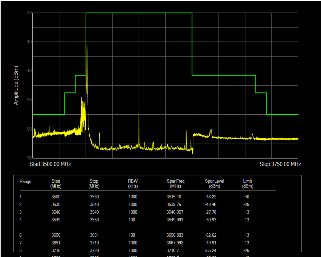
n77(3550-3700) SCS=30kHz CP_QPSK BW=100MHz Channel=640000 RB=1@272
