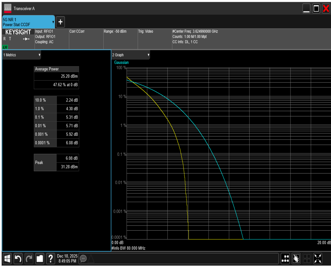
n78(3550-3700) SCS=30kHz DFT_QPSK BW=80MHz Channel=644000 RB=216@0
