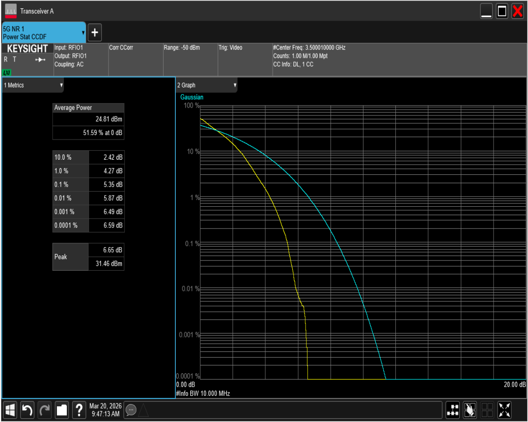
n77(3450-3550) SCS=30kHz DFT_QPSK BW=10MHz Channel=633332 RB=24@0
