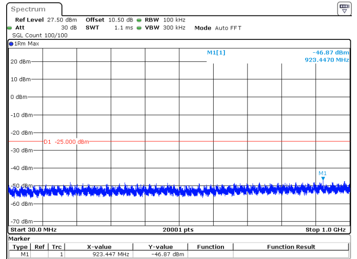
15MHz_30kHz_2612.5MHz_DFT-s-OFDM QPSK_RB1@37 -46.87 dBm
