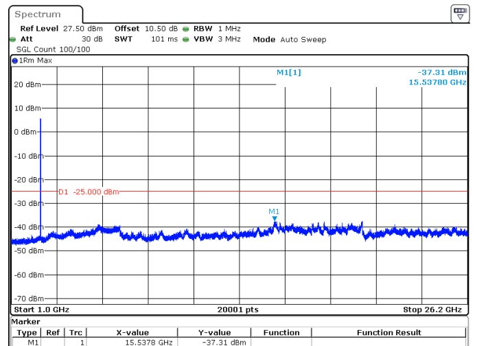
15MHz_30kHz_2612.5MHz_DFT-s-OFDM QPSK_RB36@0 -37.31 dBm
