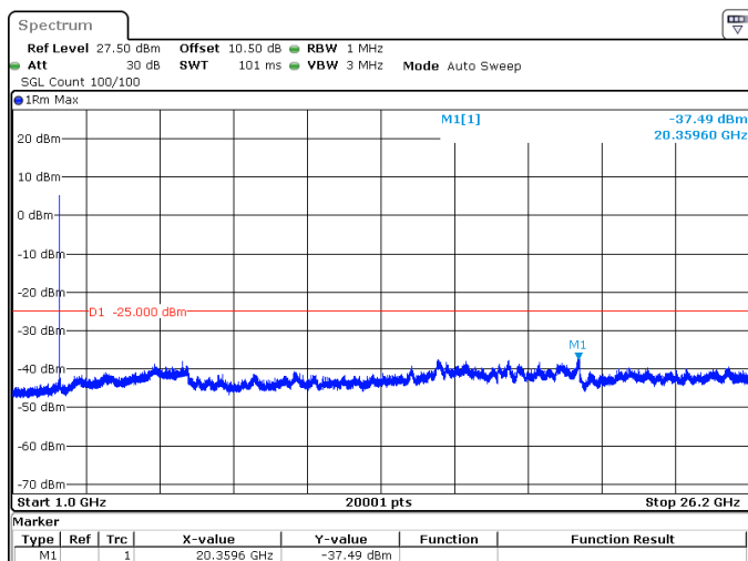
15MHz_30kHz_2595MHz_DFT-s-OFDM QPSK_RB36@0 -37.49 dBm
