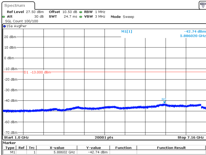
15MHz_15kHz_706.5MHz_DFT-s-OFDM QPSK_RB1@78 -42.74 dBm
