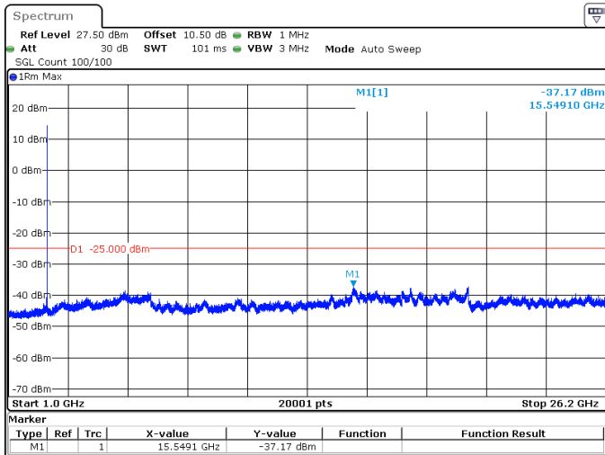
15MHz_30kHz_2612.5MHz_DFT-s-OFDM QPSK_RB1@37 -37.17 dBm
