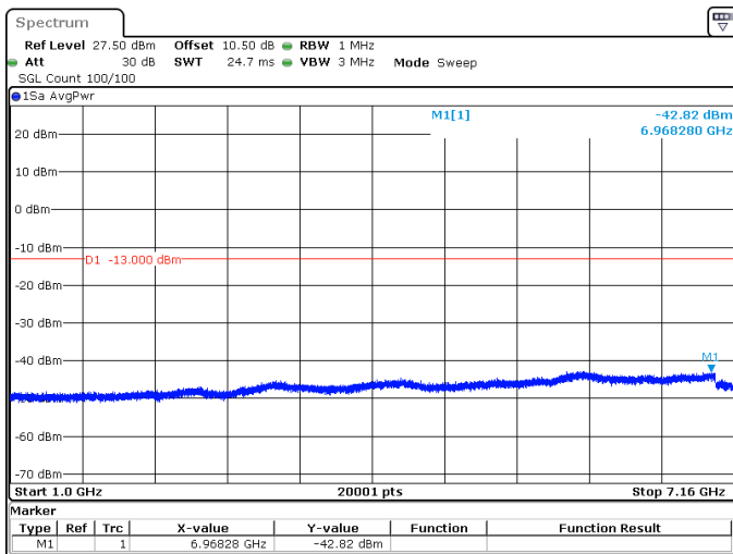
5MHz_15kHz_707.5MHz_DFT-s-OFDM QPSK_RB1@24 -42.82 dBm
