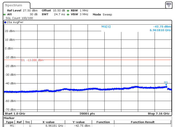
15MHz_15kHz_708.5MHz_DFT-s-OFDM QPSK_RB75@0 -42.75 dBm
