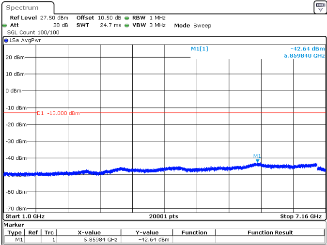
5MHz_15kHz_713.5MHz_DFT-s-OFDM QPSK_RB1@24 -42.64 dBm
