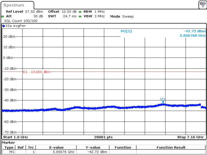
5MHz_15kHz_713.5MHz_DFT-s-OFDM QPSK_RB1@0 -42.72 dBm
