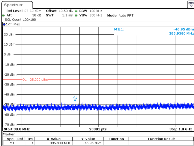
15MHz_30kHz_2612.5MHz_DFT-s-OFDM QPSK_RB1@0 -46.95 dBm
