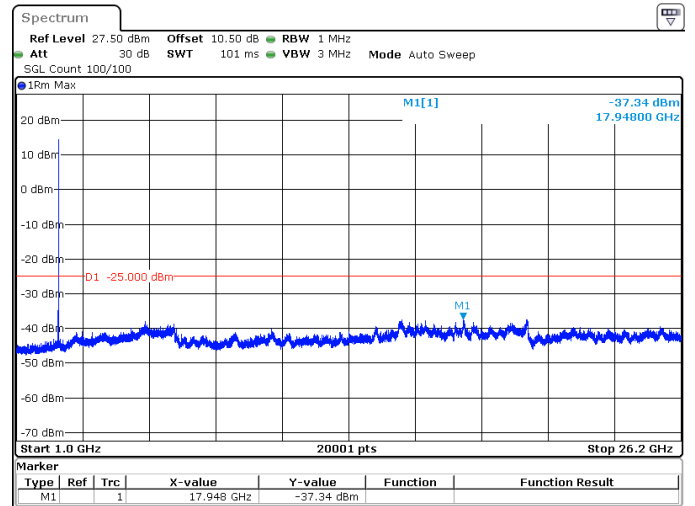
15MHz_30kHz_2577.5MHz_DFT-s-OFDM QPSK_RB1@37 -37.34 dBm
