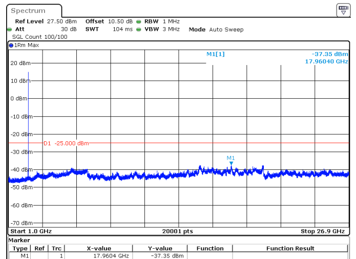
10MHz_30kHz_2501.01MHz_DFT-s-OFDM QPSK_RB1@23 -37.35 dBm
