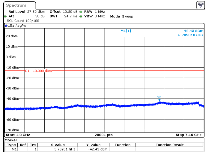
15MHz_15kHz_708.5MHz_DFT-s-OFDM QPSK_RB1@78 -42.43 dBm
