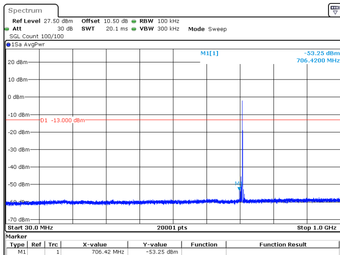
10MHz_15kHz_711MHz_DFT-s-OFDM QPSK_RB1@51 -53.25 dBm
