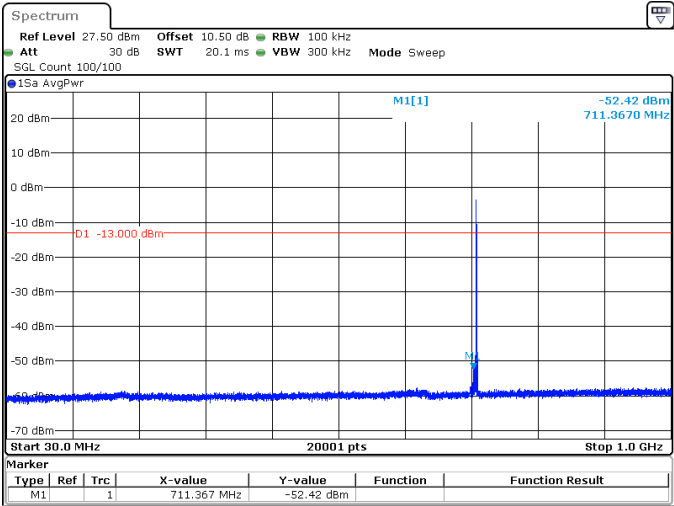
5MHz_15kHz_713.5MHz_DFT-s-OFDM QPSK_RB1@24 -52.42 dBm
