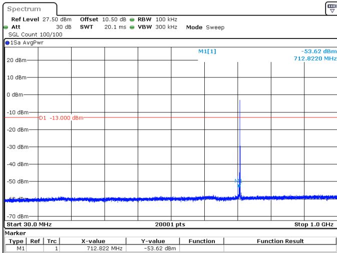
15MHz_15kHz_708.5MHz_DFT-s-OFDM QPSK_RB1@78 -53.62 dBm
