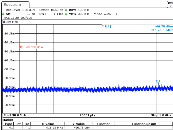
15MHz_30kHz_2577.5MHz_DFT-s-OFDM QPSK_RB1@37 -66.78 dBm
