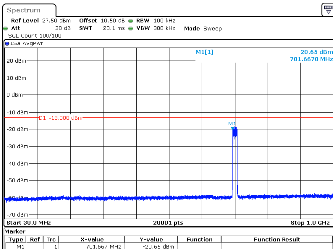
15MHz_15kHz_708.5MHz_DFT-s-OFDM QPSK_RB75@0 -20.65 dBm
