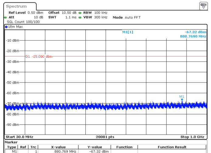
40MHz_30kHz_2600MHz_DFT-s-OFDM QPSK_RB100@0 -67.32 dBm
