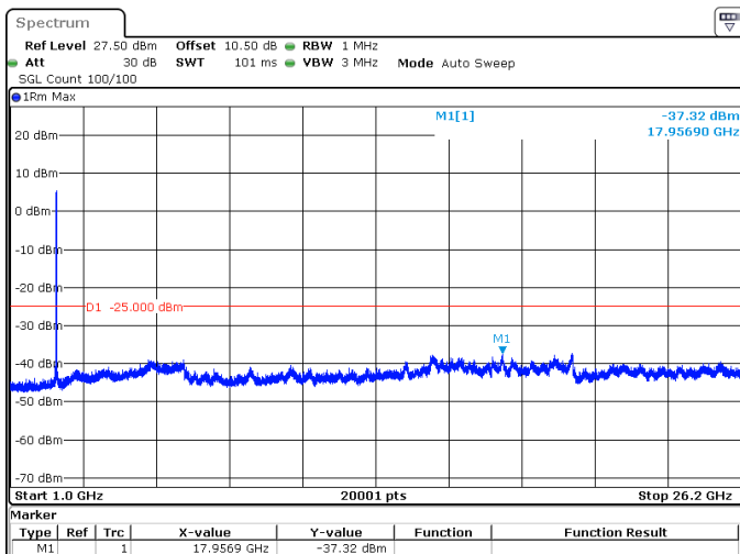
25MHz_30kHz_2582.5MHz_DFT-s-OFDM QPSK_RB64@0 -37.32 dBm
