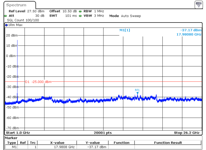
5MHz_15kHz_2595MHz_DFT-s-OFDM QPSK_RB1@0 -37.17 dBm
