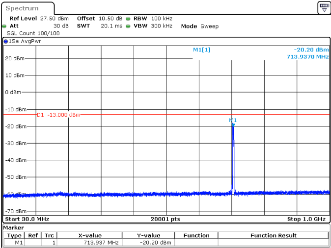
5MHz_15kHz_713.5MHz_DFT-s-OFDM QPSK_RB25@0 -20.20 dBm
