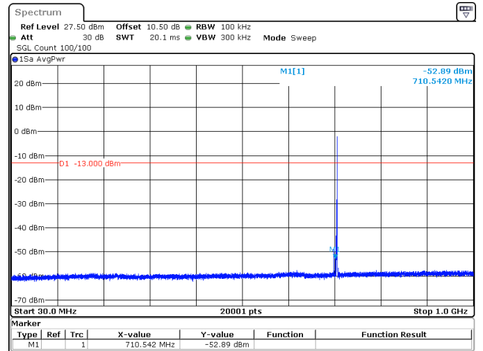
15MHz_15kHz_706.5MHz_DFT-s-OFDM QPSK_RB1@78 -52.89 dBm
