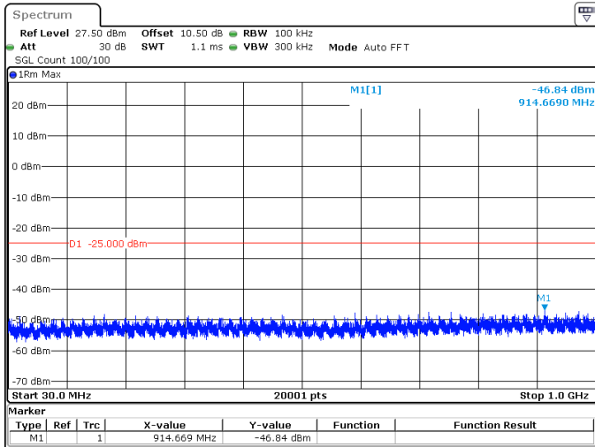
15MHz_30kHz_2577.5MHz_DFT-s-OFDM QPSK_RB1@0 -46.84 dBm
