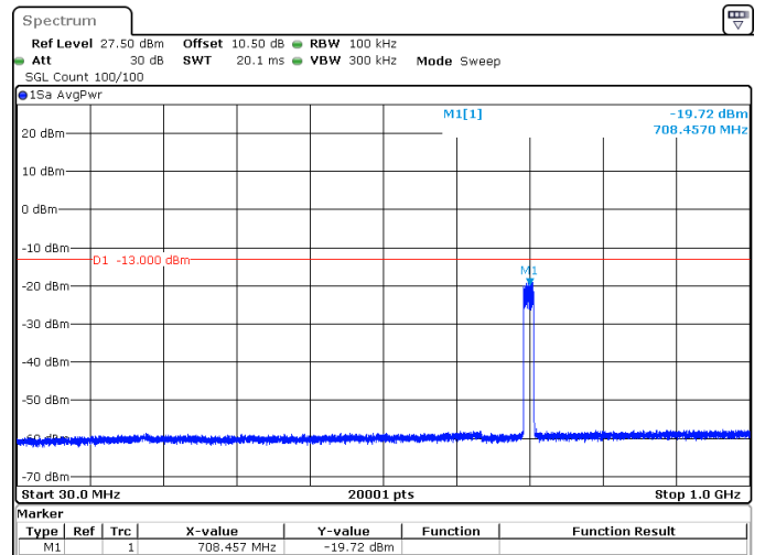
15MHz_15kHz_707.5MHz_DFT-s-OFDM QPSK_RB75@0 -19.72 dBm
