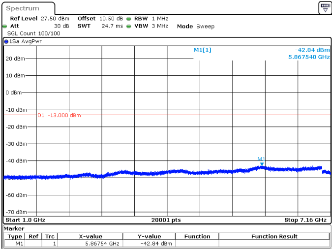
5MHz_15kHz_713.5MHz_DFT-s-OFDM QPSK_RB25@0 -42.84 dBm
