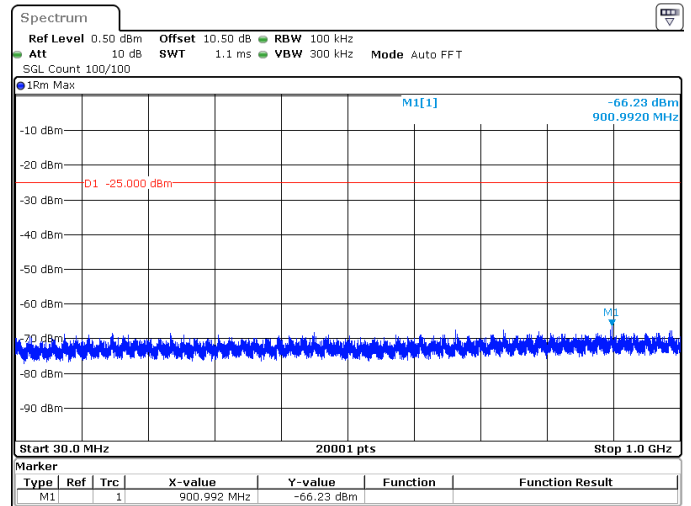
25MHz_30kHz_2582.5MHz_DFT-s-OFDM QPSK_RB1@64 -66.23 dBm
