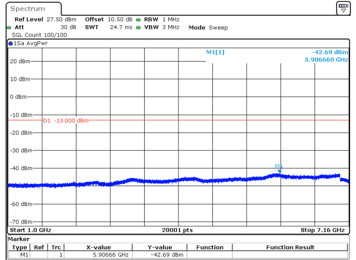
15MHz_15kHz_707.5MHz_DFT-s-OFDM QPSK_RB1@0 -42.69 dBm
