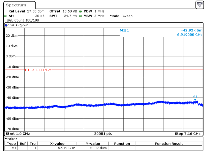
15MHz_15kHz_708.5MHz_DFT-s-OFDM QPSK_RB1@0 -42.92 dBm
