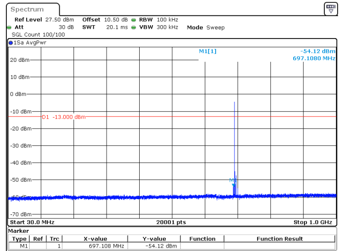
10MHz_15kHz_704MHz_DFT-s-OFDM QPSK_RB1@0 -54.12 dBm
