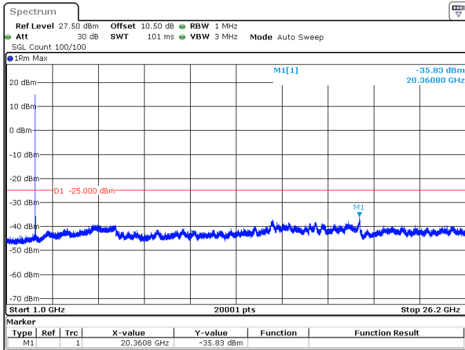
25MHz_30kHz_2582.5MHz_DFT-s-OFDM QPSK_RB1@0 -35.83 dBm
