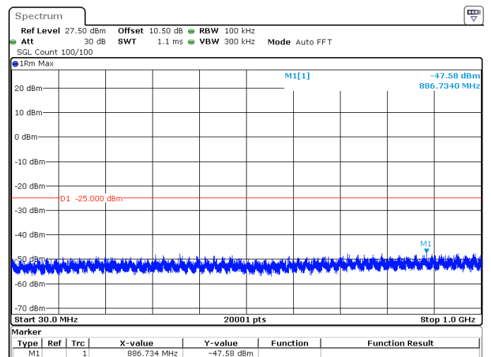
15MHz_30kHz_2595MHz_DFT-s-OFDM QPSK_RB36@0 -47.58 dBm
