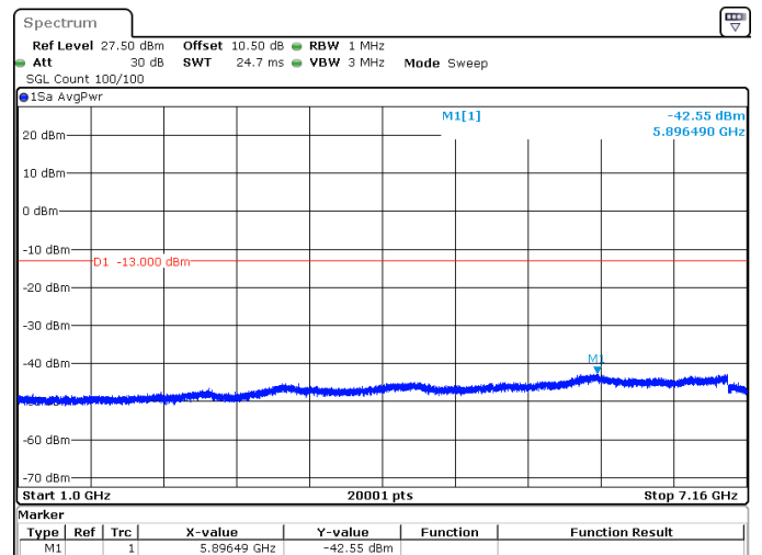
10MHz_15kHz_711MHz_DFT-s-OFDM QPSK_RB1@51 -42.55 dBm
