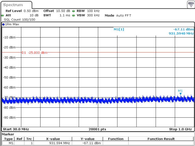
5MHz_15kHz_2572.5MHz_DFT-s-OFDM QPSK_RB1@0 -67.11 dBm
