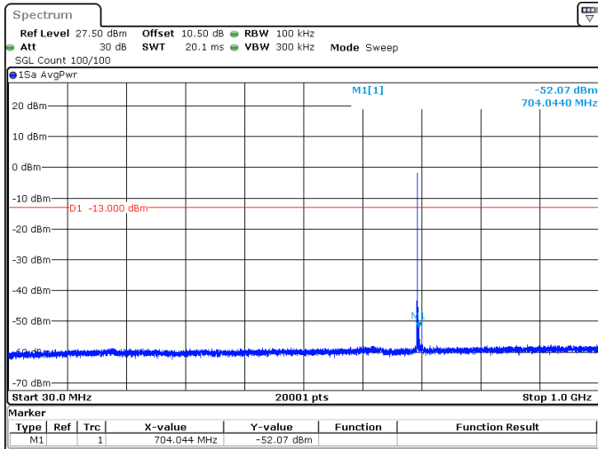
15MHz_15kHz_708.5MHz_DFT-s-OFDM QPSK_RB1@0 -52.07 dBm
