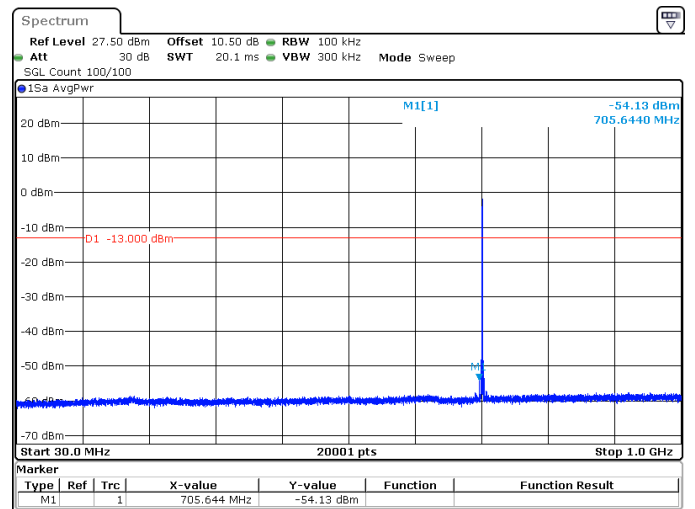
5MHz_15kHz_707.5MHz_DFT-s-OFDM QPSK_RB1@24 -54.13 dBm
