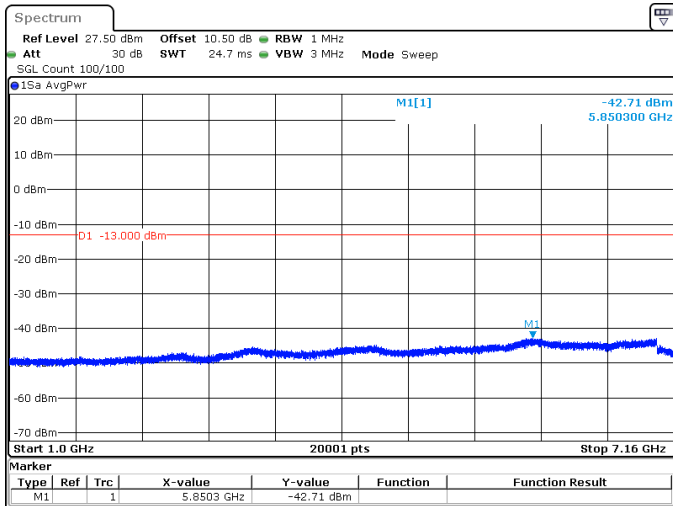
15MHz_15kHz_707.5MHz_DFT-s-OFDM QPSK_RB1@78 -42.71 dBm
