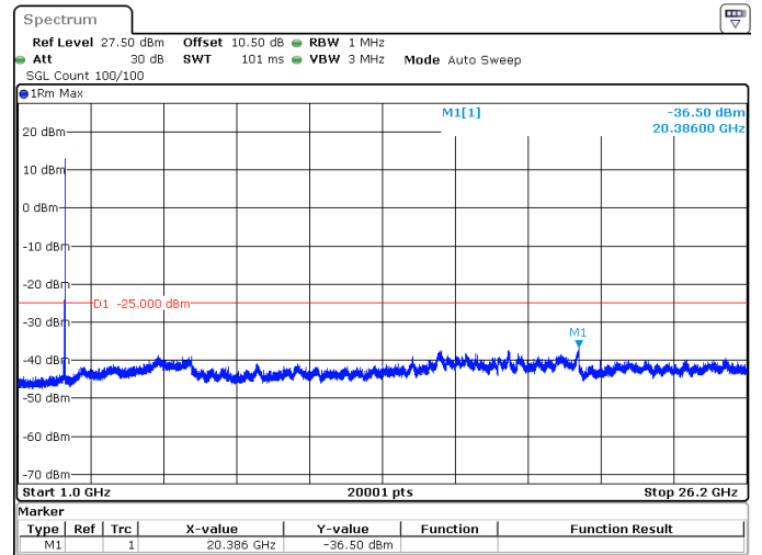
40MHz_30kHz_2595MHz_DFT-s-OFDM QPSK_RB1@105 -36.50 dBm
