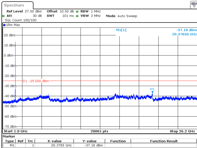
40MHz_30kHz_2600MHz_DFT-s-OFDM QPSK_RB1@105 -37.18 dBm
