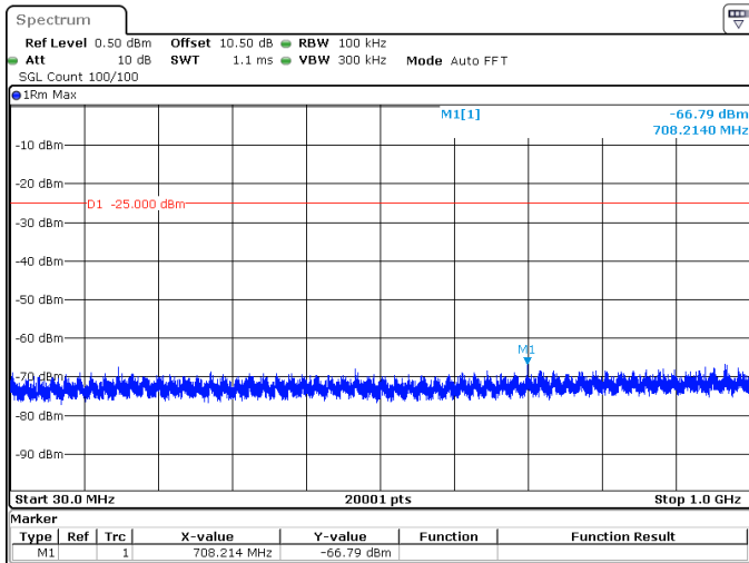
40MHz_30kHz_2595MHz_DFT-s-OFDM QPSK_RB1@105 -66.79 dBm
