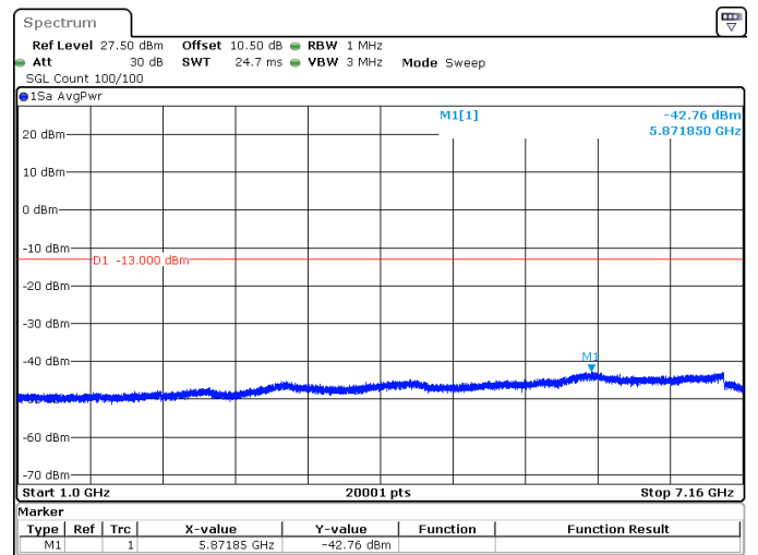
10MHz_15kHz_707.5MHz_DFT-s-OFDM QPSK_RB1@51 -42.76 dBm
