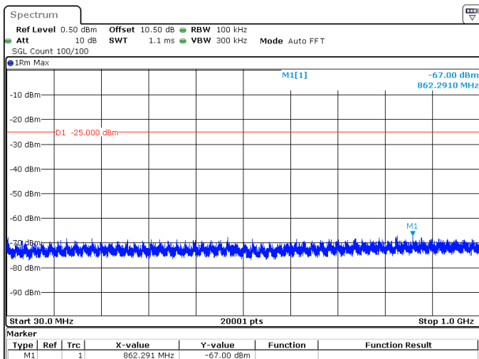
40MHz_30kHz_2595MHz_DFT-s-OFDM QPSK_RB100@0 -67.00 dBm
