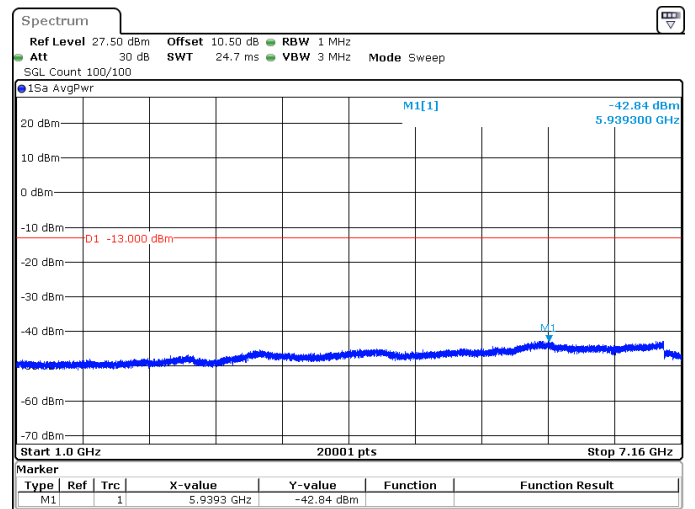
10MHz_15kHz_704MHz_DFT-s-OFDM QPSK_RB1@51 -42.84 dBm
