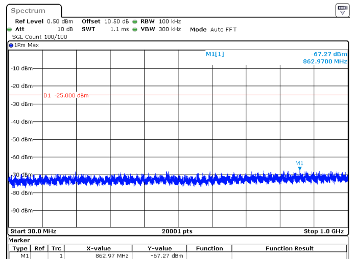
15MHz_30kHz_2595MHz_DFT-s-OFDM QPSK_RB1@37 -67.27 dBm
