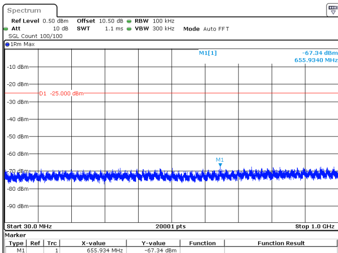
15MHz_30kHz_2577.5MHz_DFT-s-OFDM QPSK_RB36@0 -67.34 dBm
