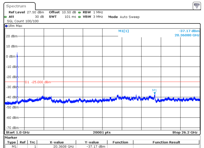
40MHz_30kHz_2595MHz_DFT-s-OFDM QPSK_RB100@0 -37.17 dBm
