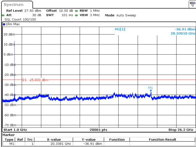
5MHz_15kHz_2572.5MHz_DFT-s-OFDM QPSK_RB1@24 -36.91 dBm
