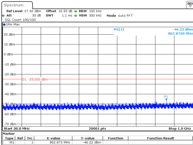
5MHz_15kHz_2595MHz_DFT-s-OFDM QPSK_RB1@24 -46.22 dBm
