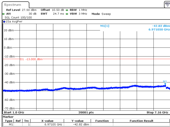
10MHz_15kHz_704MHz_DFT-s-OFDM QPSK_RB1@0 -42.82 dBm
