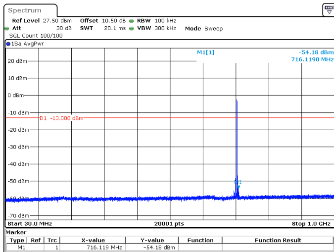
10MHz_15kHz_707.5MHz_DFT-s-OFDM QPSK_RB1@51 -54.18 dBm
