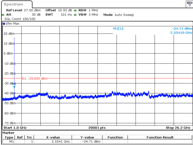
5MHz_15kHz_2572.5MHz_DFT-s-OFDM QPSK_RB1@0 -34.71 dBm
