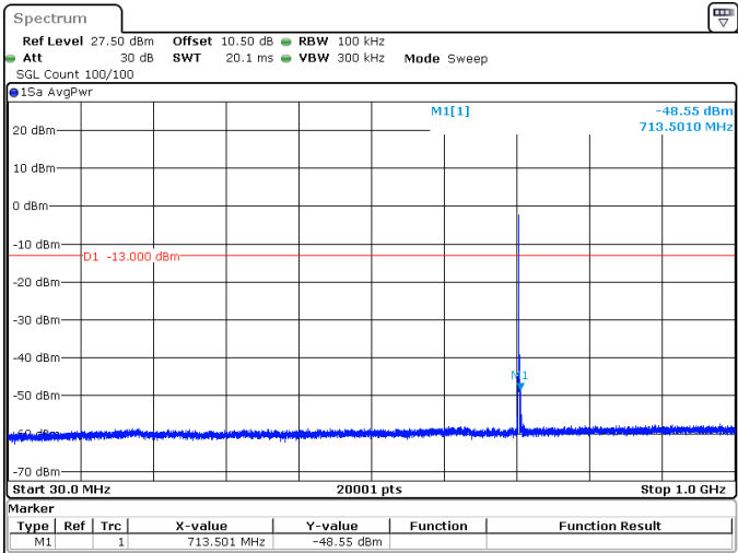
5MHz_15kHz_713.5MHz_DFT-s-OFDM QPSK_RB1@0 -48.55 dBm
