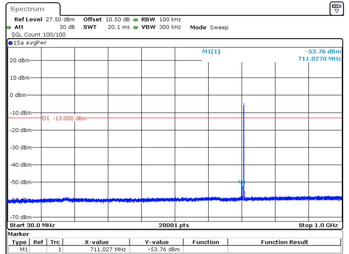
15MHz_15kHz_707.5MHz_DFT-s-OFDM QPSK_RB1@78 -53.76 dBm
