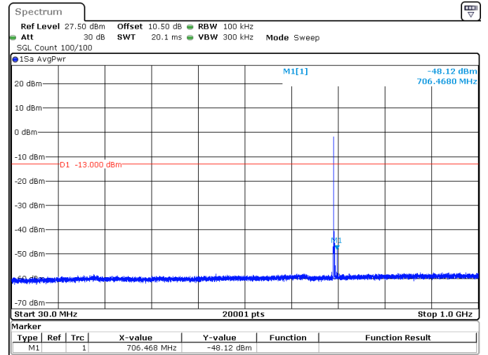
15MHz_15kHz_706.5MHz_DFT-s-OFDM QPSK_RB1@0 -48.12 dBm
