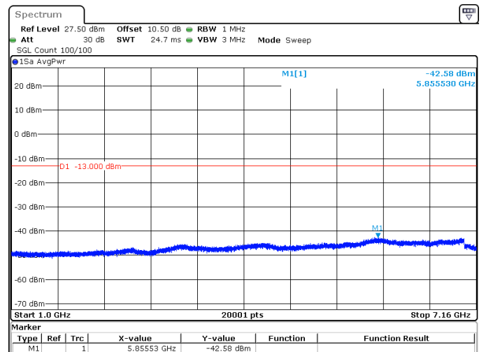
15MHz_15kHz_706.5MHz_DFT-s-OFDM QPSK_RB75@0 -42.58 dBm
