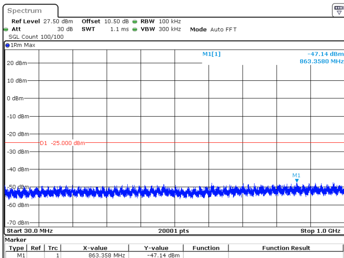
15MHz_30kHz_2612.5MHz_DFT-s-OFDM QPSK_RB36@0 -47.14 dBm
