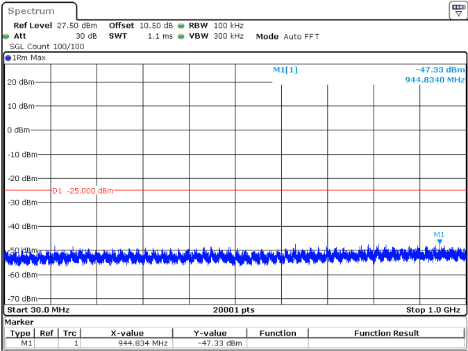
5MHz_15kHz_2572.5MHz_DFT-s-OFDM QPSK_RB1@24 -47.33 dBm
