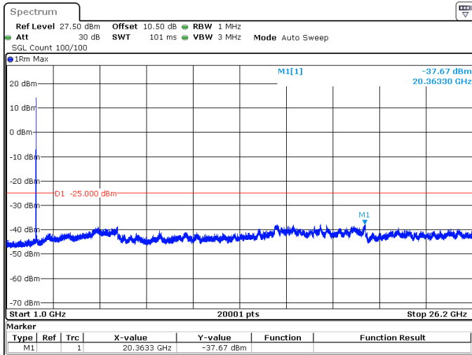
40MHz_30kHz_2600MHz_DFT-s-OFDM QPSK_RB1@0 -37.67 dBm
