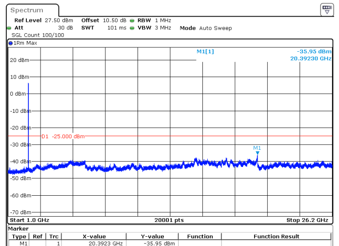
15MHz_30kHz_2577.5MHz_DFT-s-OFDM QPSK_RB36@0 -35.95 dBm
