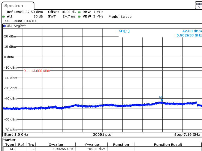
15MHz_15kHz_707.5MHz_DFT-s-OFDM QPSK_RB75@0 -42.38 dBm
