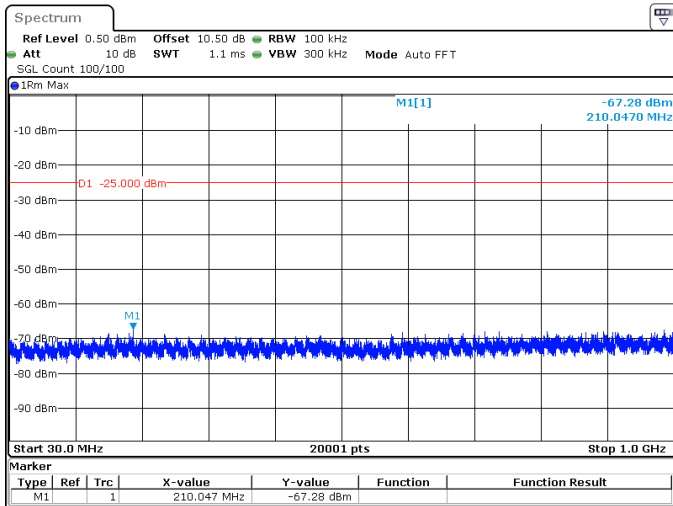
30MHz_30kHz_2605MHz_DFT-s-OFDM QPSK_RB1@77 -67.28 dBm
