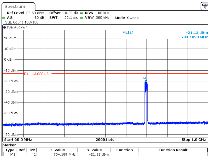
15MHz_15kHz_706.5MHz_DFT-s-OFDM QPSK_RB75@0 -21.15 dBm
