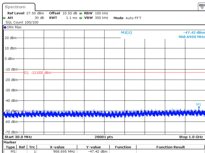
40MHz_15kHz_1760MHz_DFT-s-OFDM QPSK_RB216@0 -47.42 dBm
