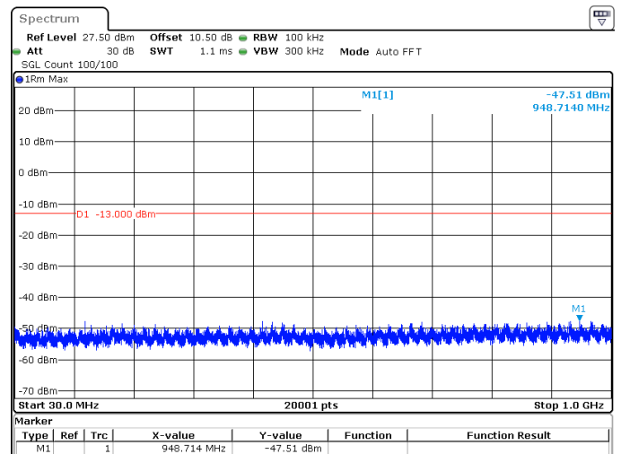
5MHz_15kHz_1777.5MHz_DFT-s-OFDM QPSK_RB1@24 -47.51 dBm
