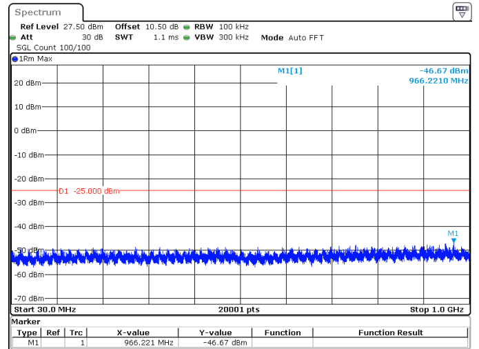
10MHz_15kHz_2535MHz_DFT-s-OFDM QPSK_RB1@51 -46.67 dBm
