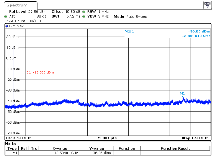
15MHz_15kHz_1717.5MHz_DFT-s-OFDM QPSK_RB1@0 -36.86 dBm
