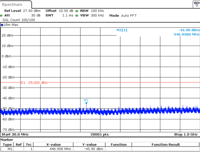
100MHz_30kHz_2546.01MHz_DFT-s-OFDM QPSK_RB1@0 -45.90 dBm
