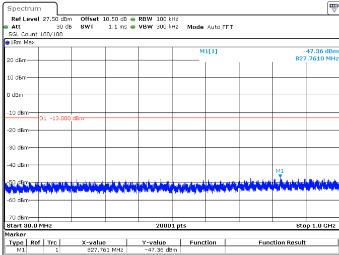
10MHz_15kHz_1715MHz_DFT-s-OFDM QPSK_RB1@0 -47.36 dBm
