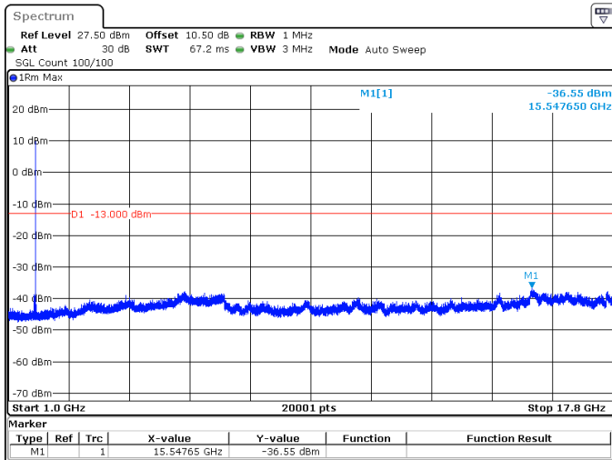
30MHz_15kHz_1725MHz_DFT-s-OFDM QPSK_RB1@159 -36.55 dBm
