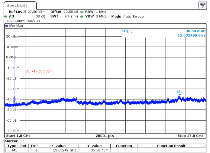
40MHz_15kHz_1745MHz_DFT-s-OFDM QPSK_RB1@215 -36.58 dBm
