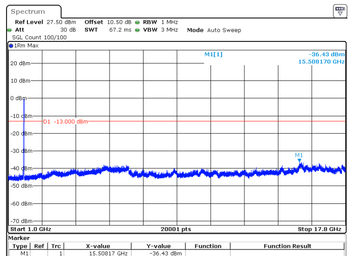
25MHz_15kHz_1767.5MHz_DFT-s-OFDM QPSK_RB128@0 -36.43 dBm
