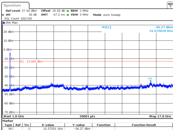
40MHz_15kHz_1745MHz_DFT-s-OFDM QPSK_RB216@0 -36.27 dBm
