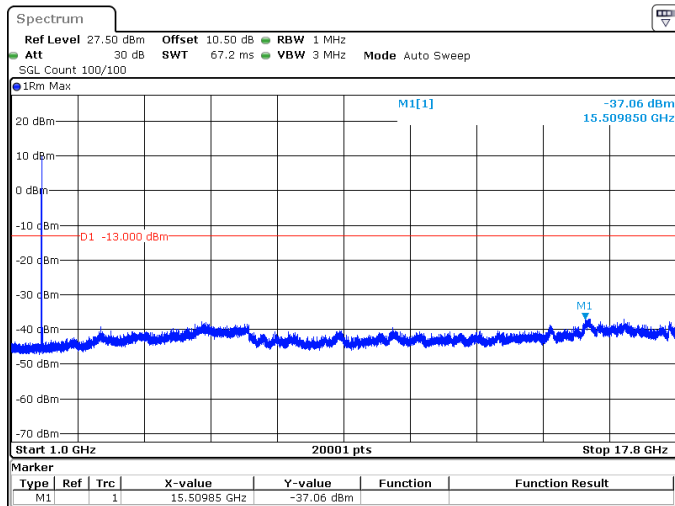
25MHz_15kHz_1767.5MHz_DFT-s-OFDM QPSK_RB1@0 -37.06 dBm
