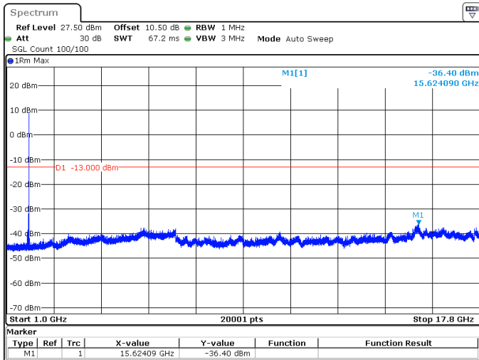
30MHz_15kHz_1765MHz_DFT-s-OFDM QPSK_RB1@159 -36.40 dBm
