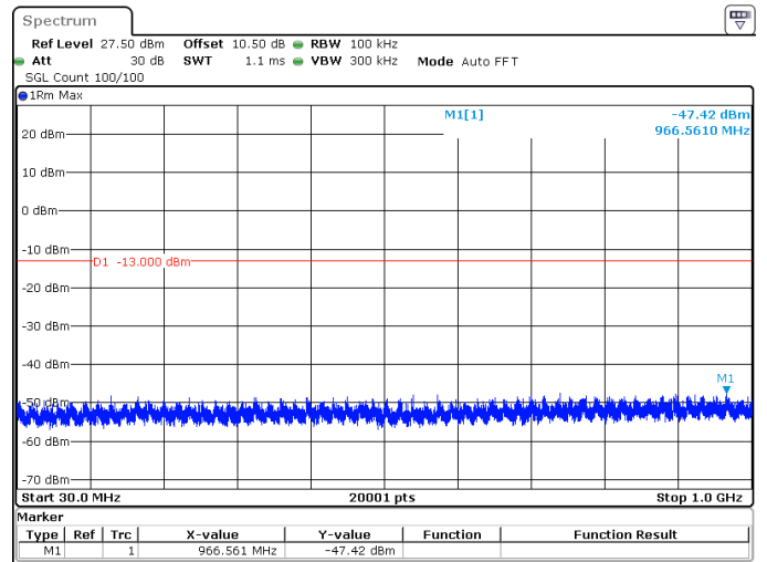
25MHz_15kHz_1722.5MHz_DFT-s-OFDM QPSK_RB1@0 -47.42 dBm
