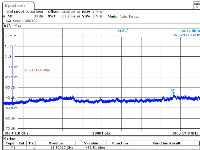
15MHz_15kHz_1772.5MHz_DFT-s-OFDM QPSK_RB1@0 -36.51 dBm
