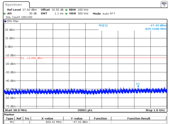
15MHz_15kHz_1772.5MHz_DFT-s-OFDM QPSK_RB1@0 -47.43 dBm
