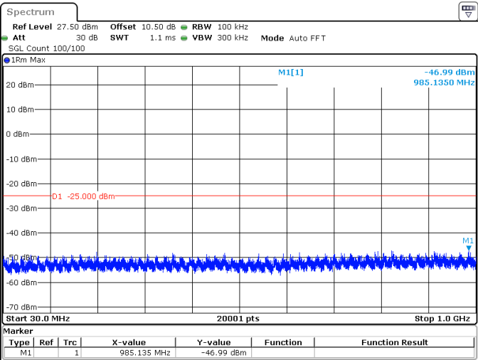
5MHz_15kHz_2567.5MHz_DFT-s-OFDM QPSK_RB1@0 -46.99 dBm
