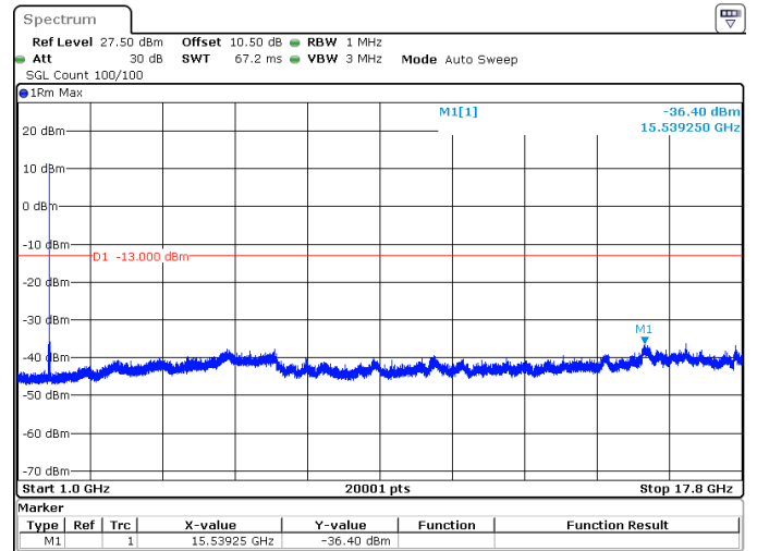
15MHz_15kHz_1717.5MHz_DFT-s-OFDM QPSK_RB1@78 -36.40 dBm
