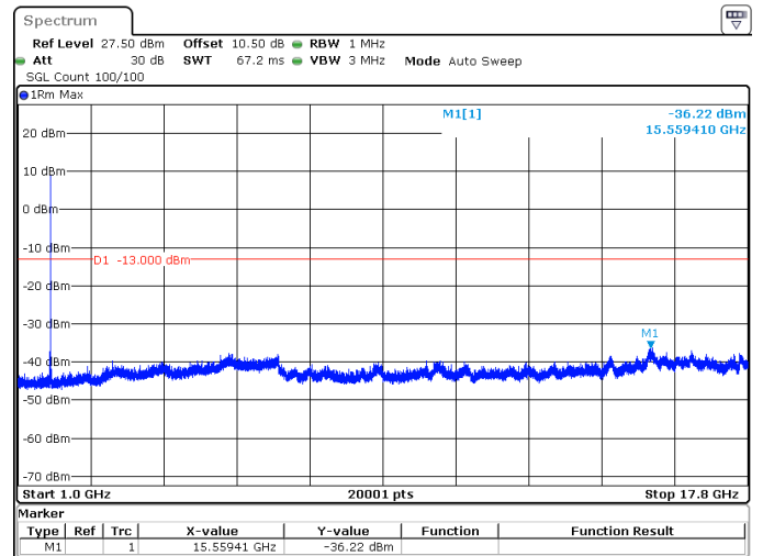
15MHz_15kHz_1745MHz_DFT-s-OFDM QPSK_RB1@0 -36.22 dBm
