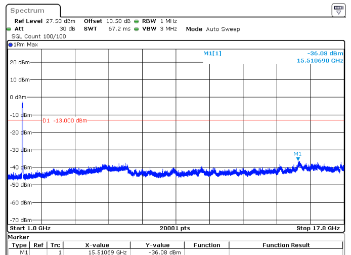
40MHz_15kHz_1730MHz_DFT-s-OFDM QPSK_RB216@0 -36.08 dBm
