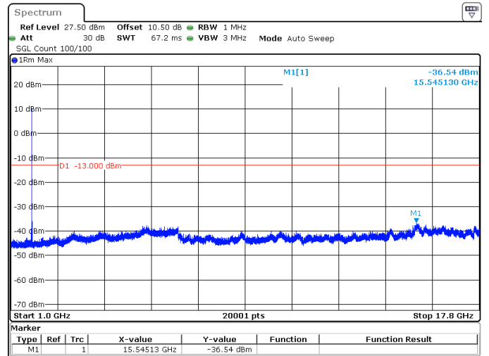
10MHz_15kHz_1745MHz_DFT-s-OFDM QPSK_RB1@51 -36.54 dBm
