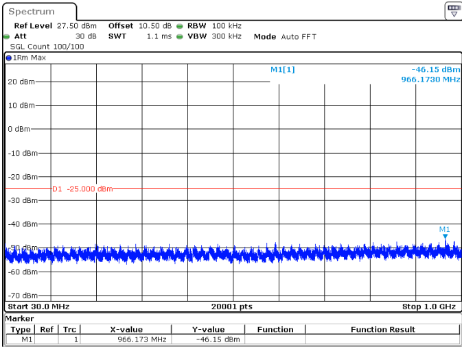
5MHz_15kHz_2567.5MHz_DFT-s-OFDM QPSK_RB25@0 -46.15 dBm
