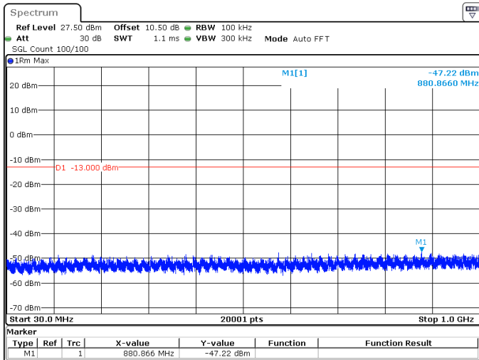
40MHz_15kHz_1745MHz_DFT-s-OFDM QPSK_RB1@215 -47.22 dBm
