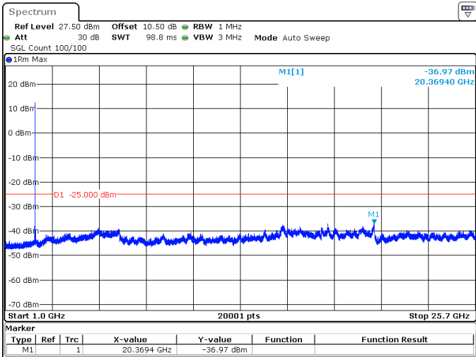
5MHz_15kHz_2567.5MHz_DFT-s-OFDM QPSK_RB1@0 -36.97 dBm
