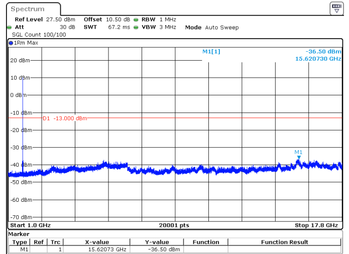
10MHz_15kHz_1715MHz_DFT-s-OFDM QPSK_RB1@51 -36.50 dBm
