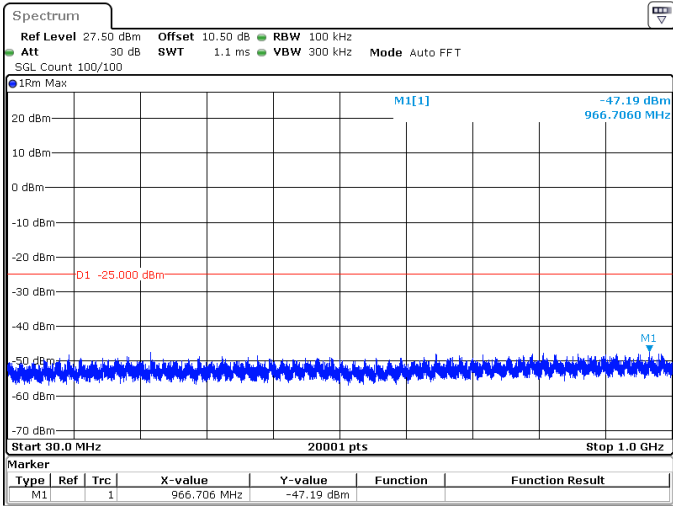
5MHz_15kHz_2567.5MHz_DFT-s-OFDM QPSK_RB1@24 -47.19 dBm
