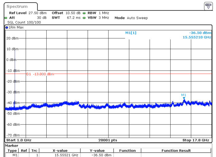
40MHz_15kHz_1760MHz_DFT-s-OFDM QPSK_RB1@215 -36.50 dBm
