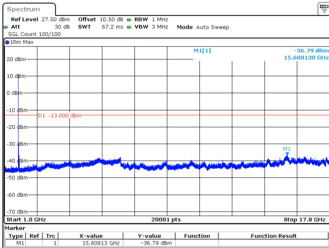
25MHz_15kHz_1722.5MHz_DFT-s-OFDM QPSK_RB1@0 -36.79 dBm
