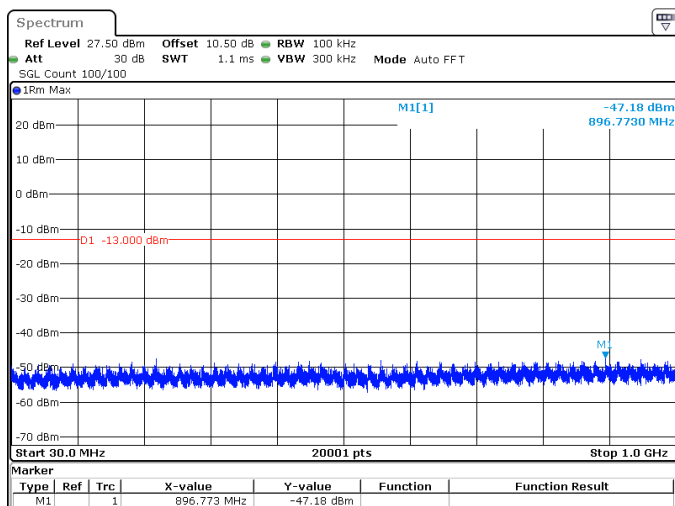
15MHz_15kHz_1745MHz_DFT-s-OFDM QPSK_RB75@0 -47.18 dBm
