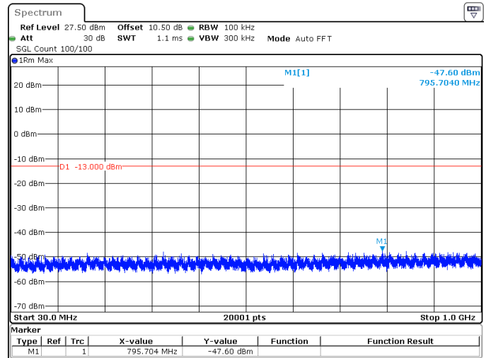
30MHz_15kHz_1725MHz_DFT-s-OFDM QPSK_RB1@159 -47.60 dBm
