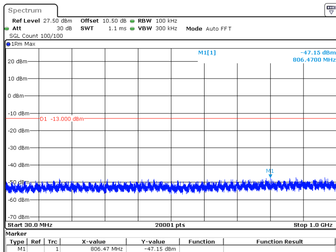
15MHz_15kHz_1745MHz_DFT-s-OFDM QPSK_RB1@78 -47.15 dBm
