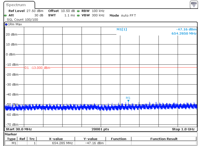
5MHz_15kHz_1745MHz_DFT-s-OFDM QPSK_RB1@0 -47.16 dBm
