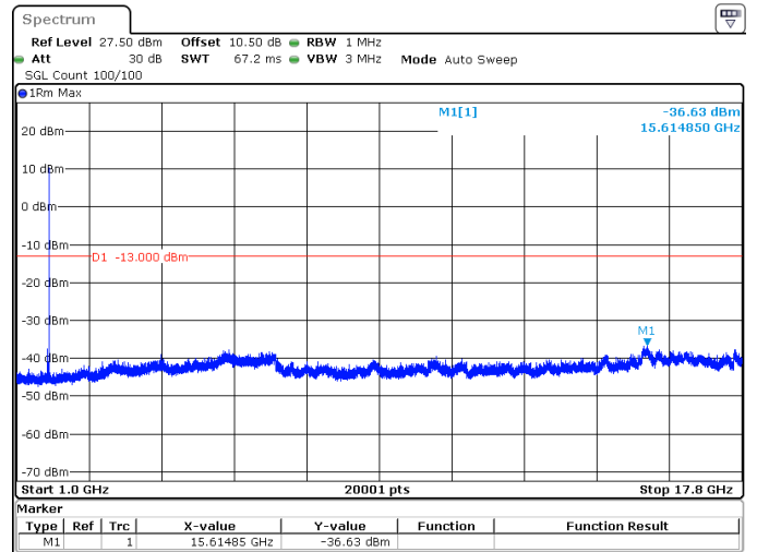
40MHz_15kHz_1730MHz_DFT-s-OFDM QPSK_RB1@215 -36.63 dBm
