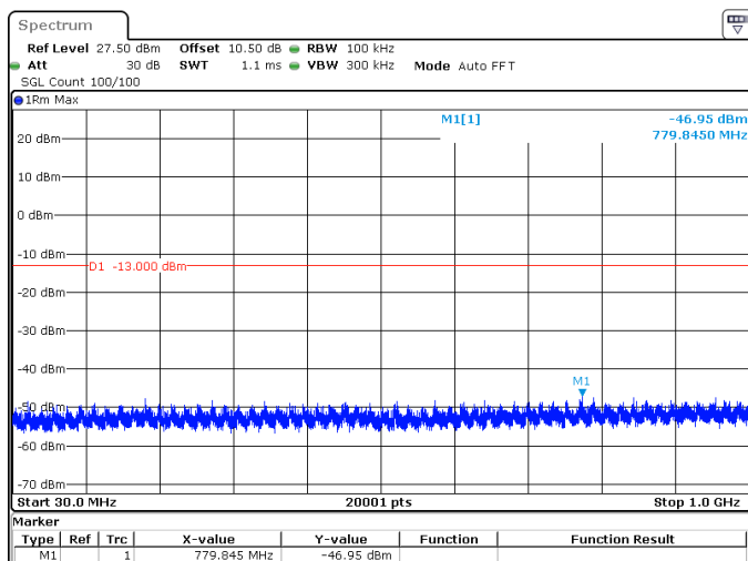
5MHz_15kHz_1777.5MHz_DFT-s-OFDM QPSK_RB25@0 -46.95 dBm
