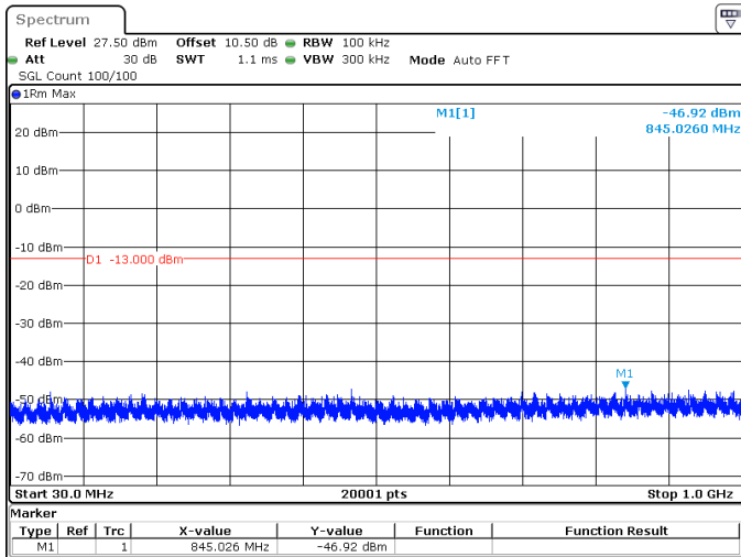
15MHz_15kHz_1717.5MHz_DFT-s-OFDM QPSK_RB1@78 -46.92 dBm
