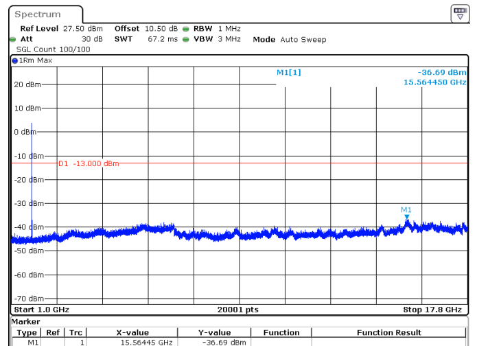
5MHz_15kHz_1745MHz_DFT-s-OFDM QPSK_RB25@0 -36.69 dBm
