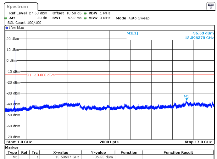
25MHz_15kHz_1767.5MHz_DFT-s-OFDM QPSK_RB1@132 -36.53 dBm
