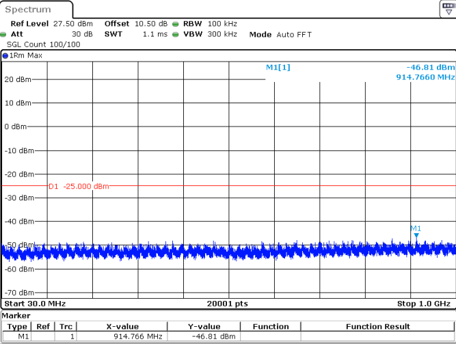
100MHz_30kHz_2546.01MHz_DFT-s-OFDM QPSK_RB270@0 -46.81 dBm
