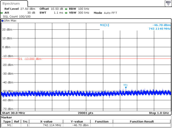
30MHz_15kHz_1745MHz_DFT-s-OFDM QPSK_RB160@0 -46.70 dBm
