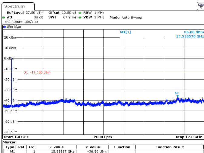
15MHz_15kHz_1717.5MHz_DFT-s-OFDM QPSK_RB75@0 -36.86 dBm
