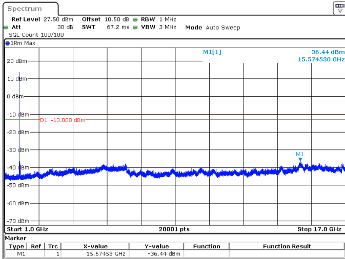
30MHz_15kHz_1725MHz_DFT-s-OFDM QPSK_RB1@0 -36.44 dBm
