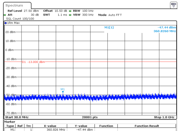
15MHz_15kHz_1717.5MHz_DFT-s-OFDM QPSK_RB75@0 -47.44 dBm
