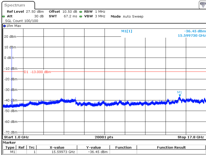
40MHz_15kHz_1745MHz_DFT-s-OFDM QPSK_RB1@0 -36.45 dBm
