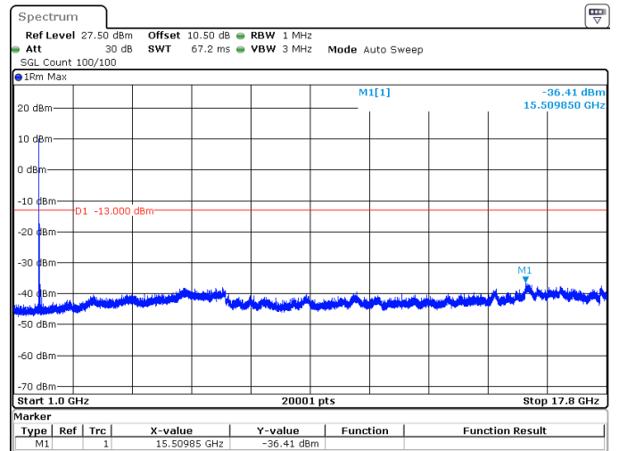
40MHz_15kHz_1730MHz_DFT-s-OFDM QPSK_RB1@0 -36.41 dBm
