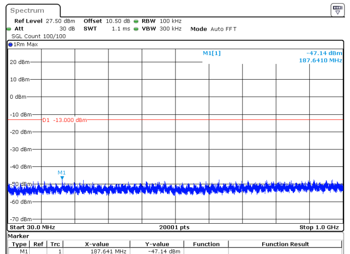
30MHz_15kHz_1765MHz_DFT-s-OFDM QPSK_RB160@0 -47.14 dBm
