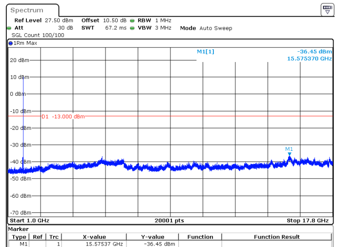
15MHz_15kHz_1772.5MHz_DFT-s-OFDM QPSK_RB1@78 -36.45 dBm
