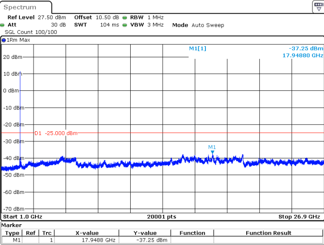
100MHz_30kHz_2546.01MHz_DFT-s-OFDM QPSK_RB1@0 -37.25 dBm
