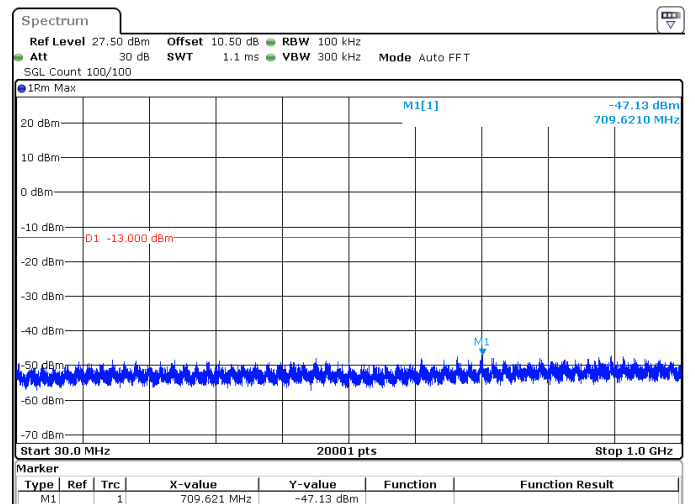
40MHz_15kHz_1745MHz_DFT-s-OFDM QPSK_RB216@0 -47.13 dBm
