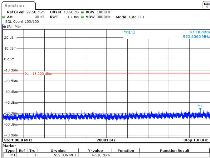
5MHz_15kHz_1745MHz_DFT-s-OFDM QPSK_RB1@24 -47.10 dBm
