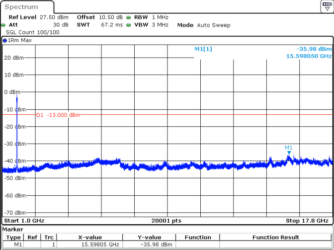
30MHz_15kHz_1745MHz_DFT-s-OFDM QPSK_RB160@0 -35.98 dBm
