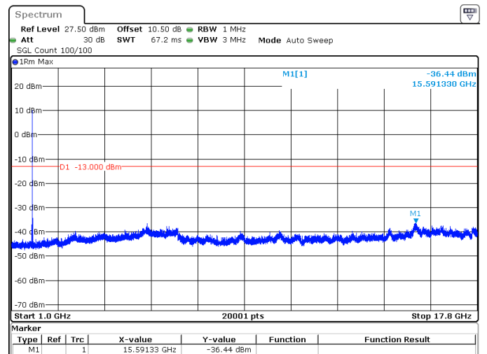
15MHz_15kHz_1745MHz_DFT-s-OFDM QPSK_RB1@78 -36.44 dBm
