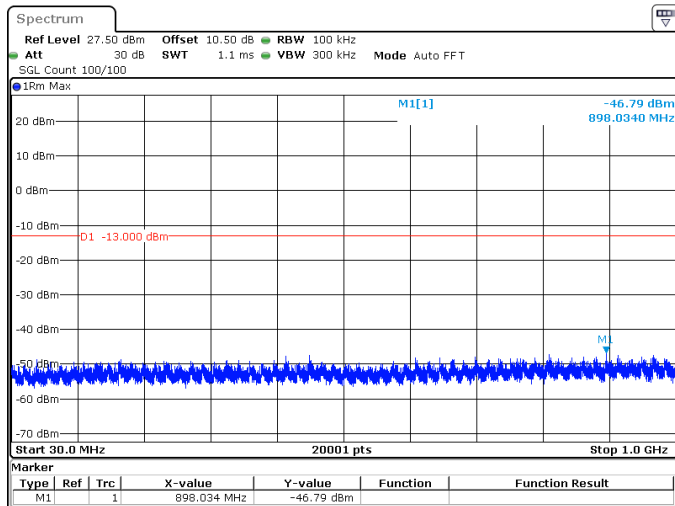
15MHz_15kHz_1745MHz_DFT-s-OFDM QPSK_RB1@0 -46.79 dBm
