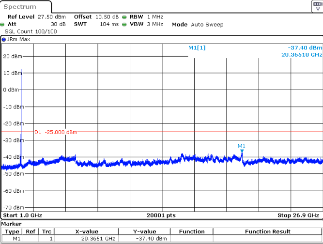
100MHz_30kHz_2546.01MHz_DFT-s-OFDM QPSK_RB1@272 -37.40 dBm
