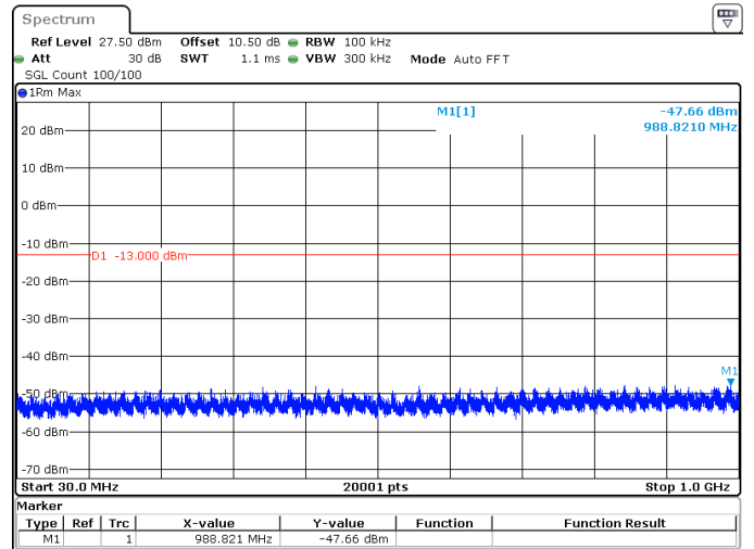
30MHz_15kHz_1765MHz_DFT-s-OFDM QPSK_RB1@159 -47.66 dBm
