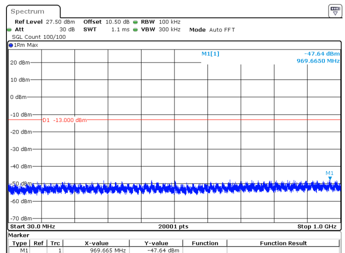
15MHz_15kHz_1772.5MHz_DFT-s-OFDM QPSK_RB75@0 -47.64 dBm
