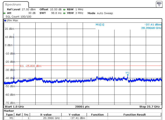
5MHz_15kHz_2535MHz_DFT-s-OFDM QPSK_RB1@0 -37.41 dBm
