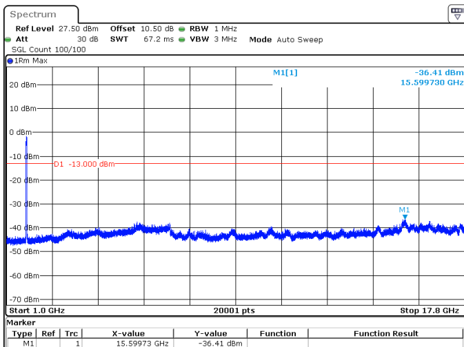
30MHz_15kHz_1725MHz_DFT-s-OFDM QPSK_RB160@0 -36.41 dBm
