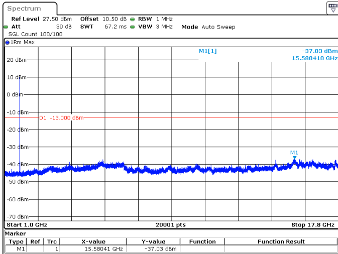
5MHz_15kHz_1745MHz_DFT-s-OFDM QPSK_RB1@0 -37.03 dBm
