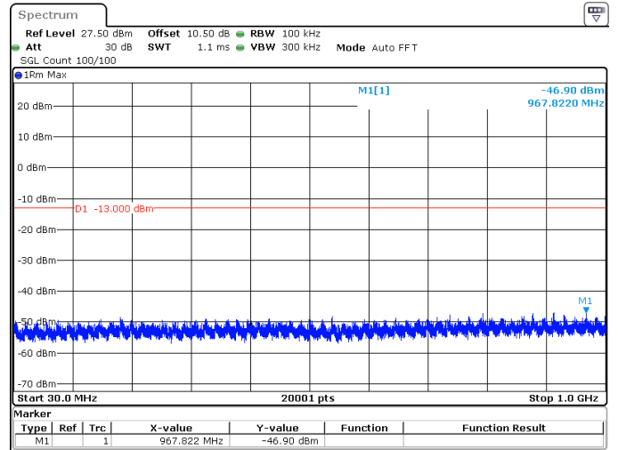
30MHz_15kHz_1725MHz_DFT-s-OFDM QPSK_RB1@0 -46.90 dBm
