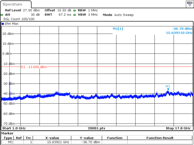
30MHz_15kHz_1745MHz_DFT-s-OFDM QPSK_RB1@0 -36.70 dBm
