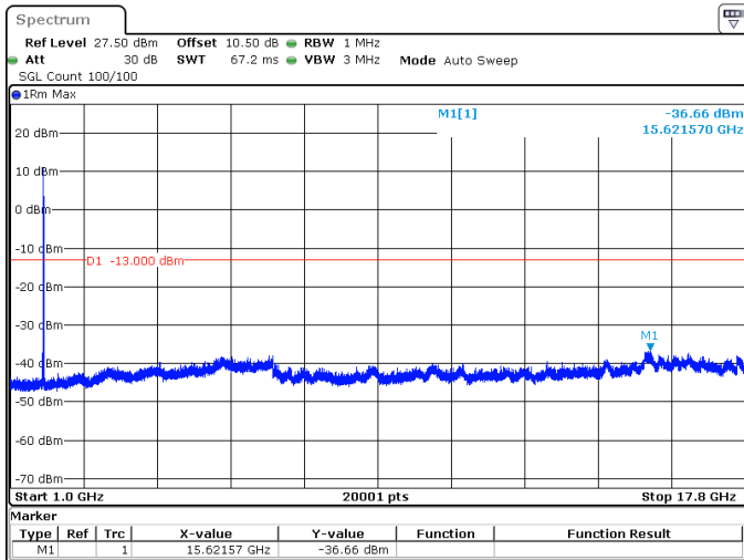
20MHz_15kHz_1745MHz_DFT-s-OFDM QPSK_RB1@105 -36.66 dBm
