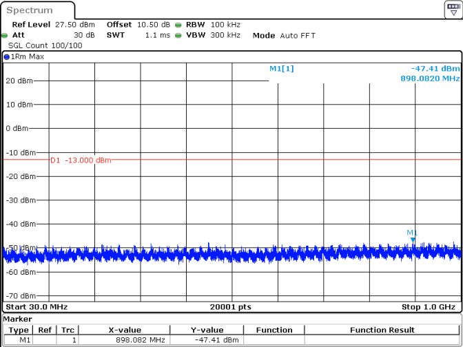
30MHz_15kHz_1745MHz_DFT-s-OFDM QPSK_RB1@0 -47.41 dBm
