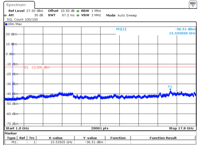
10MHz_15kHz_1715MHz_DFT-s-OFDM QPSK_RB1@0 -36.51 dBm
