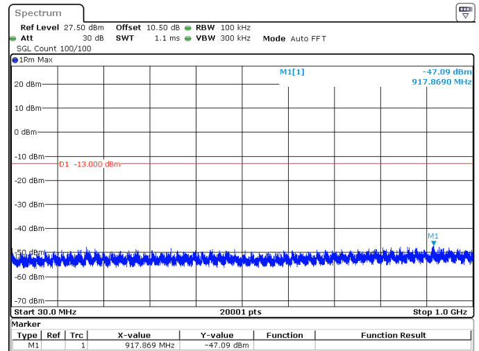
25MHz_15kHz_1767.5MHz_DFT-s-OFDM QPSK_RB1@0 -47.09 dBm
