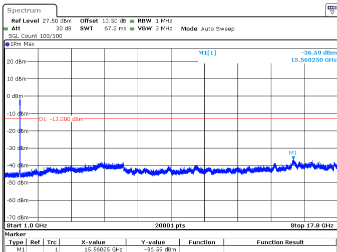
30MHz_15kHz_1765MHz_DFT-s-OFDM QPSK_RB160@0 -36.59 dBm
