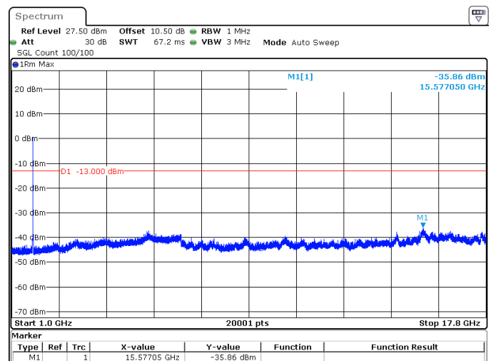
15MHz_15kHz_1745MHz_DFT-s-OFDM QPSK_RB75@0 -35.86 dBm
