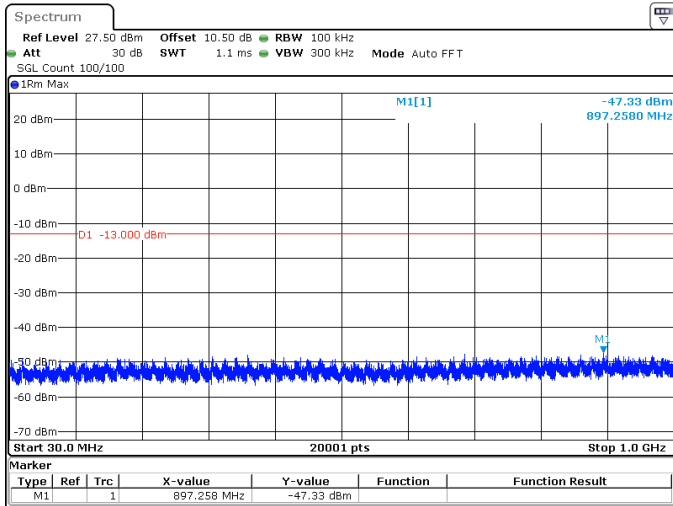
15MHz_15kHz_1717.5MHz_DFT-s-OFDM QPSK_RB1@0 -47.33 dBm
