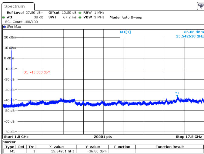
25MHz_15kHz_1722.5MHz_DFT-s-OFDM QPSK_RB1@132 -36.86 dBm
