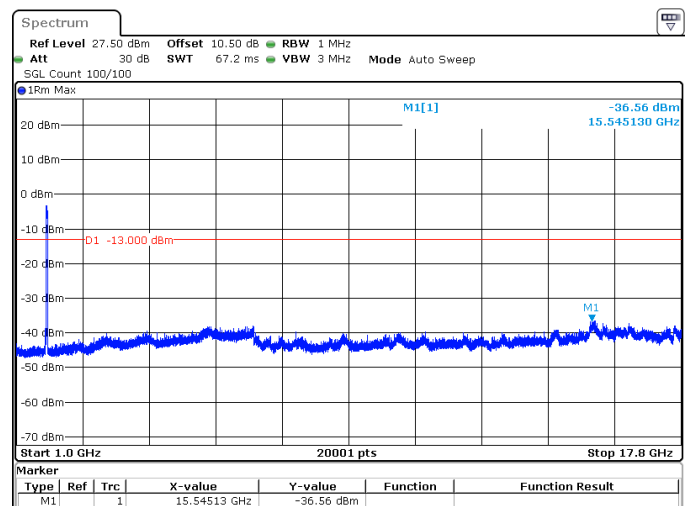
40MHz_15kHz_1760MHz_DFT-s-OFDM QPSK_RB216@0 -36.56 dBm
