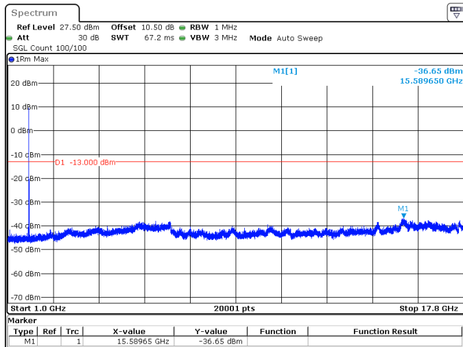
5MHz_15kHz_1777.5MHz_DFT-s-OFDM QPSK_RB1@0 -36.65 dBm
