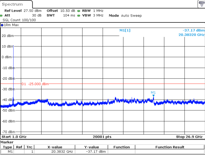
100MHz_30kHz_2592.99MHz_DFT-s-OFDM QPSK_RB1@272 -37.17 dBm
