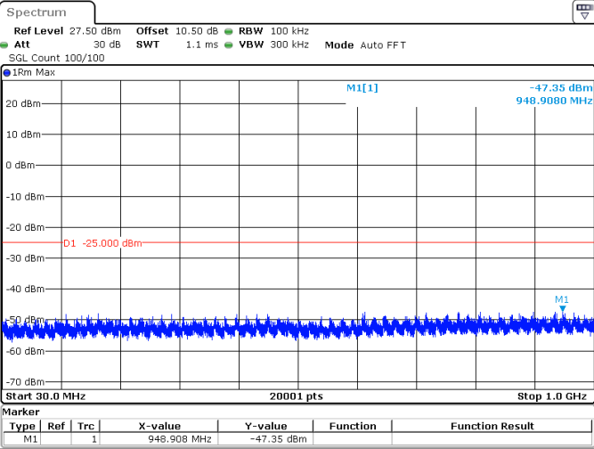
100MHz_30kHz_2592.99MHz_DFT-s-OFDM QPSK_RB1@272 -47.35 dBm
