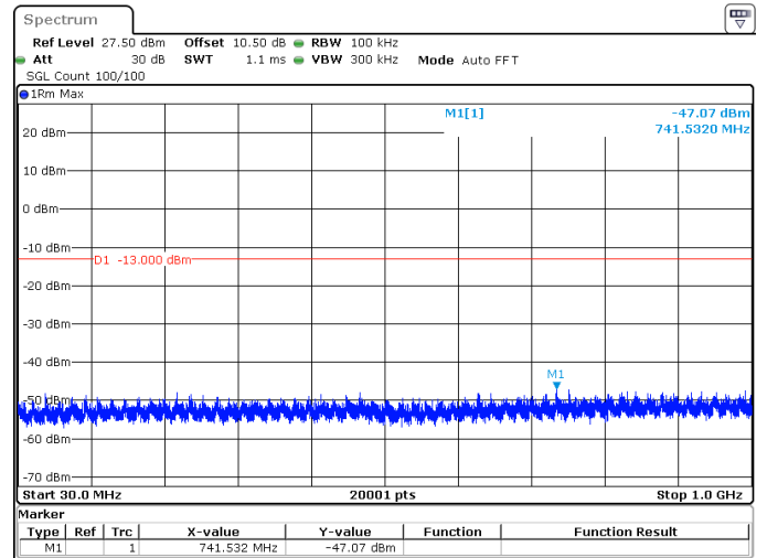
10MHz_15kHz_1775MHz_DFT-s-OFDM QPSK_RB1@51 -47.07 dBm
