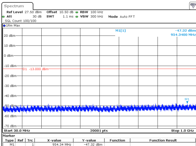
40MHz_15kHz_1730MHz_DFT-s-OFDM QPSK_RB216@0 -47.32 dBm
