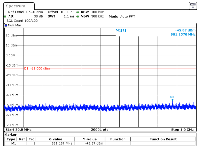
25MHz_15kHz_1722.5MHz_DFT-s-OFDM QPSK_RB1@132 -45.87 dBm
