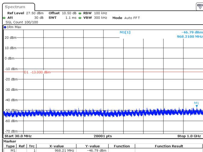
25MHz_15kHz_1767.5MHz_DFT-s-OFDM QPSK_RB128@0 -46.79 dBm
