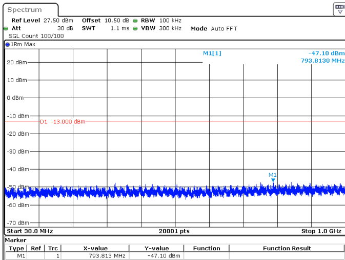
40MHz_15kHz_1730MHz_DFT-s-OFDM QPSK_RB1@0 -47.10 dBm
