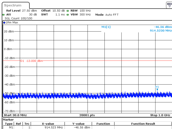
25MHz_15kHz_1767.5MHz_DFT-s-OFDM QPSK_RB1@132 -46.56 dBm
