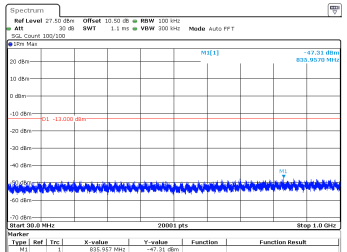
30MHz_15kHz_1725MHz_DFT-s-OFDM QPSK_RB160@0 -47.31 dBm
