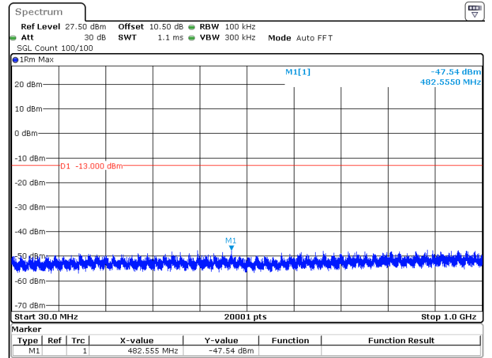
40MHz_15kHz_1745MHz_DFT-s-OFDM QPSK_RB1@0 -47.54 dBm
