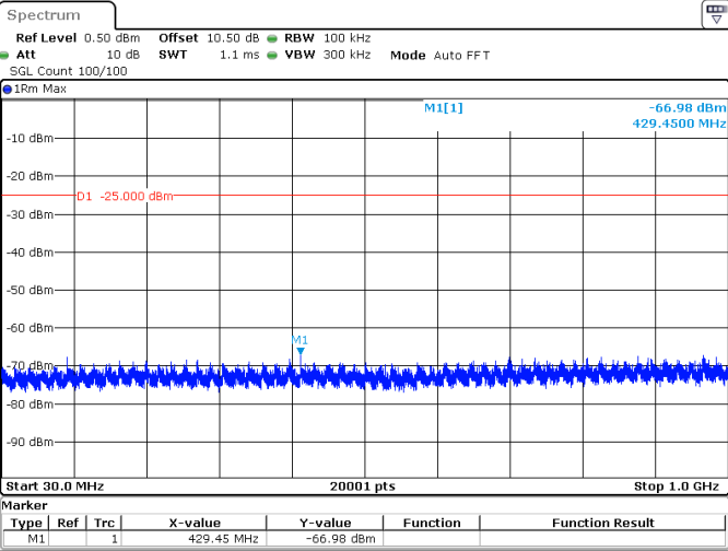
100MHz_30kHz_2546.01MHz_DFT-s-OFDM QPSK_RB1@272 -66.98 dBm
