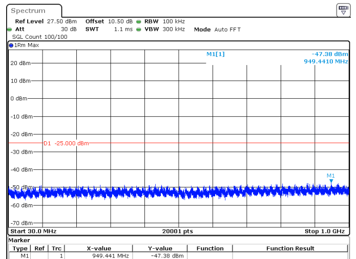
5MHz_15kHz_2535MHz_DFT-s-OFDM QPSK_RB1@24 -47.38 dBm
