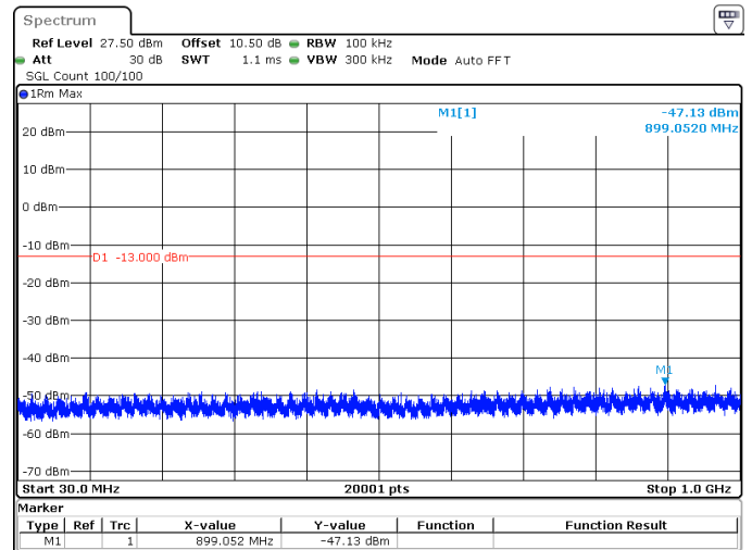
5MHz_15kHz_1777.5MHz_DFT-s-OFDM QPSK_RB1@0 -47.13 dBm
