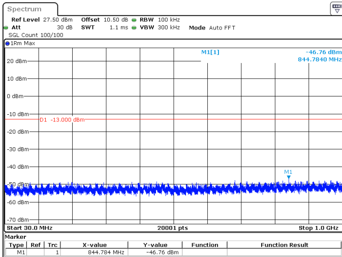
10MHz_15kHz_1715MHz_DFT-s-OFDM QPSK_RB1@51 -46.76 dBm
