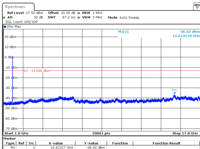
15MHz_15kHz_1772.5MHz_DFT-s-OFDM QPSK_RB75@0 -36.02 dBm
