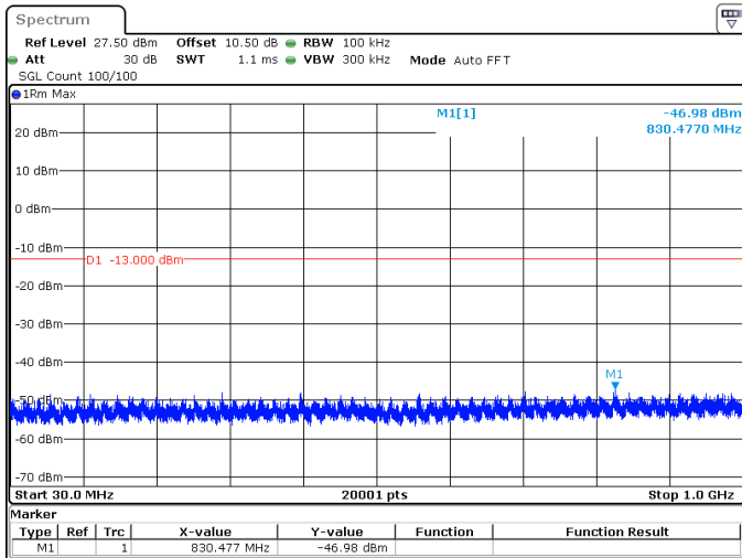
40MHz_15kHz_1730MHz_DFT-s-OFDM QPSK_RB1@215 -46.98 dBm
