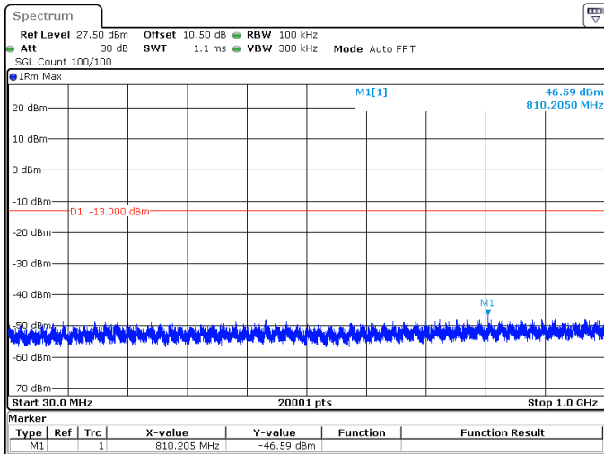
10MHz_15kHz_1745MHz_DFT-s-OFDM QPSK_RB1@51 -46.59 dBm
