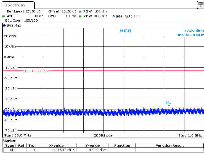
15MHz_30kHz_3542.5MHz_DFT-s-OFDM QPSK_RB1@0 -47.29 dBm
