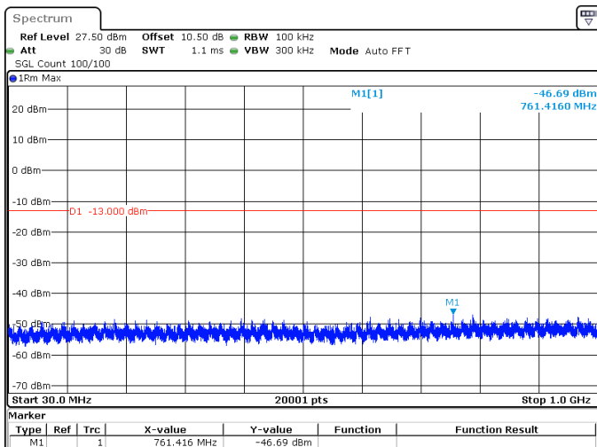
15MHz_30kHz_3542.5MHz_DFT-s-OFDM QPSK_RB36@0 -46.69 dBm
