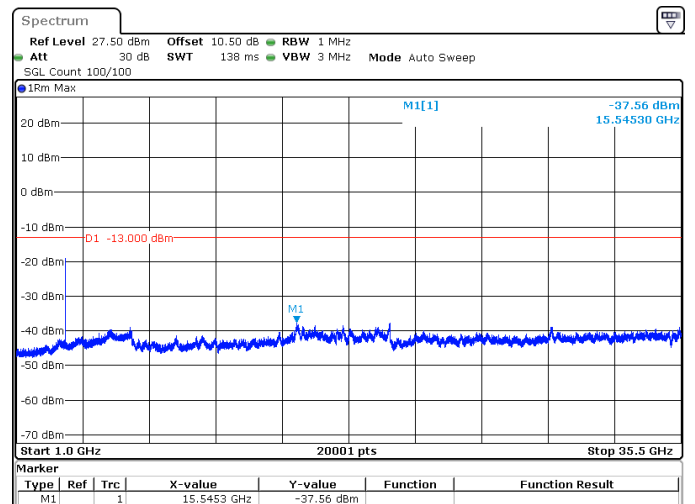
15MHz_30kHz_3542.5MHz_DFT-s-OFDM QPSK_RB36@0 -37.56 dBm
