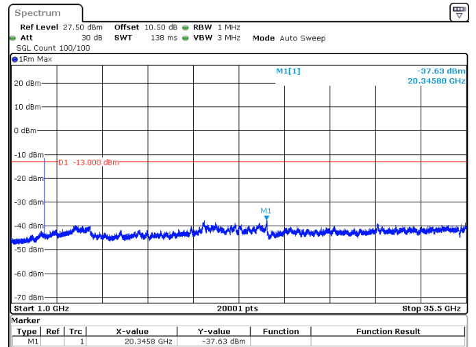
15MHz_30kHz_3500MHz_DFT-s-OFDM QPSK_RB1@0 -37.63 dBm
