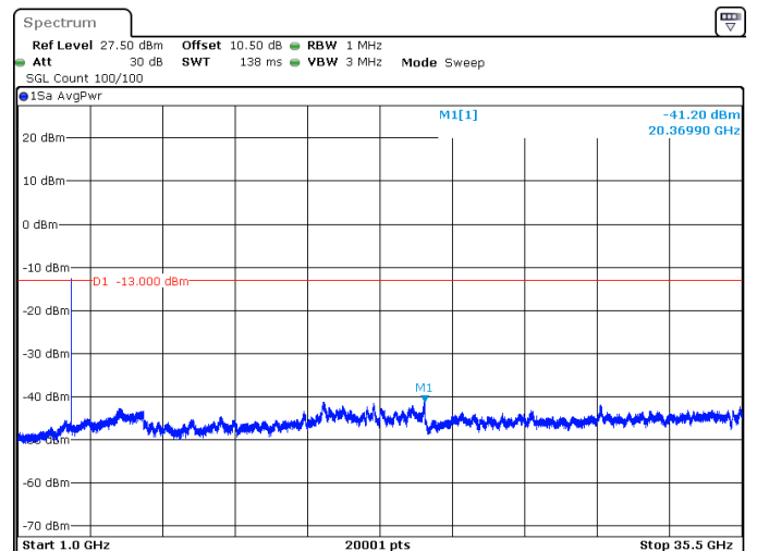
15MHz_15kHz_3542.5MHz_DFT-s-OFDM QPSK_RB75@0 -41.20 dBm
