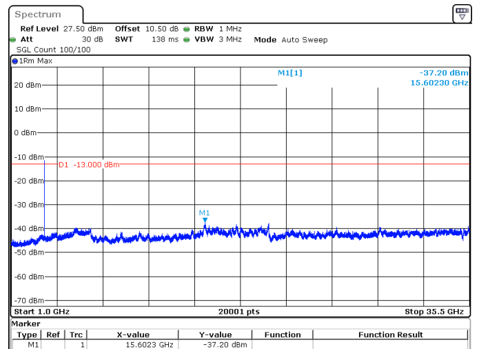
15MHz_30kHz_3500MHz_DFT-s-OFDM QPSK_RB1@37 -37.20 dBm
