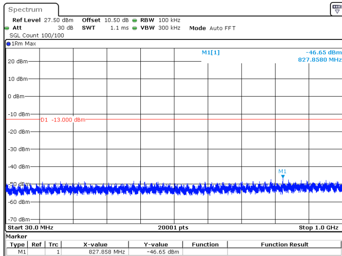
10MHz_15kHz_3545MHz_DFT-s-OFDM QPSK_RB1@0 -46.65 dBm
