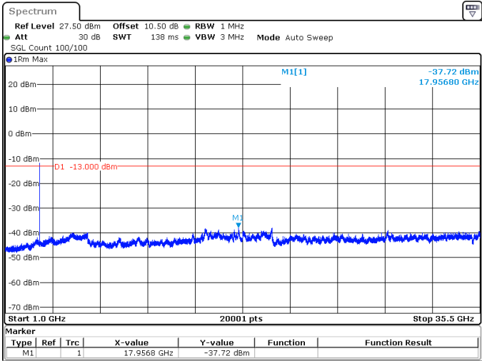
15MHz_15kHz_3500MHz_DFT-s-OFDM QPSK_RB1@78 -37.72 dBm
