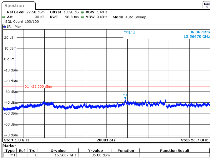
15MHz_15kHz_2535MHz_DFT-s-OFDM QPSK_RB1@78 -36.86 dBm
