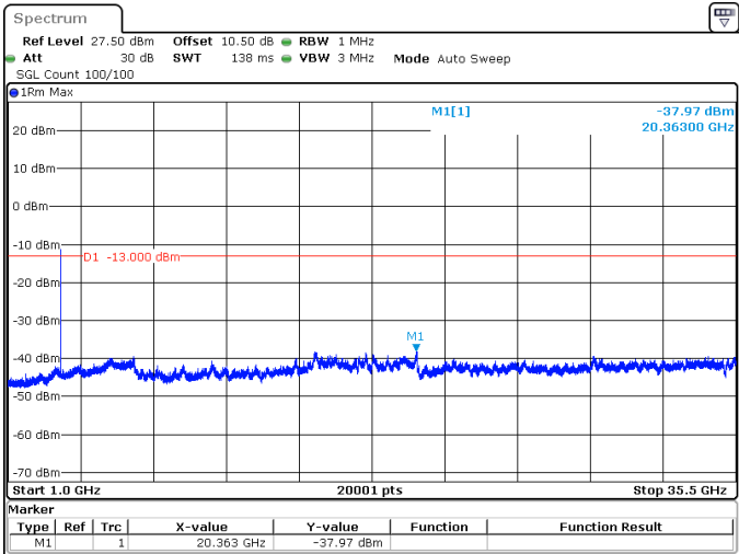
15MHz_15kHz_3500MHz_DFT-s-OFDM QPSK_RB1@0 -37.97 dBm
