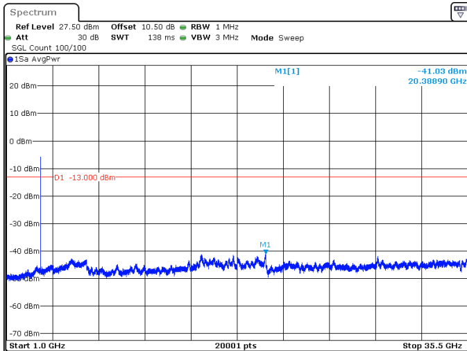
15MHz_15kHz_3542.5MHz_DFT-s-OFDM QPSK_RB1@78 -41.03 dBm
