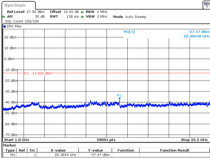
15MHz_15kHz_3457.5MHz_DFT-s-OFDM QPSK_RB1@0 -37.47 dBm
