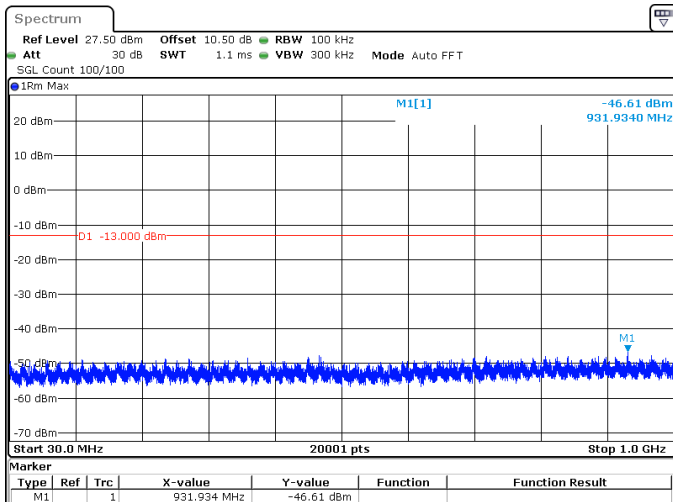
10MHz_30kHz_3545MHz_DFT-s-OFDM QPSK_RB24@0 -46.61 dBm
