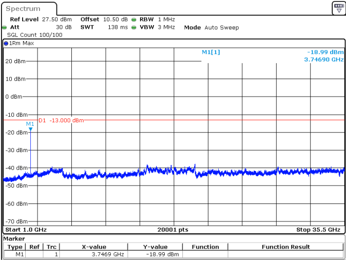
15MHz_15kHz_3500MHz_DFT-s-OFDM QPSK_RB75@0 -18.99 dBm
