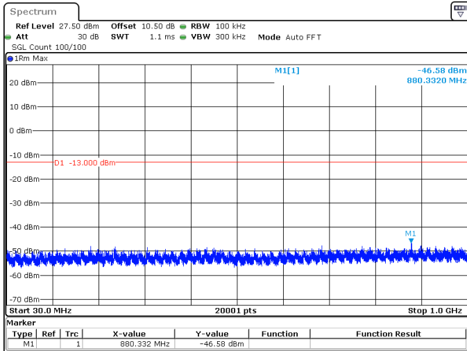
30MHz_15kHz_3500MHz_DFT-s-OFDM QPSK_RB1@0 -46.58 dBm
