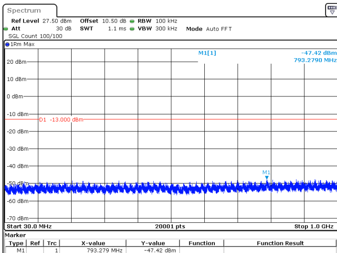
30MHz_15kHz_3465MHz_DFT-s-OFDM QPSK_RB160@0 -47.42 dBm
