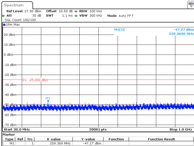
15MHz_15kHz_2562.5MHz_DFT-s-OFDM QPSK_RB1@78 -47.27 dBm
