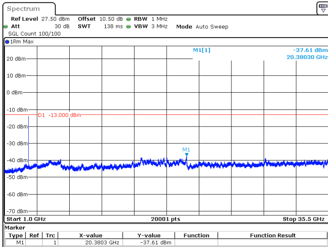
20MHz_30kHz_3540MHz_DFT-s-OFDM QPSK_RB1@50 -37.61 dBm
