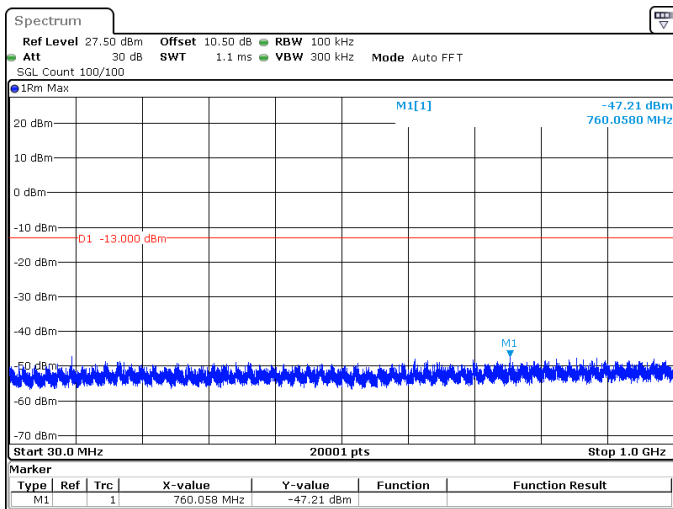
30MHz_15kHz_3535MHz_DFT-s-OFDM QPSK_RB1@159 -47.21 dBm
