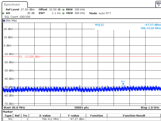
15MHz_30kHz_3457.5MHz_DFT-s-OFDM QPSK_RB1@0 -47.27 dBm
