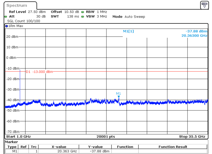
30MHz_15kHz_3500MHz_DFT-s-OFDM QPSK_RB1@159 -37.88 dBm
