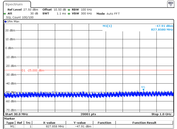
15MHz_15kHz_2535MHz_DFT-s-OFDM QPSK_RB1@0 -47.91 dBm
