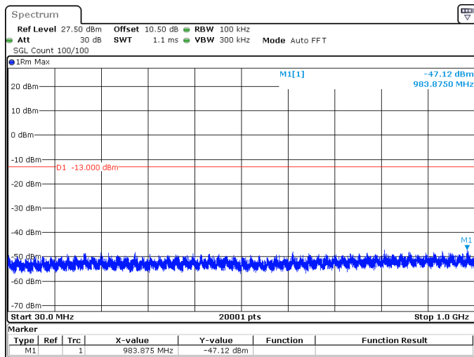
50MHz_15kHz_3475MHz_DFT-s-OFDM QPSK_RB1@269 -47.12 dBm
