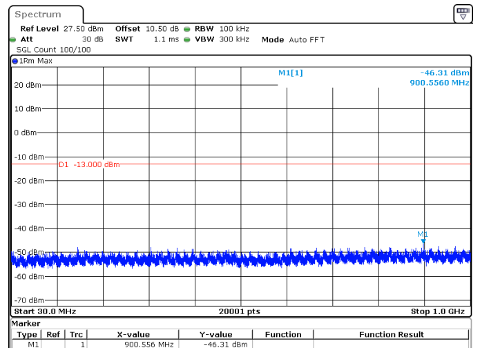
15MHz_15kHz_3457.5MHz_DFT-s-OFDM QPSK_RB75@0 -46.31 dBm
