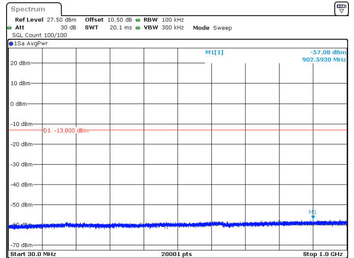
15MHz_15kHz_3542.5MHz_DFT-s-OFDM QPSK_RB1@78 -57.08 dBm
