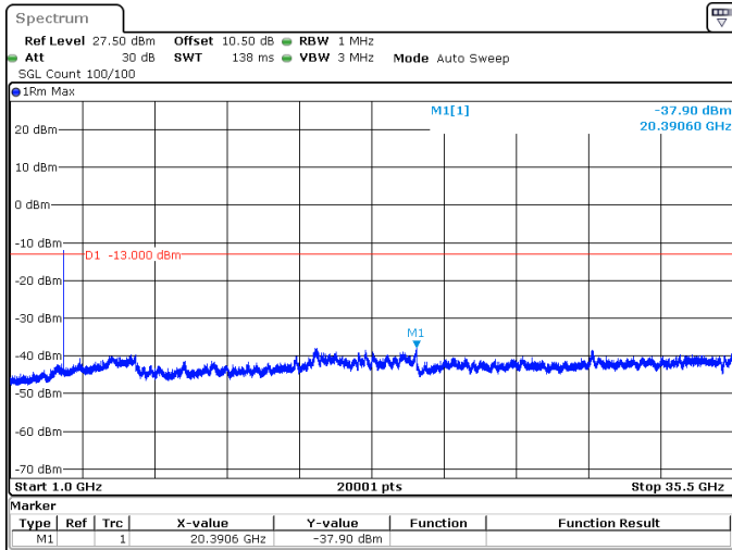
10MHz_30kHz_3545MHz_DFT-s-OFDM QPSK_RB1@0 -37.90 dBm
