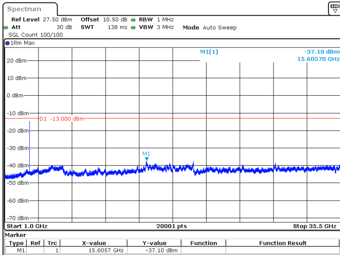
15MHz_30kHz_3542.5MHz_DFT-s-OFDM QPSK_RB1@37 -37.10 dBm
