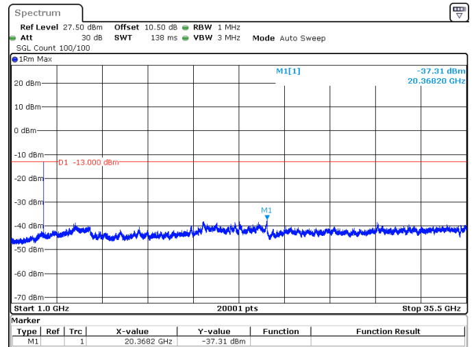
15MHz_30kHz_3457.5MHz_DFT-s-OFDM QPSK_RB1@0 -37.31 dBm
