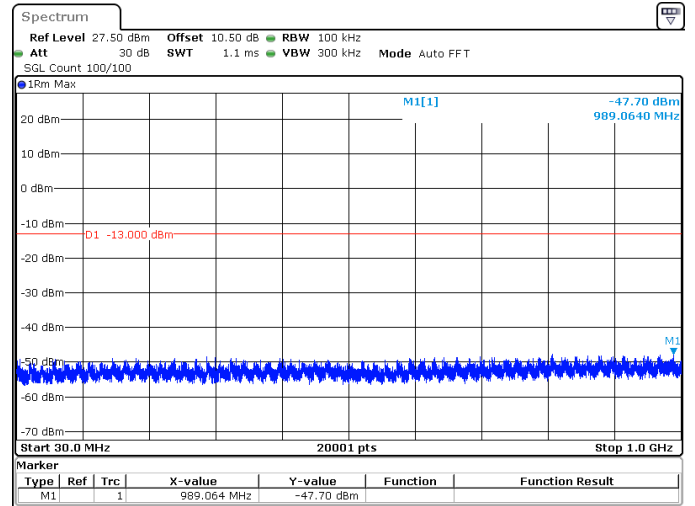
15MHz_15kHz_3457.5MHz_DFT-s-OFDM QPSK_RB1@0 -47.70 dBm
