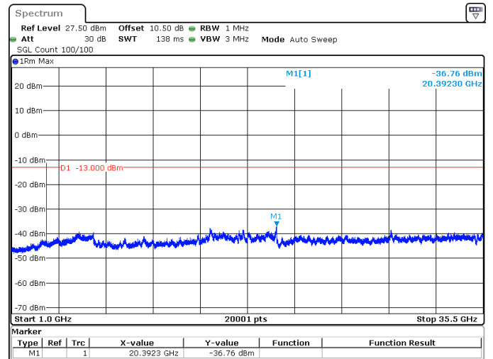
10MHz_15kHz_3545MHz_DFT-s-OFDM QPSK_RB1@0 -36.76 dBm
