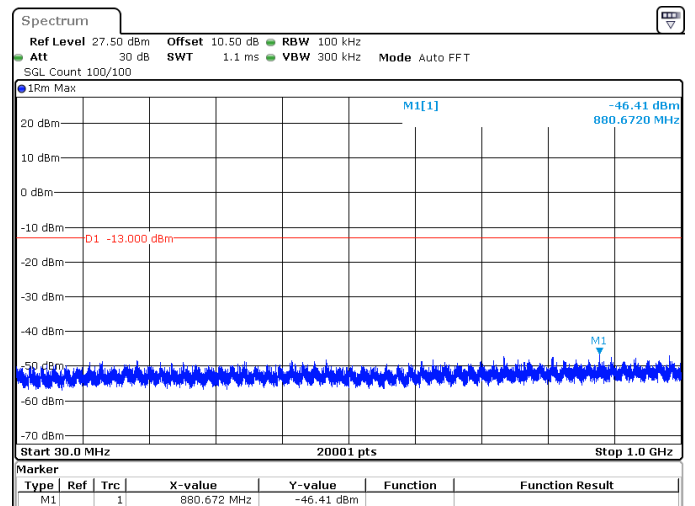
15MHz_30kHz_3457.5MHz_DFT-s-OFDM QPSK_RB1@37 -46.41 dBm
