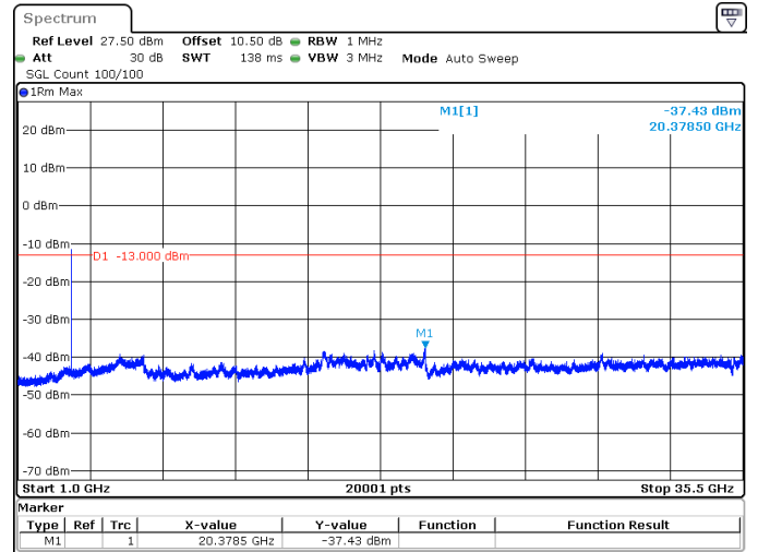
15MHz_30kHz_3542.5MHz_DFT-s-OFDM QPSK_RB1@0 -37.43 dBm
