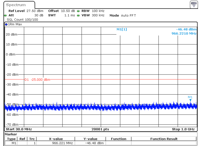
15MHz_15kHz_2507.5MHz_DFT-s-OFDM QPSK_RB1@0 -46.48 dBm
