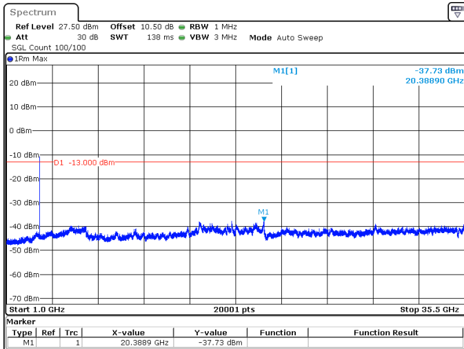
30MHz_15kHz_3465MHz_DFT-s-OFDM QPSK_RB1@159 -37.73 dBm
