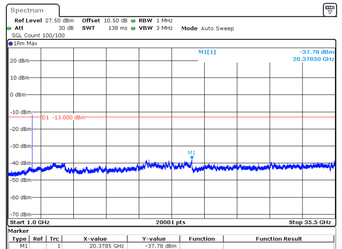
10MHz_15kHz_3545MHz_DFT-s-OFDM QPSK_RB1@51 -37.78 dBm
