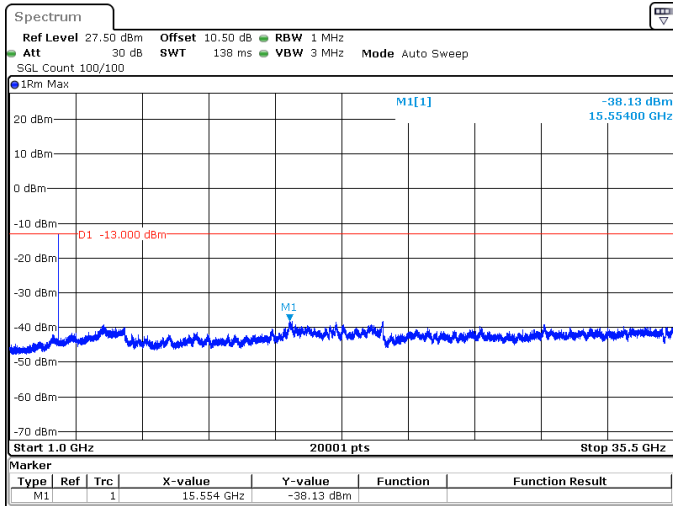
15MHz_15kHz_3542.5MHz_DFT-s-OFDM QPSK_RB1@0 -38.13 dBm
