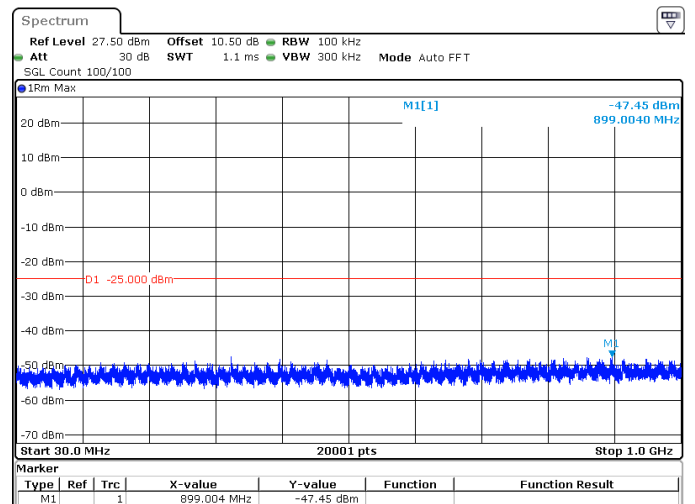
15MHz_15kHz_2507.5MHz_DFT-s-OFDM QPSK_RB75@0 -47.45 dBm
