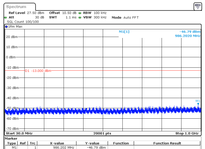
50MHz_15kHz_3475MHz_DFT-s-OFDM QPSK_RB270@0 -46.79 dBm
