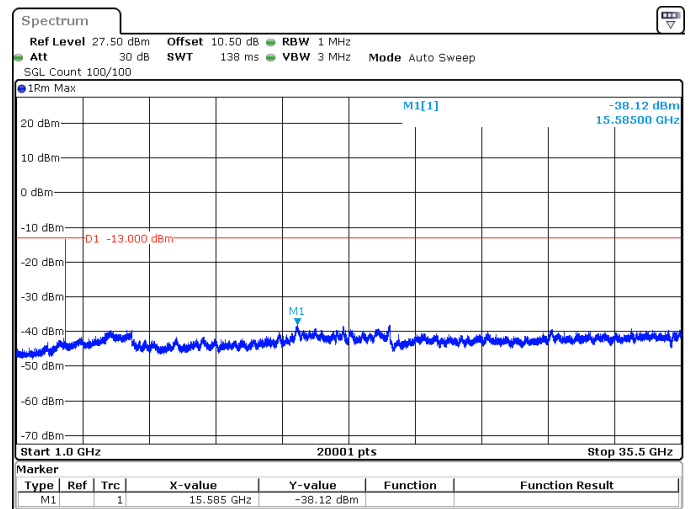
30MHz_15kHz_3535MHz_DFT-s-OFDM QPSK_RB1@159 -38.12 dBm
