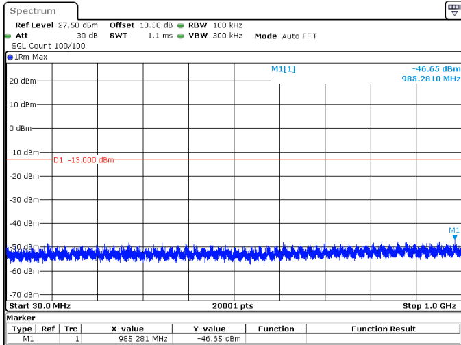
10MHz_30kHz_3545MHz_DFT-s-OFDM QPSK_RB1@23 -46.65 dBm
