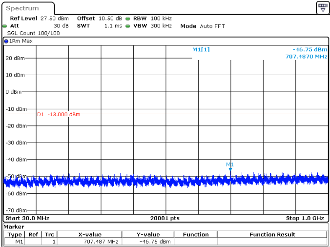
15MHz_15kHz_3707.5MHz_DFT-s-OFDM QPSK_RB75@0 -46.75 dBm
