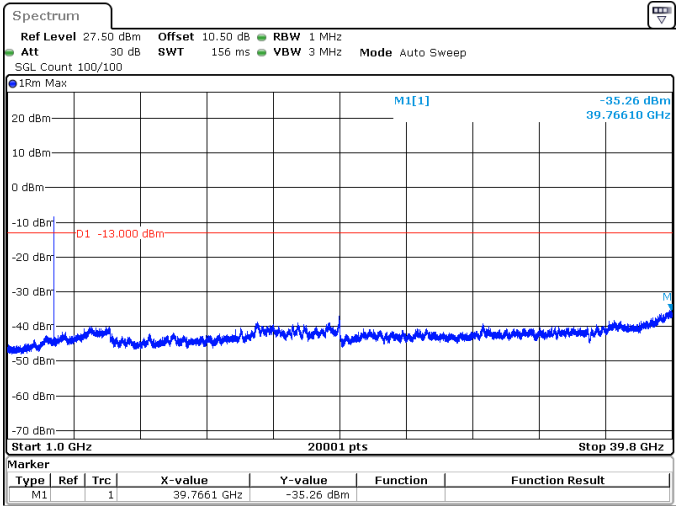
15MHz_15kHz_3707.5MHz_DFT-s-OFDM QPSK_RB1@78 -35.26 dBm
