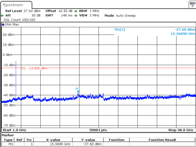
10MHz_15kHz_3705MHz_DFT-s-OFDM QPSK_RB1@51 -37.60 dBm
