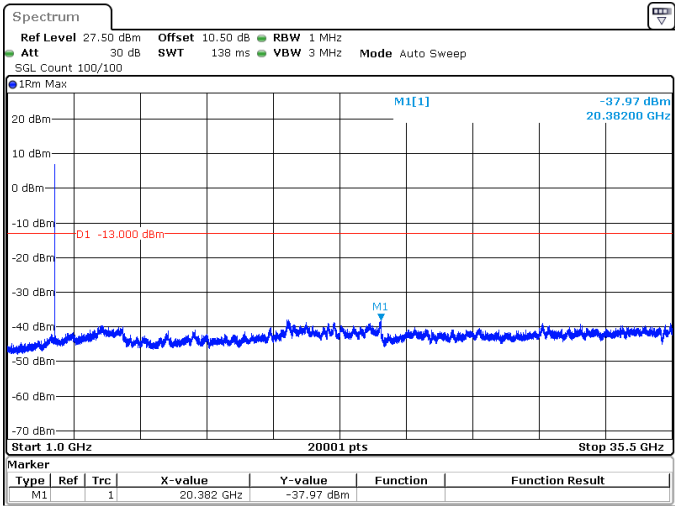
25MHz_30kHz_3462.5MHz_DFT-s-OFDM QPSK_RB1@0 -37.97 dBm
