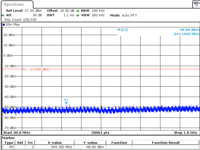
30MHz_30kHz_3535MHz_DFT-s-OFDM QPSK_RB1@77 -46.66 dBm
