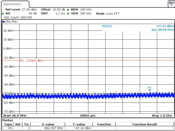
50MHz_30kHz_3475MHz_DFT-s-OFDM QPSK_RB128@0 -47.34 dBm
