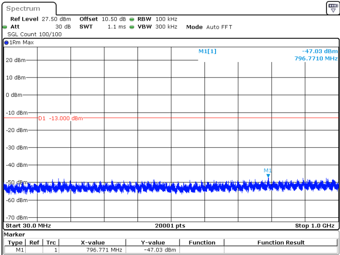
15MHz_30kHz_3542.5MHz_DFT-s-OFDM QPSK_RB1@37 -47.03 dBm
