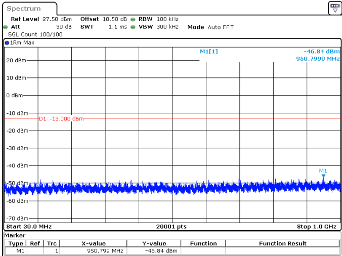
50MHz_30kHz_3475MHz_DFT-s-OFDM QPSK_RB1@132 -46.84 dBm
