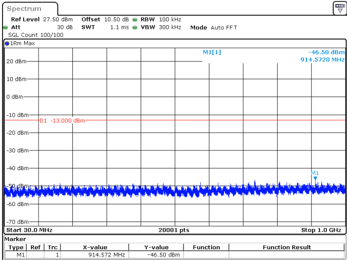
50MHz_30kHz_3500MHz_DFT-s-OFDM QPSK_RB1@132 -46.50 dBm
