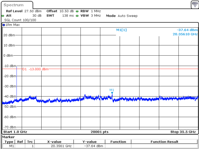
100MHz_30kHz_3500MHz_DFT-s-OFDM QPSK_RB1@272 -37.64 dBm
