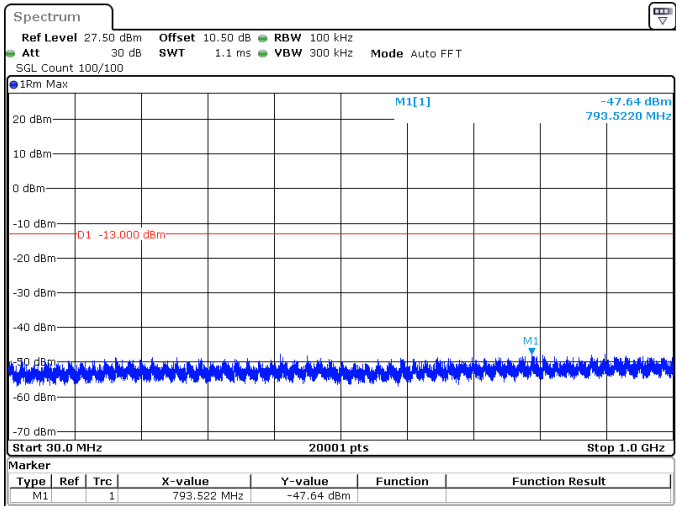
70MHz_30kHz_3515MHz_DFT-s-OFDM QPSK_RB1@188 -47.64 dBm
