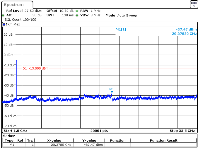
50MHz_30kHz_3500MHz_DFT-s-OFDM QPSK_RB128@0 -37.47 dBm
