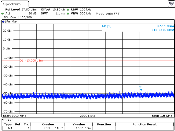
15MHz_30kHz_3542.5MHz_DFT-s-OFDM QPSK_RB36@0 -47.11 dBm
