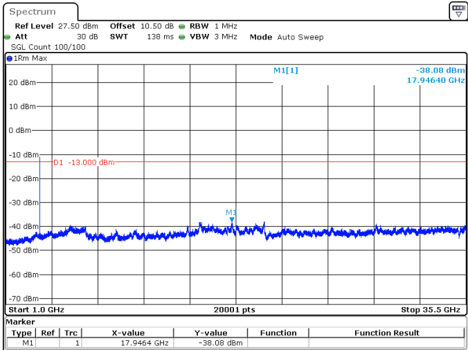
80MHz_30kHz_3500MHz_DFT-s-OFDM QPSK_RB1@216 -38.08 dBm
