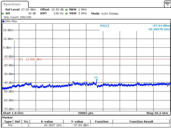
50MHz_30kHz_3500MHz_DFT-s-OFDM QPSK_RB1@0 -37.94 dBm
