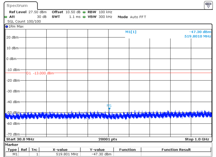
30MHz_15kHz_3750MHz_DFT-s-OFDM QPSK_RB160@0 -47.30 dBm
