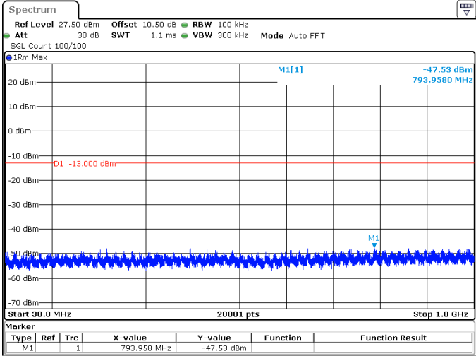
30MHz_15kHz_3715MHz_DFT-s-OFDM QPSK_RB160@0 -47.53 dBm
