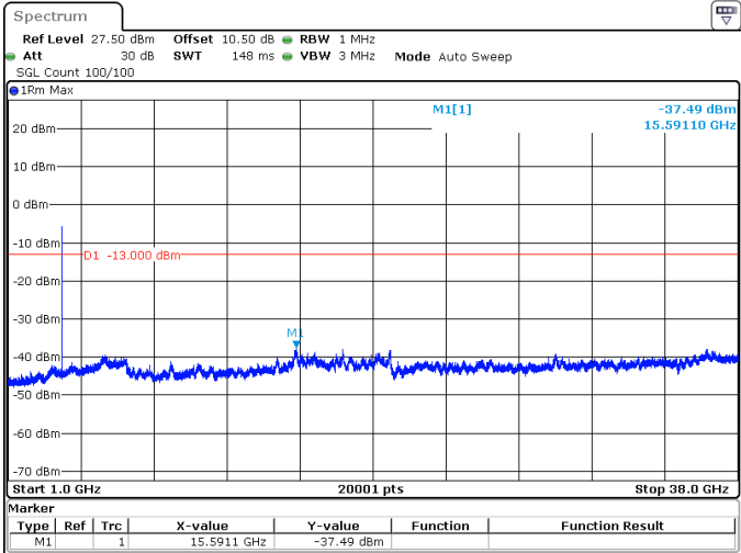
30MHz_15kHz_3715MHz_DFT-s-OFDM QPSK_RB1@159 -37.49 dBm
