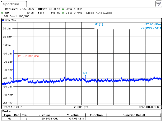
40MHz_30kHz_3720MHz_DFT-s-OFDM QPSK_RB1@105 -37.63 dBm
