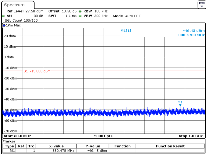
60MHz_30kHz_3730MHz_DFT-s-OFDM QPSK_RB162@0 -46.45 dBm
