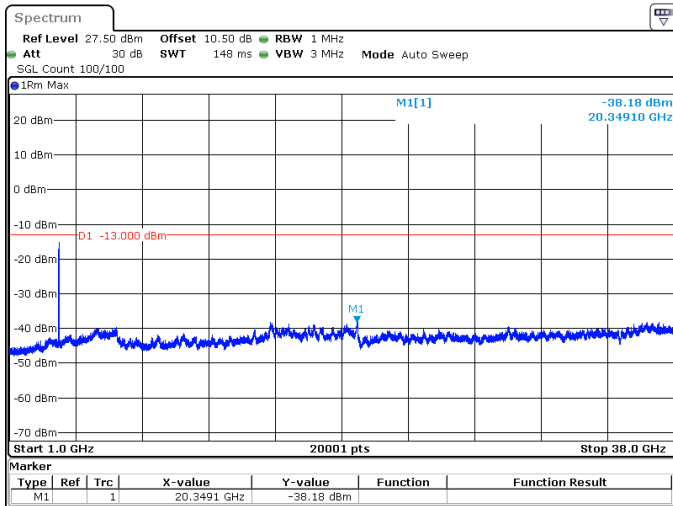
30MHz_15kHz_3750MHz_DFT-s-OFDM QPSK_RB160@0 -38.18 dBm
