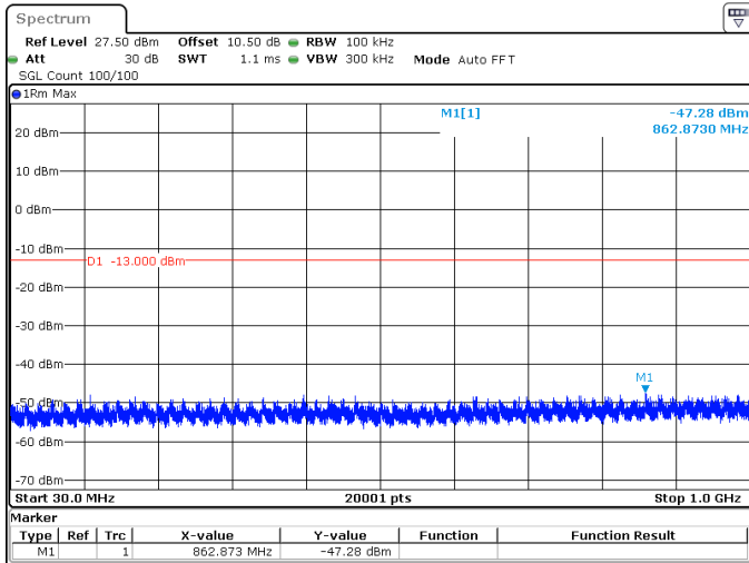
30MHz_15kHz_3750MHz_DFT-s-OFDM QPSK_RB1@159 -47.28 dBm
