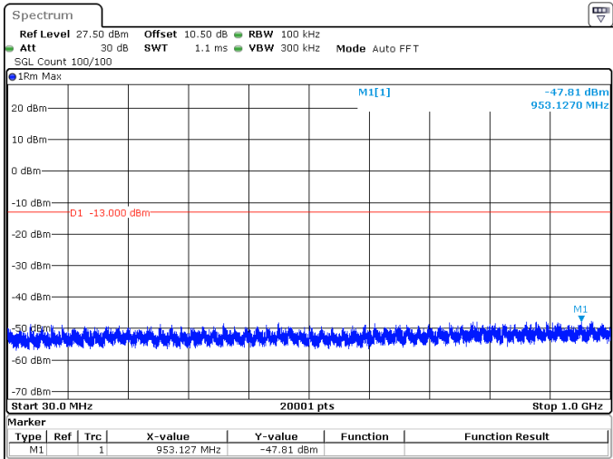
60MHz_30kHz_3730MHz_DFT-s-OFDM QPSK_RB1@161 -47.81 dBm
