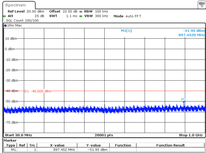
40MHz_30kHz_3680MHz_DFT-s-OFDM QPSK_RB100@0 -51.95 dBm
