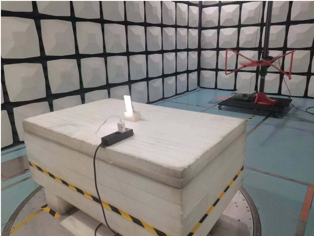
Radiated Emission 30M-1GHz front View
