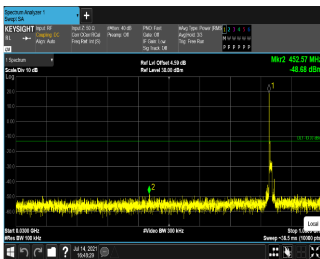
Band5-10MHz-QPSK-20600:30~1000MHz
