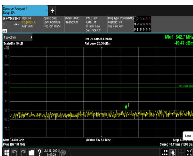
Band38-5MHz-16QAM-38225:30~1000MHz
