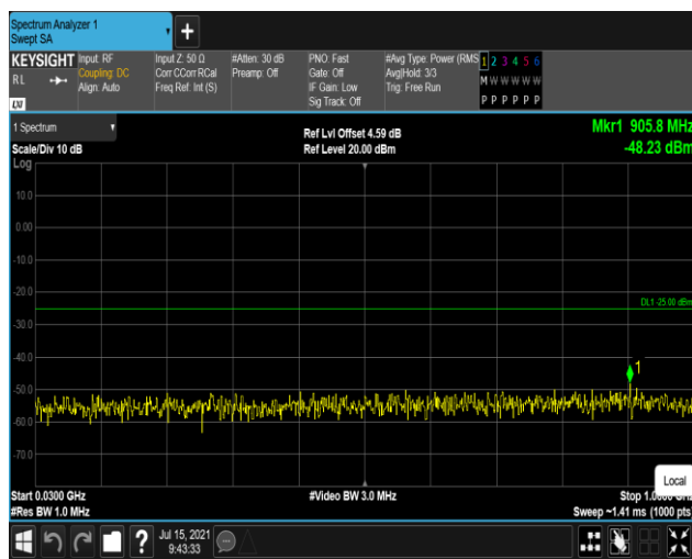
Band38-5MHz-16QAM-38000:30~1000MHz
