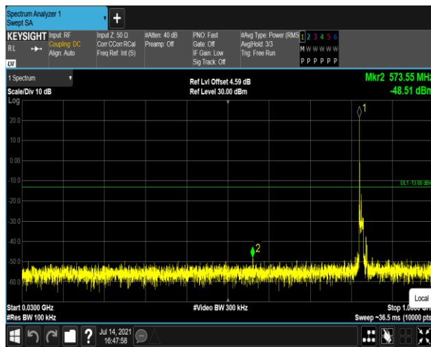
Band5-10MHz-16QAM-20525:30~1000MHz
