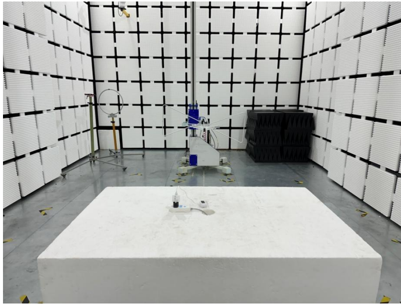
RADIATED EMISSION TEST BELOW 1GHz
