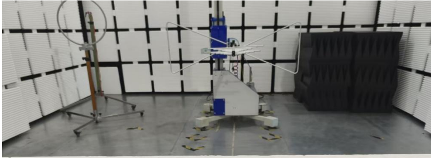
RADIATED EMISSION TEST BELOW 1GHz
