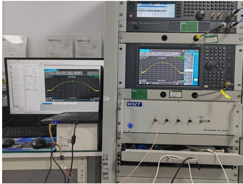
RF test photo
