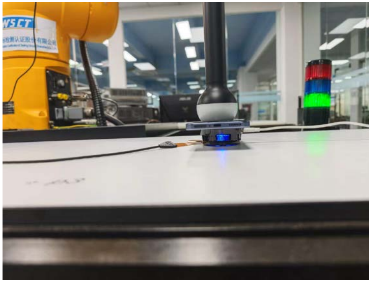
XG03Pro WPT Test setup photos
