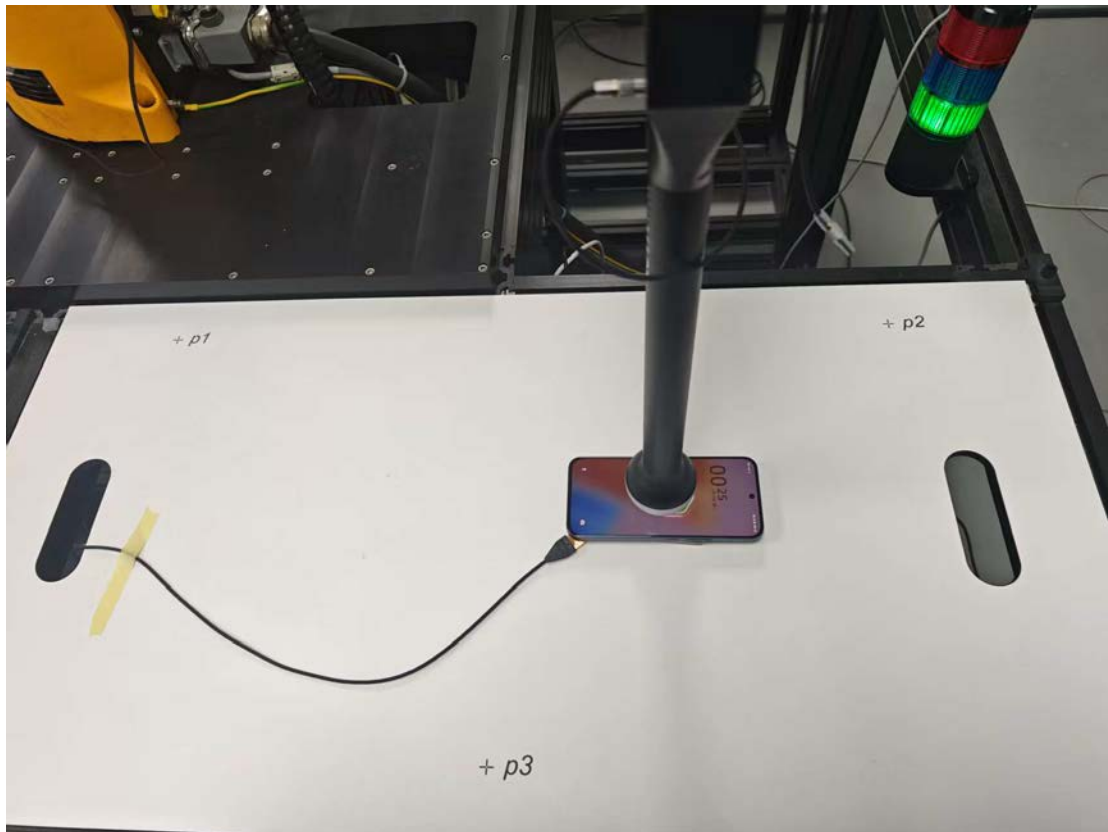
XP06 WPT Test setup photos
