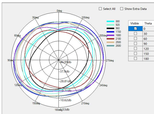
GSM 900/DCS/ WCDMA B4/B8/ LTE B3/B4/B7/B8/B38/B41/B66 Phi=0deg
