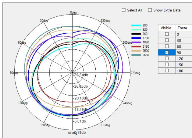
GSM 900/DCS/ WCDMA B4/B8/ LTE B3/B4/B7/B8/B38/B41/B66 Theta=90deg
