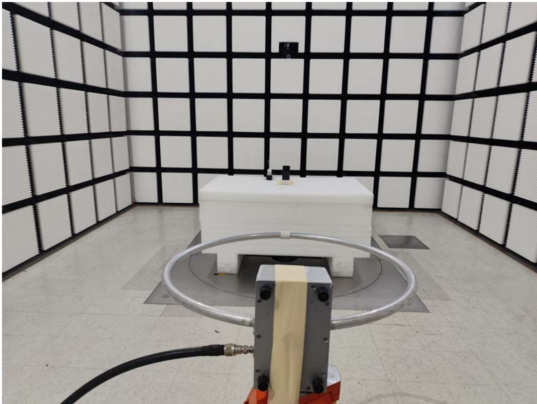
Radiated Emission 9kHz-30MHz View-Ground-parallel
