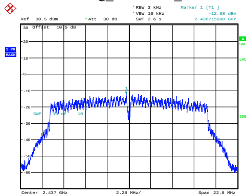
802.11g_2437MHz_Chain 0
