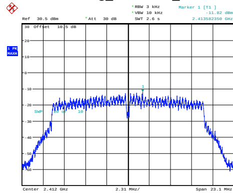
802.11g_2412MHz_Chain 0
