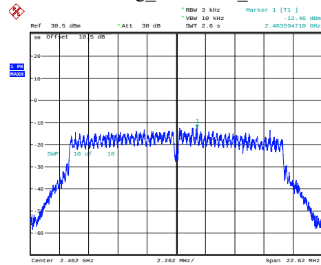
802.11g_2462MHz_Chain 0
