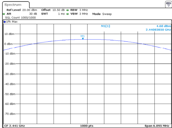
3DH1_Middle 4.60dBm
