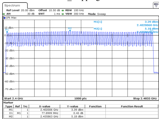
DH1_Hopping 79
