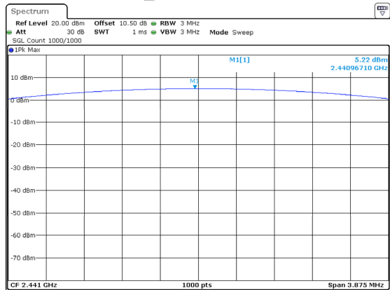
DH1_Middle 5.22dBm
