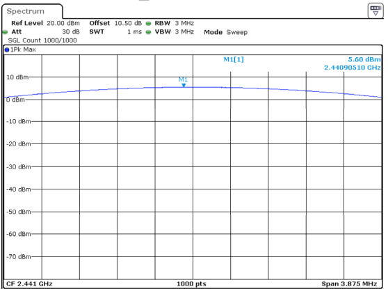
DH1_Middle 5.60dBm
