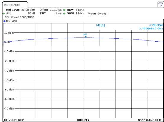
DH1_Low 4.70dBm
