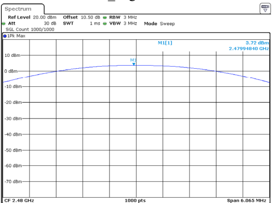
2DH1_High 3.72dBm
