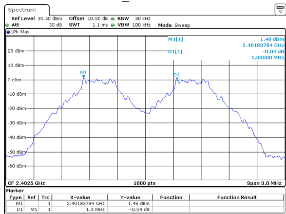
DH1_Low 1MHz
