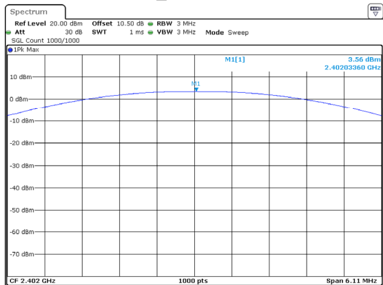
3DH1_Low 3.56dBm
