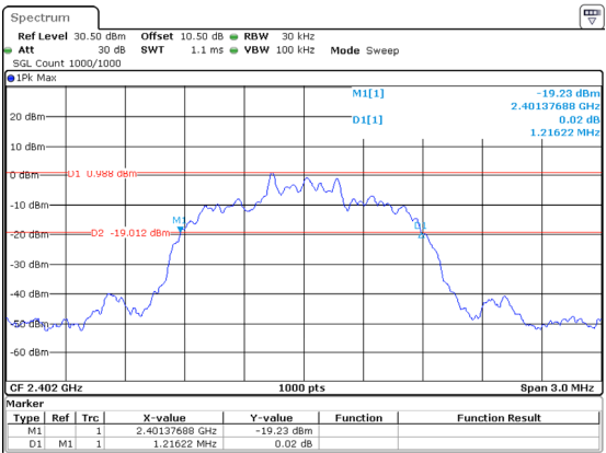
2DH1_Low 1.216MHz
