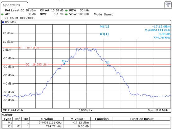
DH1_Middle 0.775MHz
