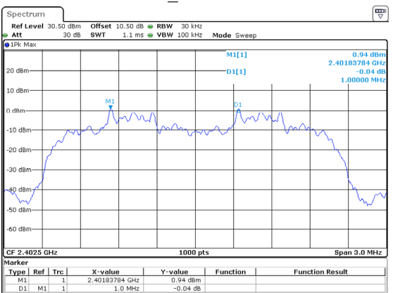
2DH1_Low 1MHz
