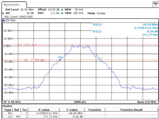
DH1_High 0.772MHz
