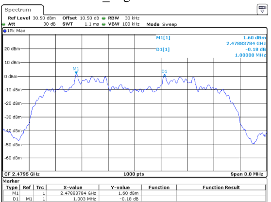
2DH1_High 1.003MHz
