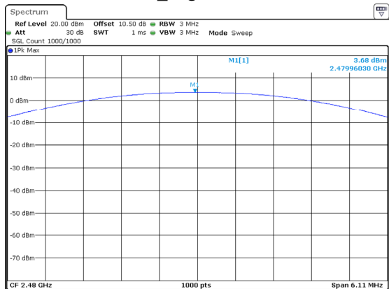
3DH1_High 3.68dBm
