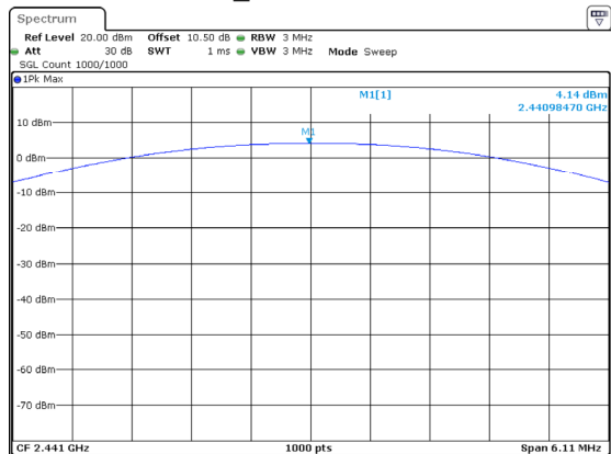
3DH1_Middle 4.14dBm
