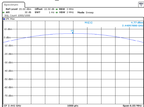
2DH1_Middle 4.77dBm
