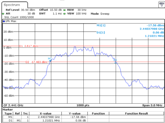
2DH1_Middle 1.210MHz
