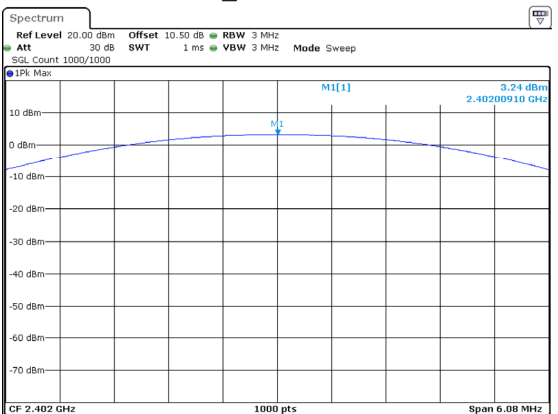
2DH1_Low 3.24dBm
