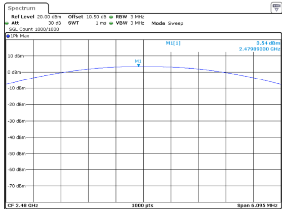
3DH1_High 3.54dBm
