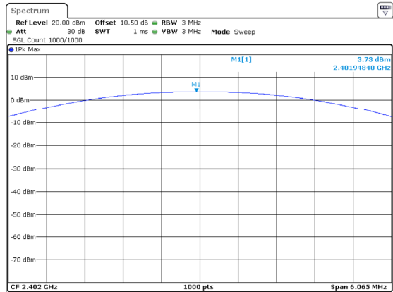
2DH1_Low 3.73dBm
