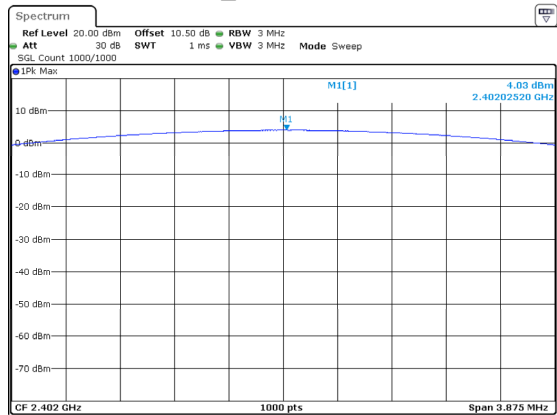
DH1_Low 4.03dBm
