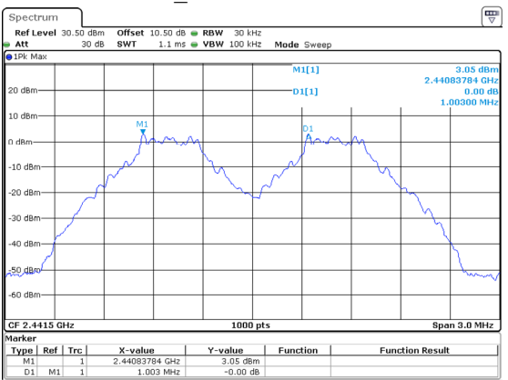
DH1_Middle 1.003MHz
