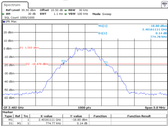
DH1_Low 0.775MHz
