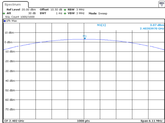
3DH1_Low 3.07dBm
