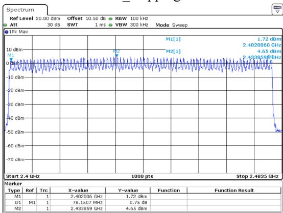
2DH1_Hopping 79
