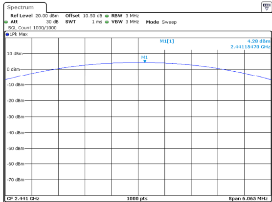
2DH1_Middle 4.28dBm
