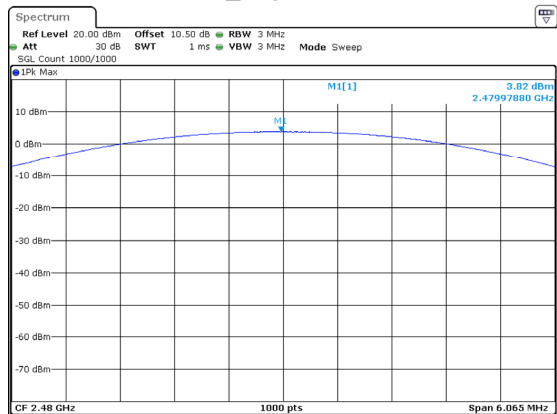
2DH1_High 3.82dBm
