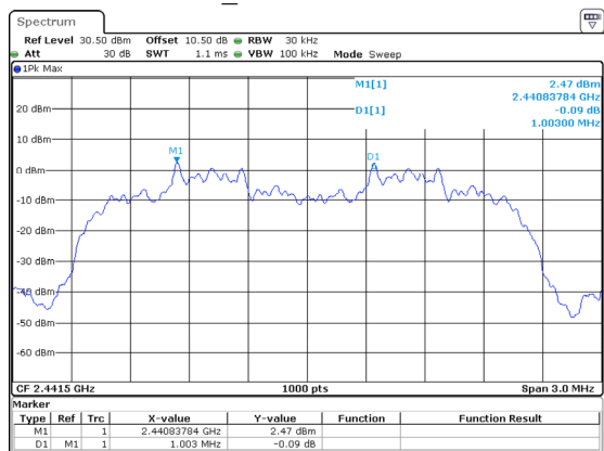
2DH1_Middle 1.003MHz
