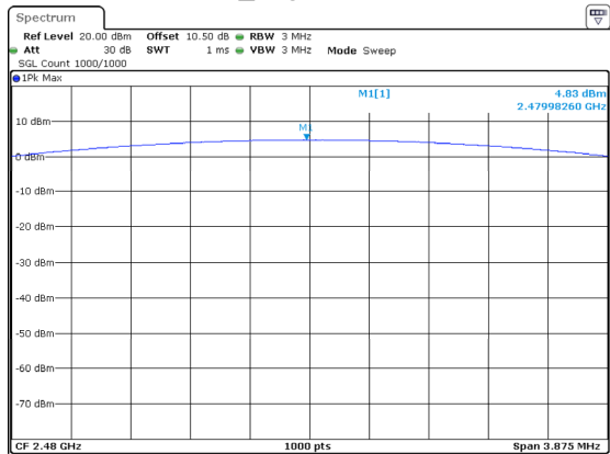
DH1_High 4.83dBm
