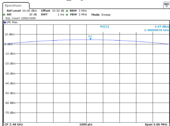
DH1_High 4.57dBm
