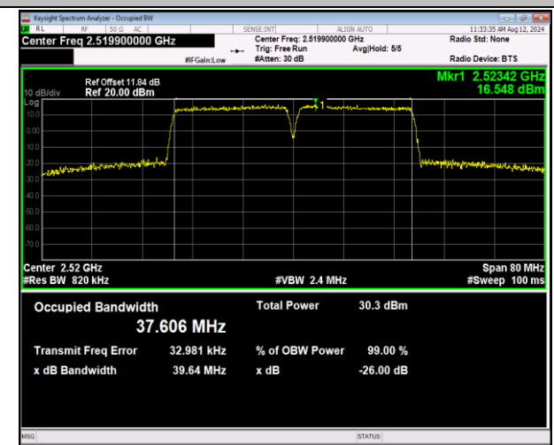
7-7-20MHz-20MHz-QPSK-QPSK-20850-21048-100RB#0-100RB#0-PASS
