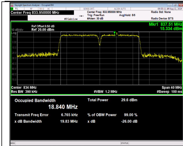
5-5-10MHz-10MHz-QPSK-QPSK-20450-20549-50RB#0-5 ORB#0-PASS
