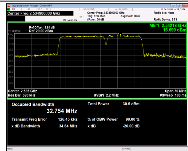
7-7-20MHz-15MHz-64QAM-64QAM-21026-21197-100RB#0-75RB#0-PASS
