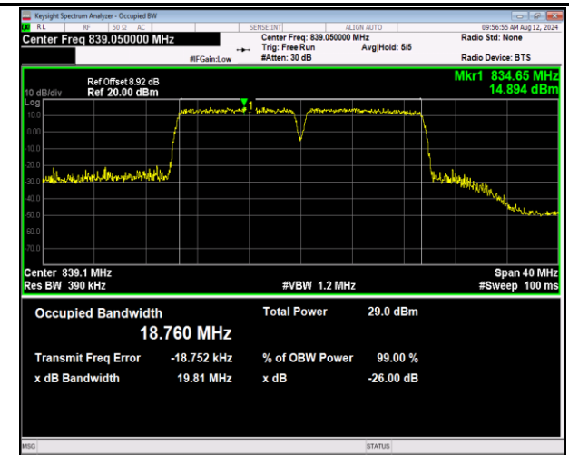
5-5-10MHz-10MHz-16QAM-16QAM-20501-20600-50RB#0-50RB#0-PASS
