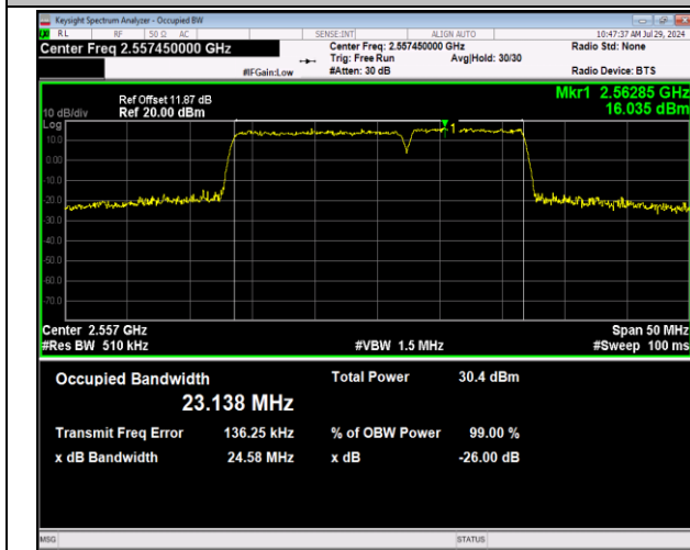
7-7-15MHz-10MHz-64QAM-64QAM-21277-21397-75RB#0-5 -50RB#0-PASS
