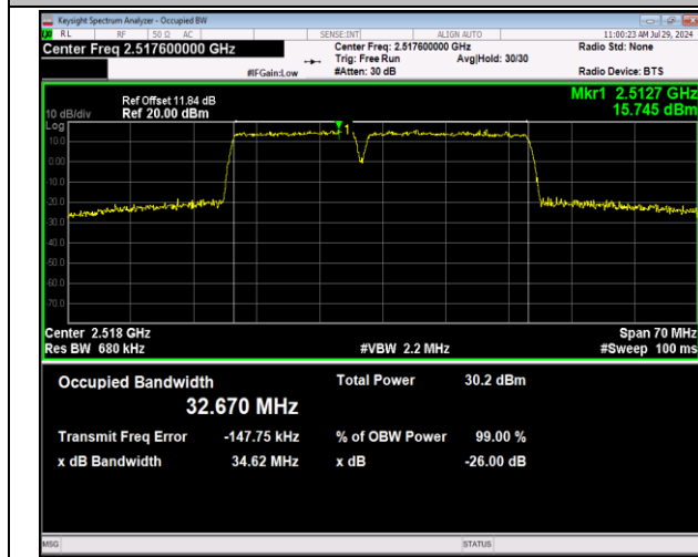
7-7-15MHz-20MHz-64QAM-64QAM-20828-20999-75RB#0-1 -100RB#0-PASS
