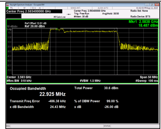
41-41-5MHz-20MHz-QPSK-QPSK-40528-40645-25RB#0-100RB#0-PASS
