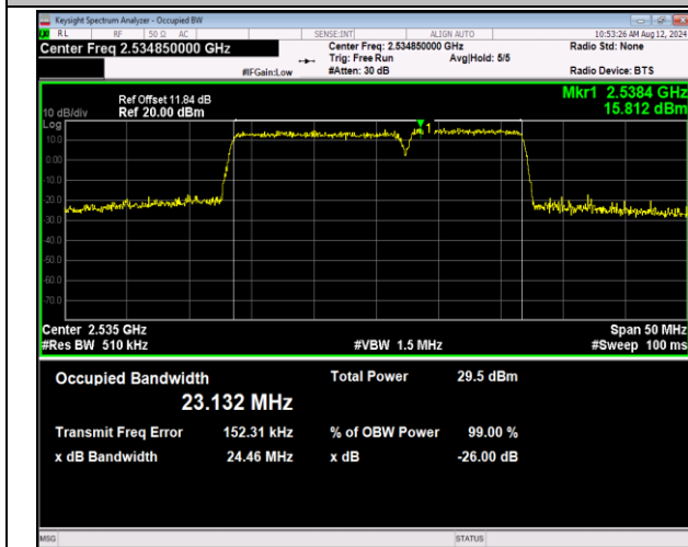
7-7-15MHz-10MHz-16QAM-16QAM-21051-21171-75RB#0-50RB#0-PASS
