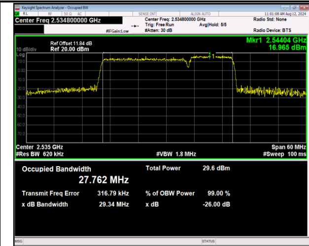
7-7-20MHz-10MHz-16QAM-16QAM-21051-21195-100RB#0-50RB#0-PASS
