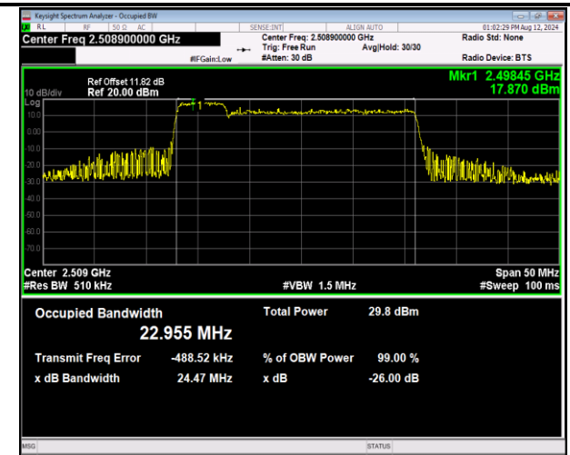
41-41-5MHz-20MHz-16QAM-16QAM-39683-39800-25RB#0-100RB#0-PASS
