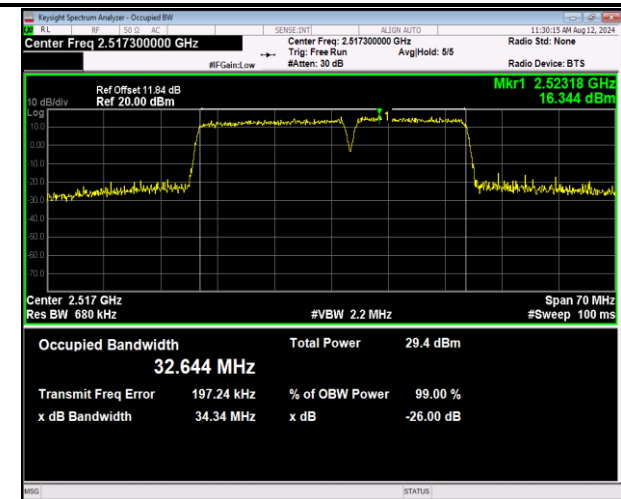
7-7-20MHz-15MHz-16QAM-16QAM-20850-21021-100RB#0-75RB#0-PASS
