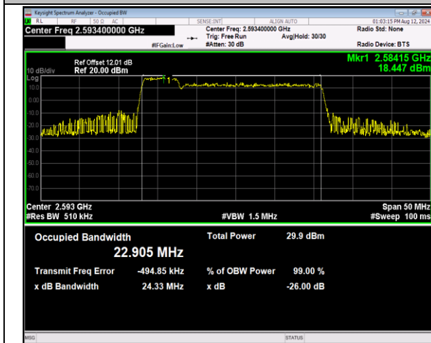
41-41-5MHz-20MHz-16QAM-16QAM-40528-40645-25RB#0-100RB#0-PASS
