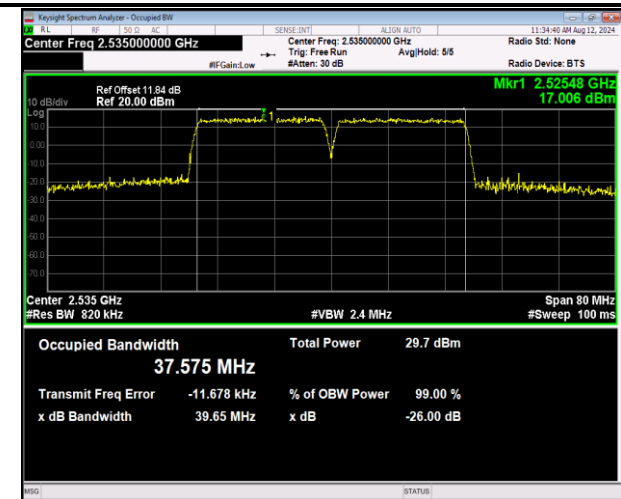
7-7-20MHz-20MHz-16QAM-16QAM-21001-21199-100RB#0-100RB#0-PASS
