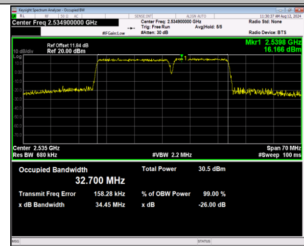
7-7-20MHz-15MHz-QPSK-QPSK-21026-21197-100RB#0-75RB#0-PASS
