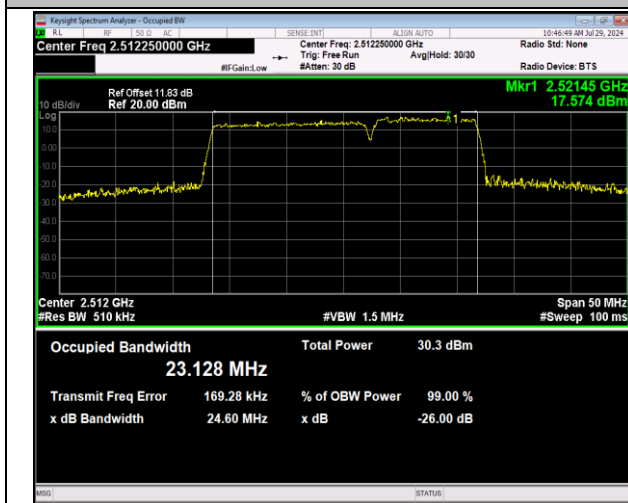
7-7-15MHz-10MHz-64QAM-64QAM-20825-20945-75RB#0-50RB#0-PASS
