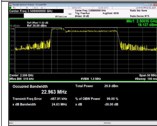
41-41-5MHz-20MHz-64QAM-64QAM-39683-39800-25RB#0-100RB#0-PASS
