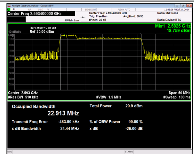
41-41-5MHz-20MHz-64QAM-64QAM-40528-40645-25RB#0-100RB#0-PASS
