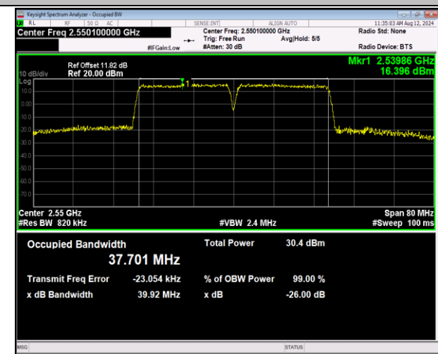
7-7-20MHz-20MHz-QPSK-QPSK-21152-21350-100RB#0-100RB#0-PASS
