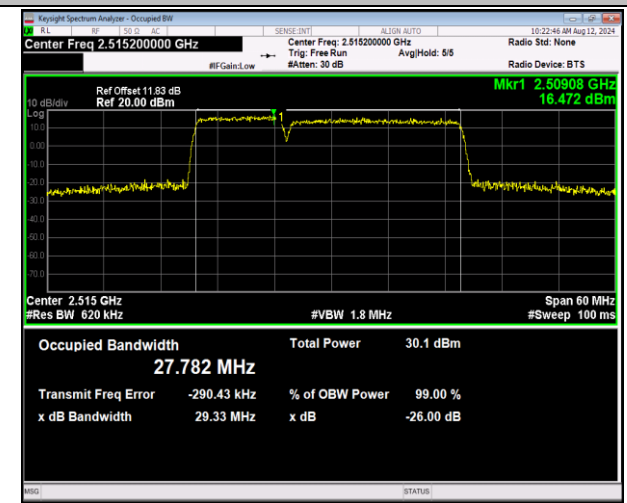
7-7-10MHz-20MHz-QPSK-QPSK-20805-20949-50RB#0-100RB#0-PASS
