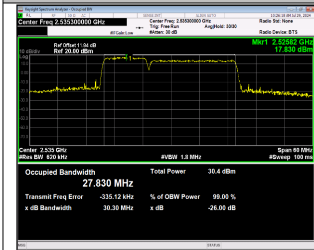
7-7-10MHz-20MHz-64QAM-64QAM-21006-21150-50RB#0 -100RB#0-PASS
