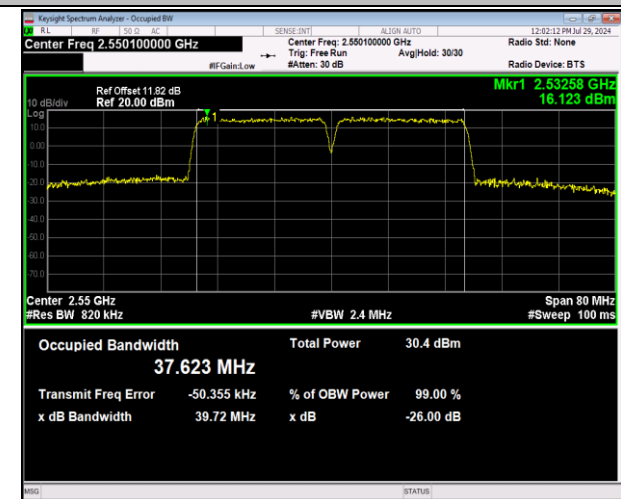
7-7-20MHz-20MHz-64QAM-64QAM-21152-21350-100RB#0-100RB#0-PASS
