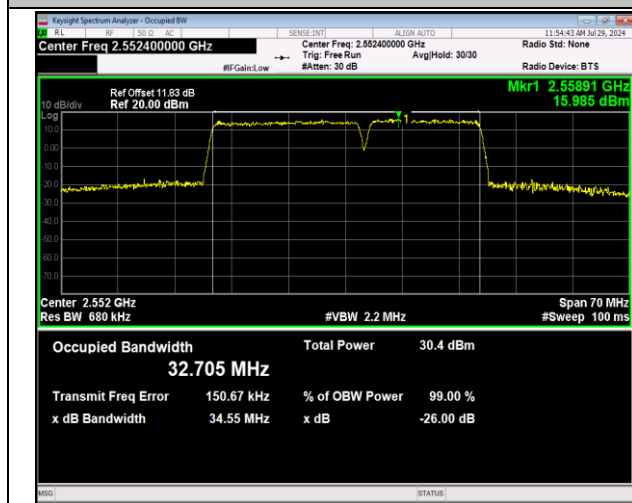
7-7-20MHz-15MHz-64QAM-64QAM-21201-21372-100RB#0-75RB#0-PASS
