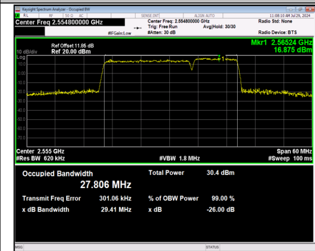
7-7-20MHz-10MHz-64QAM-64QAM-21251-21395-100RB#0-50RB#0-PASS
