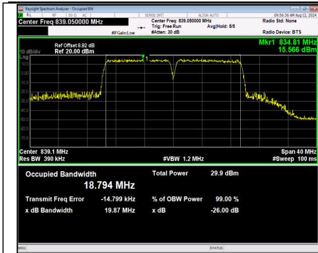
5-5-10MHz-10MHz-QPSK-QPSK-20501-20600-50RB#0-5 ORB#0-PASS
