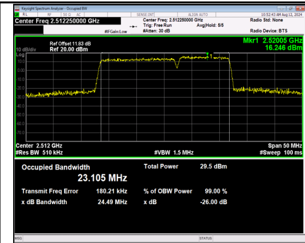
7-7-15MHz-10MHz-16QAM-16QAM-20825-20945-75RB#0-50RB#0-PASS
