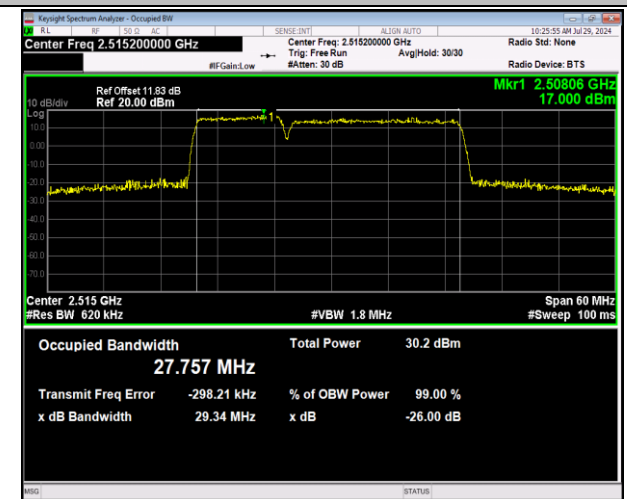
7-7-10MHz-20MHz-64QAM-64QAM-20805-20949-50RB#0-100RB#0-PASS
