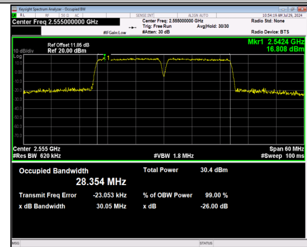
7-7-15MHz-15MHz-64QAM-64QAM-21225-21375-75RB#0-7 -75RB#0-PASS
