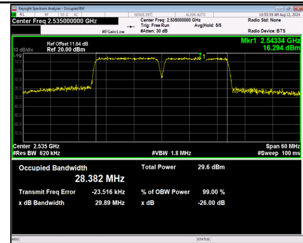
7-7-15MHz-15MHz-16QAM-16QAM-21025-21175-75RB#0-7 -75RB#0-PASS
