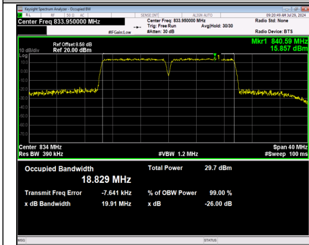
5-5-10MHz-10MHz-64QAM-64QAM-20450-20549-50RB#0-5 -50RB#0-PASS
