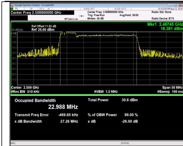
41-41-5MHz-20MHz-QPSK-QPSK-39683-39800-25RB#0-100RB#0-PASS
