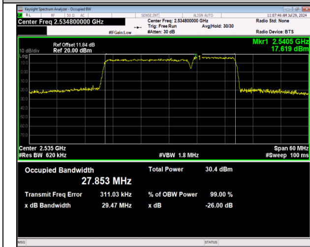
7-7-20MHz-10MHz-64QAM-64QAM-21051-21195-100RB#0-50RB#0-PASS
