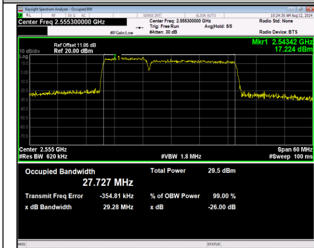
7-7-10MHz-20MHz-16QAM-16QAM-21206-21350-50RB#0 -100RB#0-PASS
