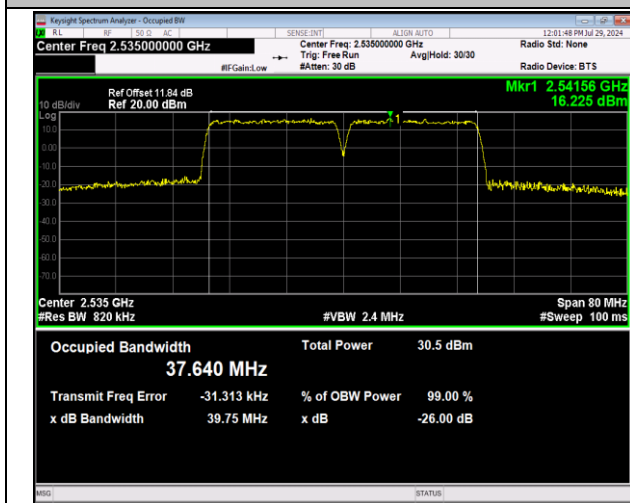
7-7-20MHz-20MHz-64QAM-64QAM-21001-21199-100RB#0-100RB#0-PASS
