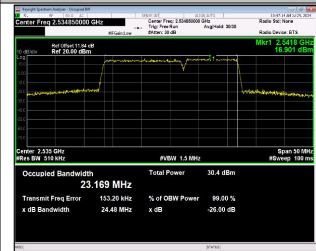
7-7-15MHz-10MHz-64QAM-64QAM-21051-21171-75RB#0-50RB#0-PASS
