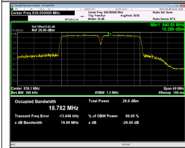
5-5-10MHz-10MHz-64QAM-64QAM-20501-20600-50RB#0-50RB#0-PASS
