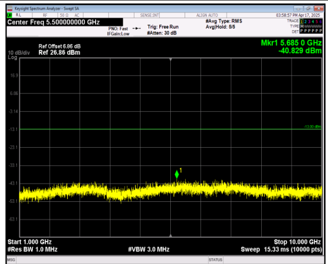
Band13-5MHz-64QAM-23230-1RB#0-Range2:1000~10000MHz
