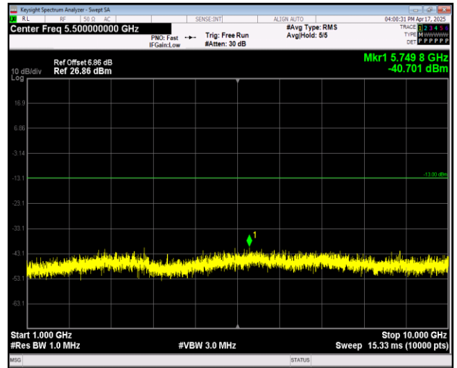
Band13-5MHz-64QAM-23205-1RB#0-Range2:1000~10000MHz
