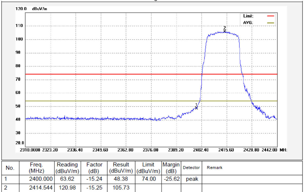
TX 11n HT20: Band edge-left side Horizontal
