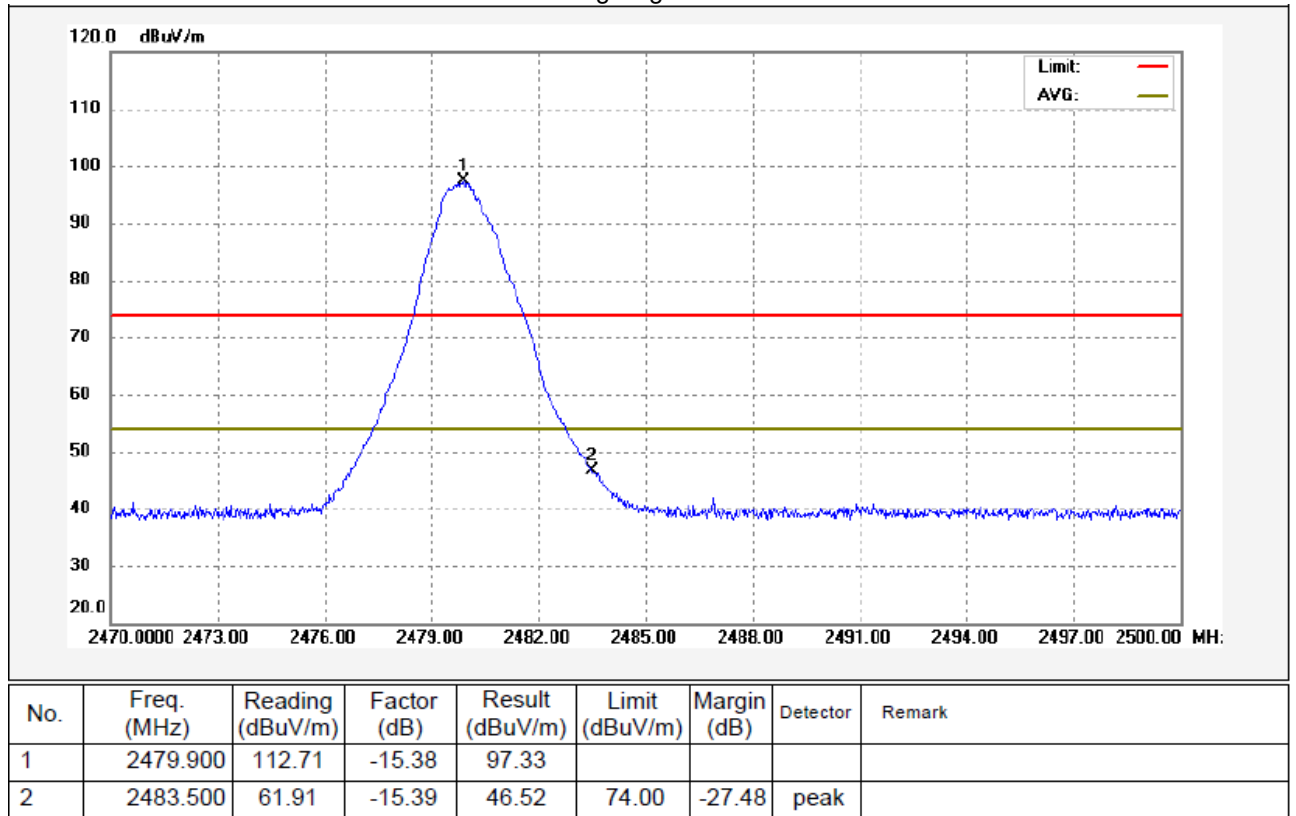
BLE: Band edge-right side Horizontal
