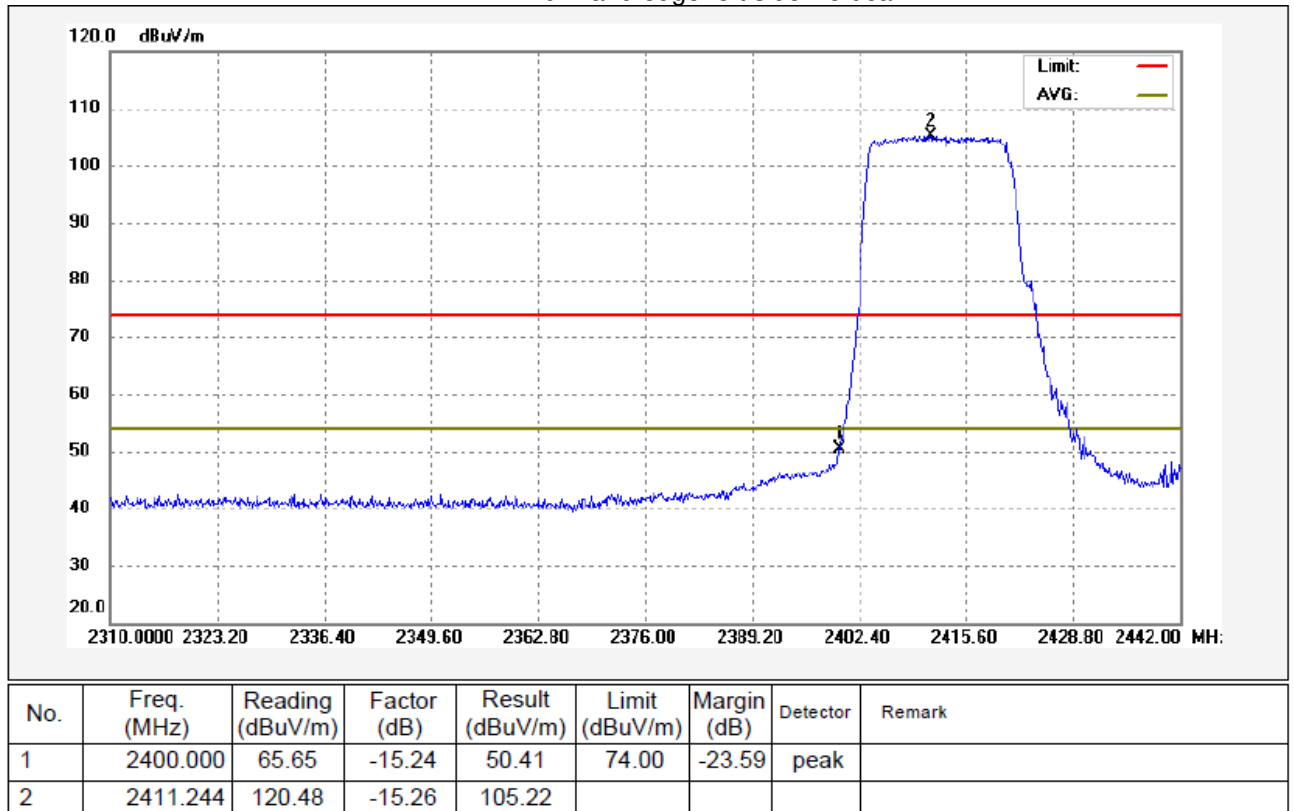
TX 11n HT20: Band edge-left side Vertical
