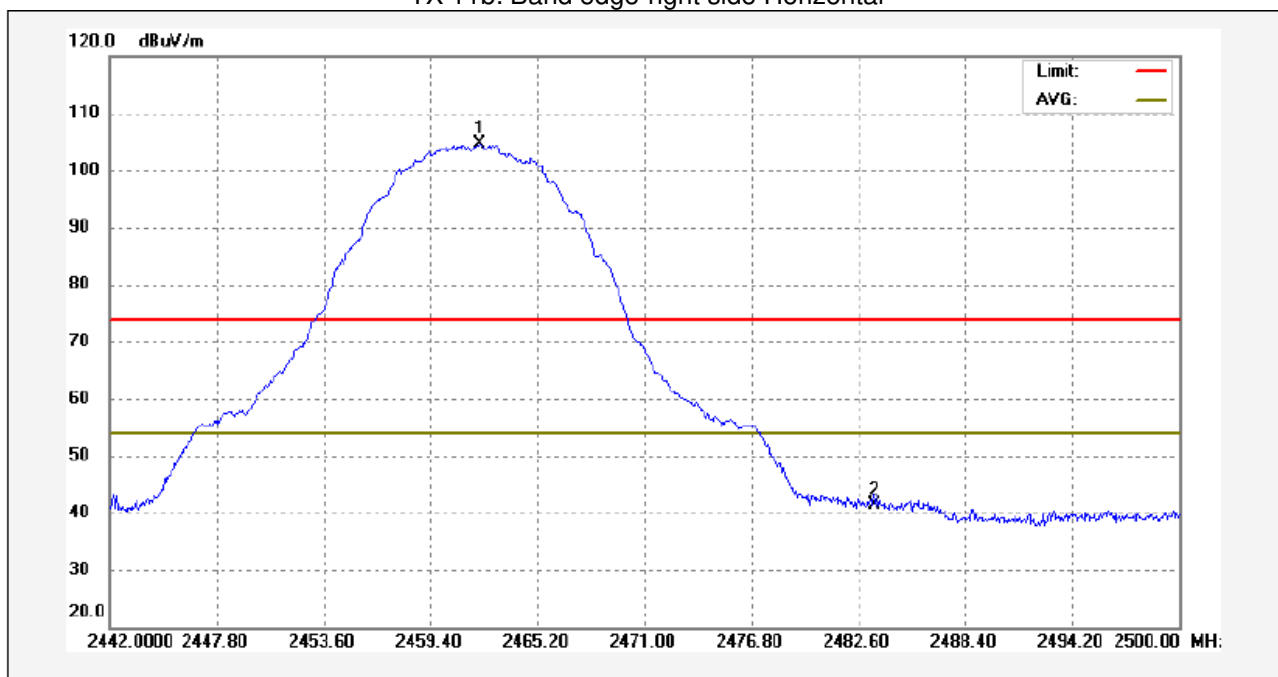
TX 11b: Band edge-right side Horizontal
