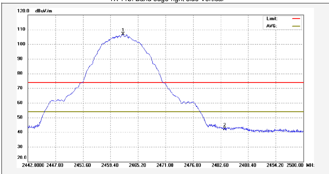
TX 11b: Band edge-right side Vertical
