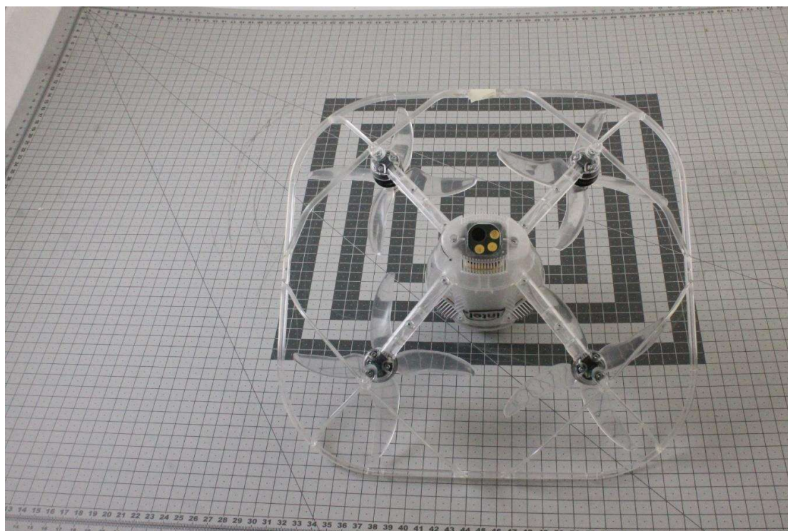
Photograph 2. EUT
