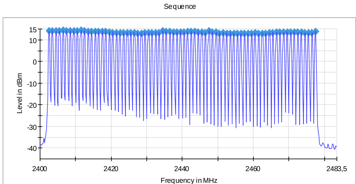
Figure 18: Number of hopping channels, modem1, CW
