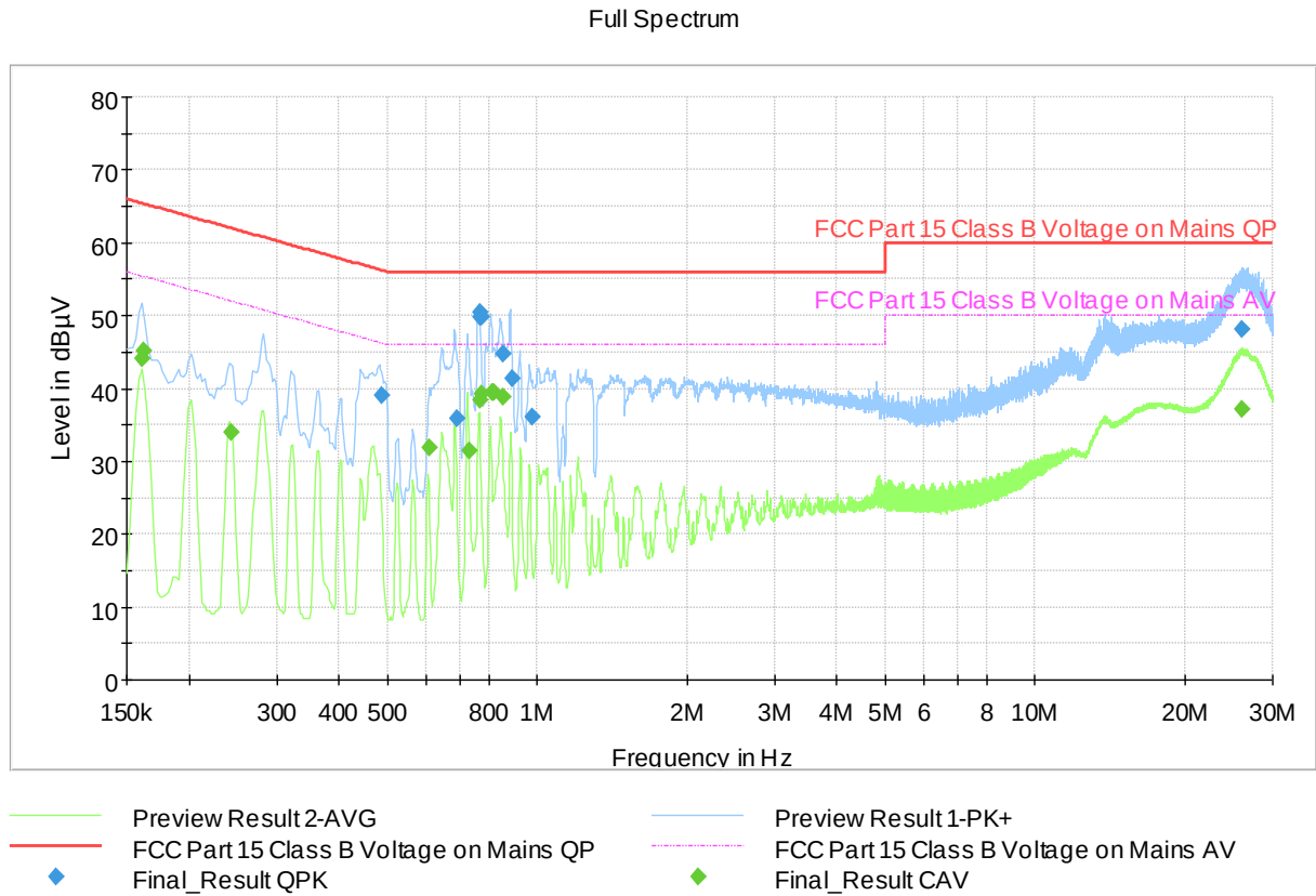
Figure 2. The measured results with peak- and average detectors at the Launch Pad AC power port
