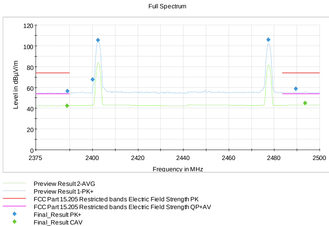
Figure 10: Radiated lower and upper band edge, modem1/ch75 modem2/channel0
