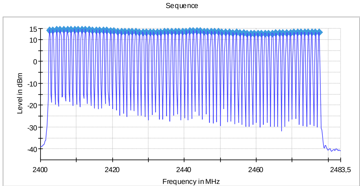
Figure 19: Number of hopping channels, modem2, CW
