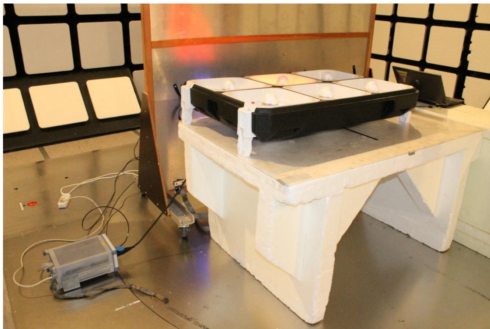
Photograph 7. Conducted emission test set-up (Launch Pad AC-port)
