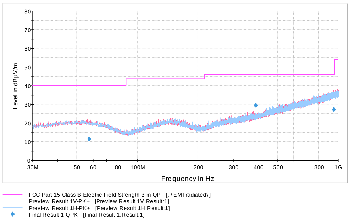
Figure 3: 30 MHz – 1000 MHz
