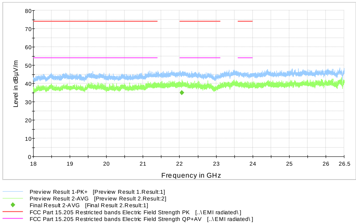
Figure 6: 18 GHz – 26.5 GHz
