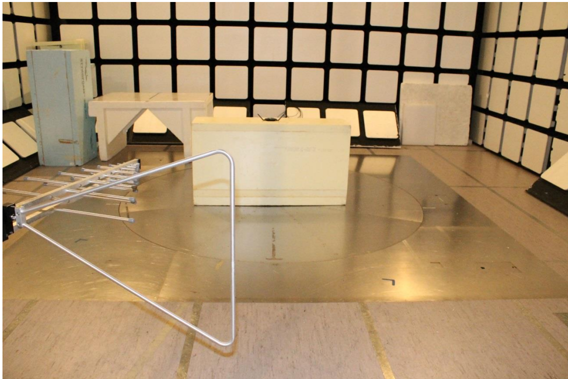
Photograph 2. Radiated Spurious Emissions 30 – 1000 MHz
