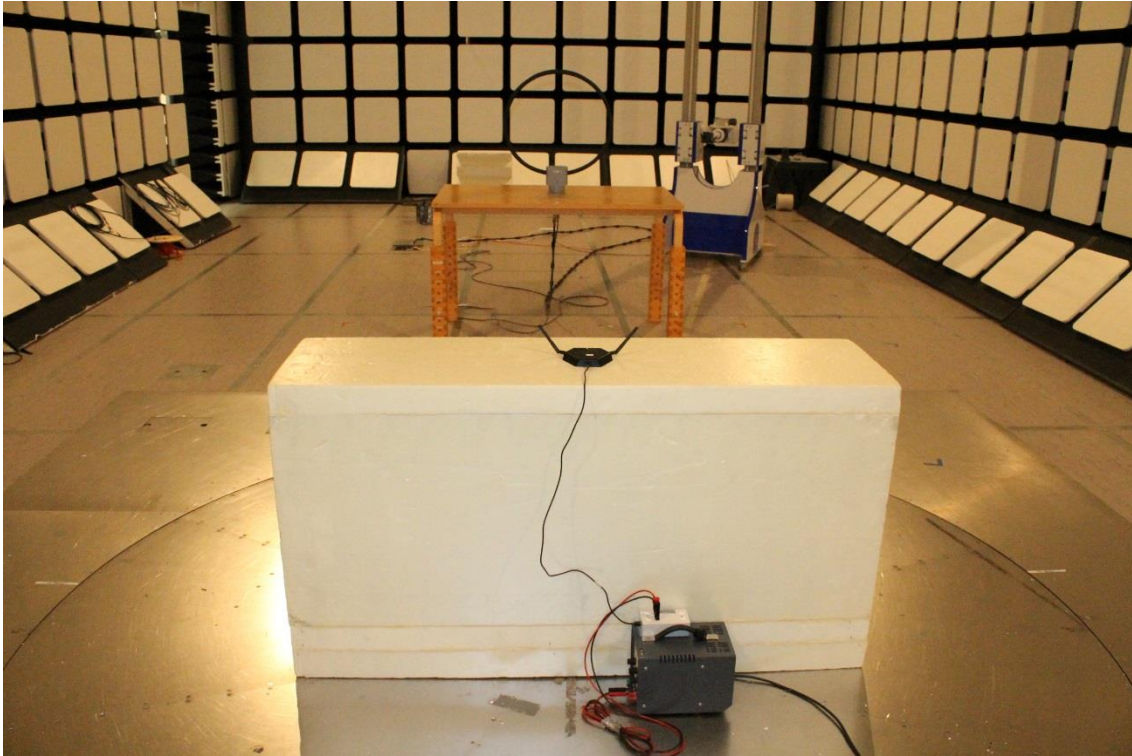
Photograph 1. Radiated Spurious Emissions 0.009 – 30 MHz
