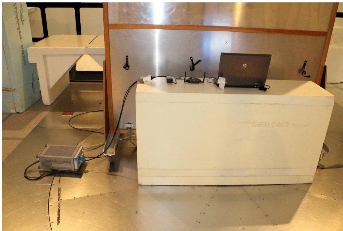
Photograph 5. Conducted Emissions
