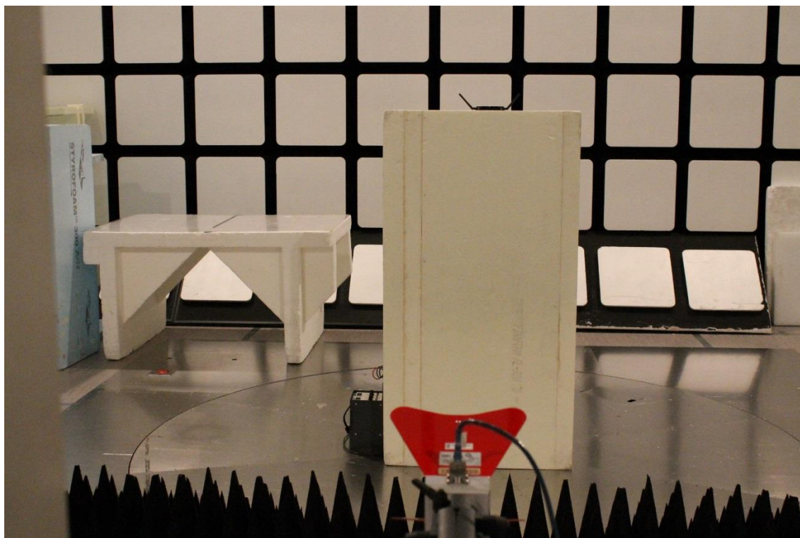
Photograph 3. Radiated Spurious Emissions 1 – 18 GHz
