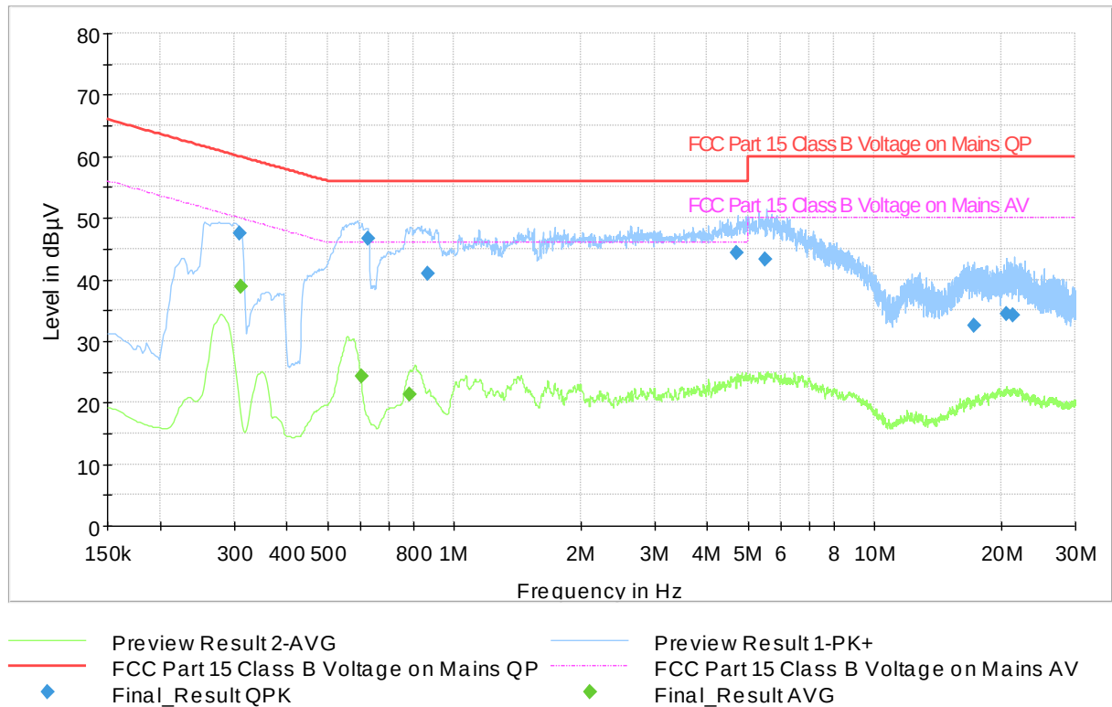
Figure 1. The measured results with peak- and average detectors at the Launch AC-port
