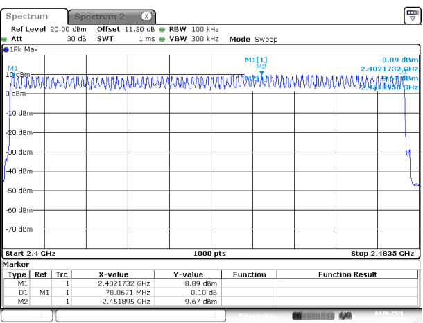
2DH1_Hopping
