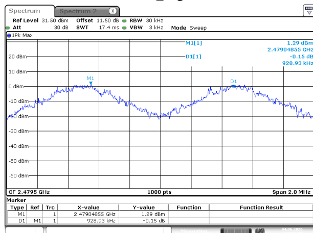
DH1_High
