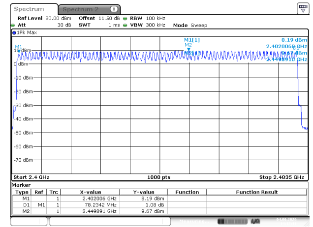
3DH1_Hopping
