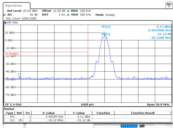
BLE_1M_Low_Channel
