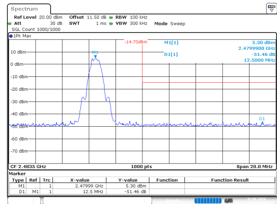
BLE_1M_High_Channel
