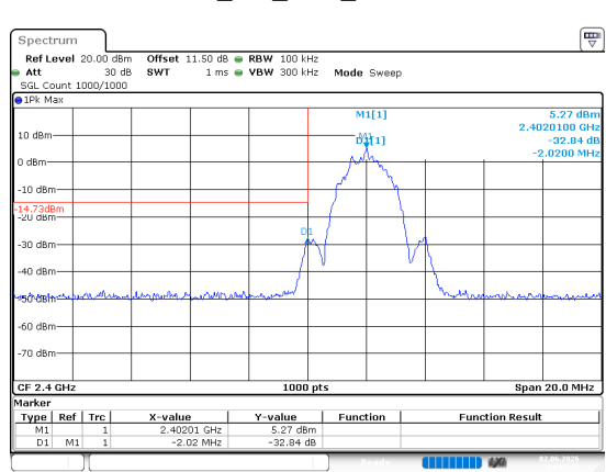
BLE_2M_Low_Channel
