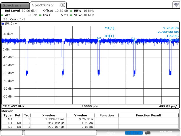
802.11n40_2437MHz
