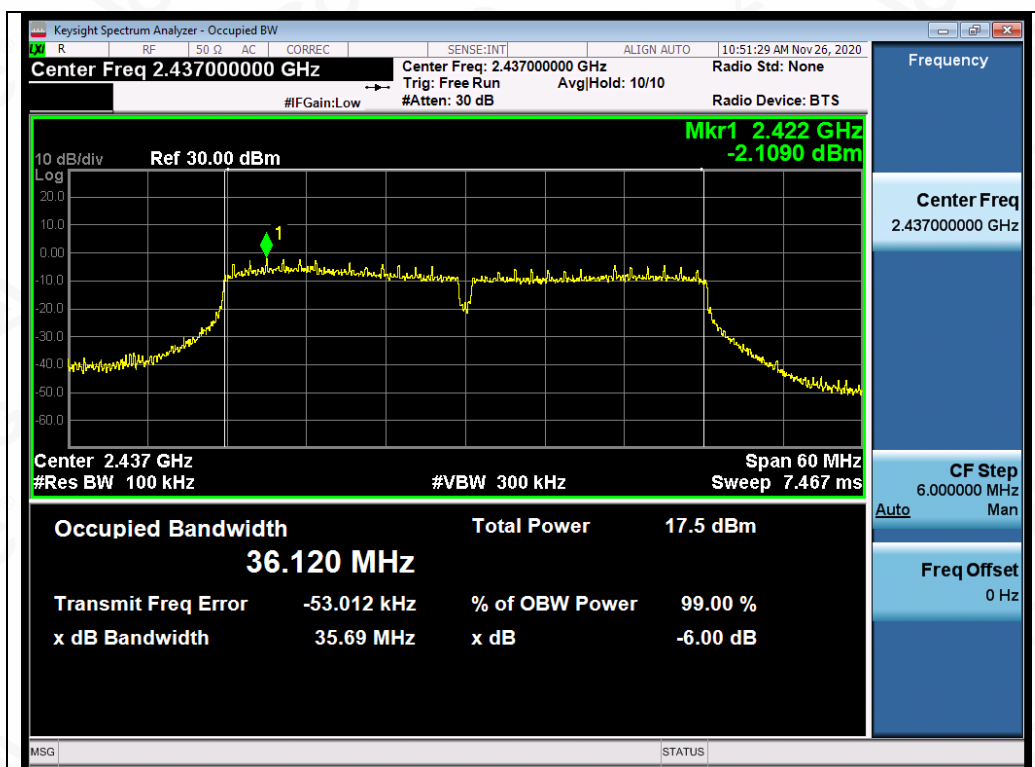
Test_Graph_802.11n40_ANT1_2437_MCS0_DTSBW
