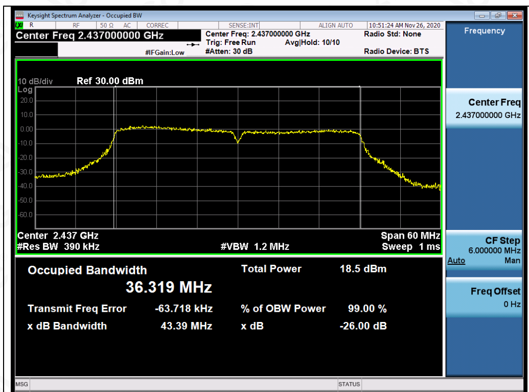
Test_Graph_802.11n40_ANT1_2437_MCS0_OBW
