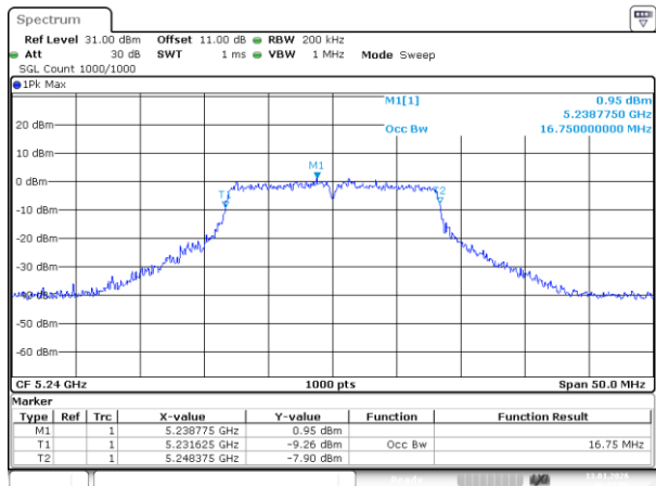
802.11a_5240MHz
