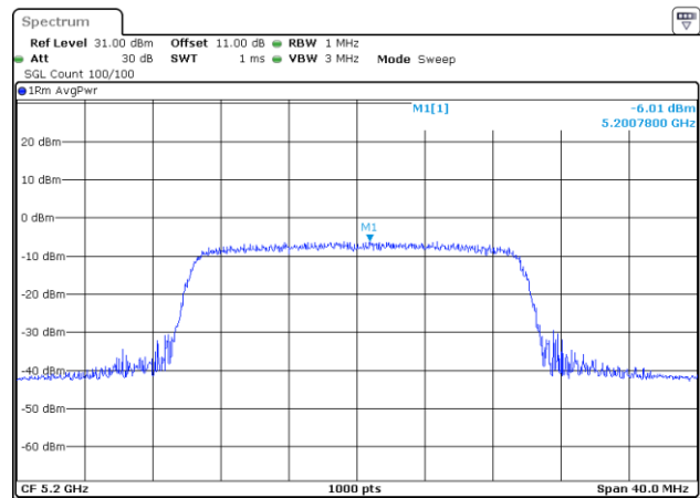
802.11ax20_5200MHz_RU_Full
