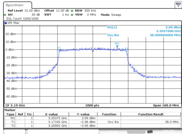
802.11ax40_5190MHz_RU_FULL
