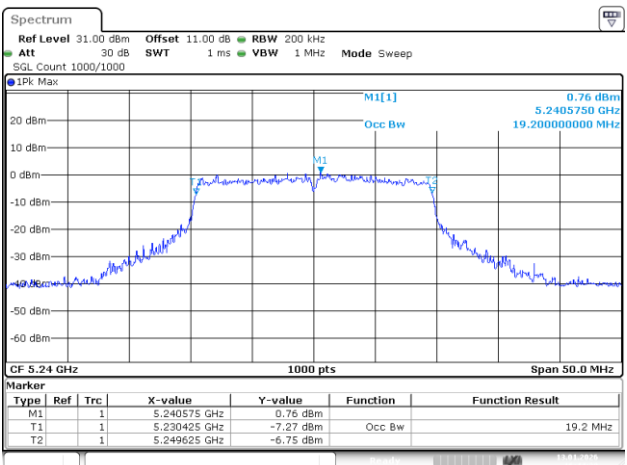
802.11ax20_5240MHz_RU_Full
