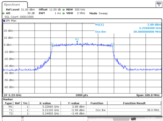
802.11ax40_5230MHz_RU_FULL
