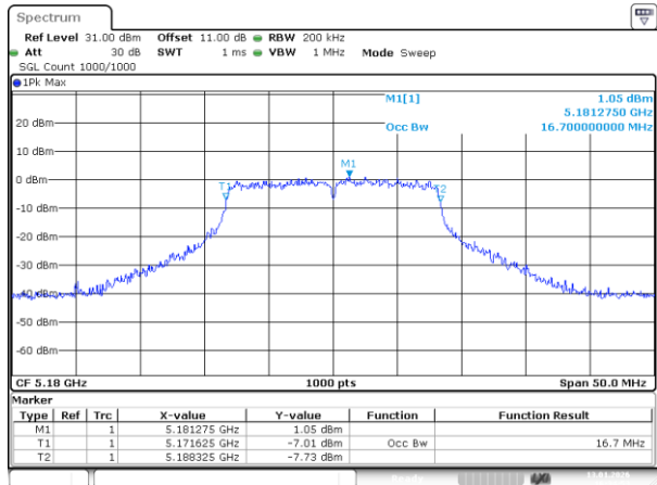
802.11a_5180MHz
