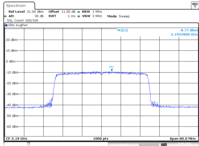
802.11ax40_5190MHz_RU_FULL
