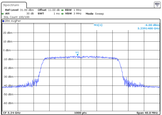
802.11ax20_5240MHz_RU_Full
