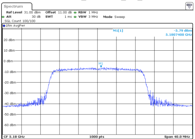
802.11ax20_5180MHz_RU_Full
