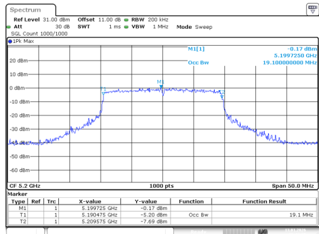
802.11ax20_5200MHz_RU_Full
