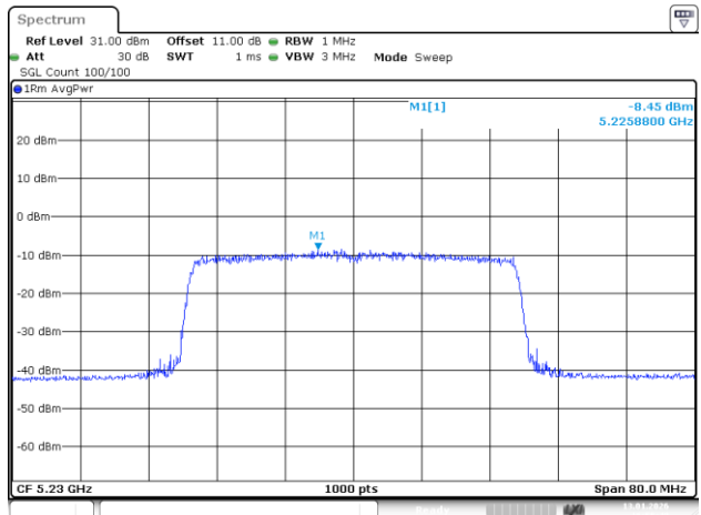
802.11ax40_5230MHz_RU_FULL
