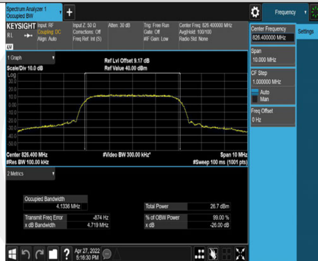
Band5-4132-2-4.719
