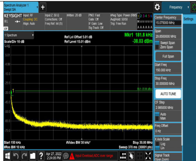
Band2-9400-4-0.15~30MHz
