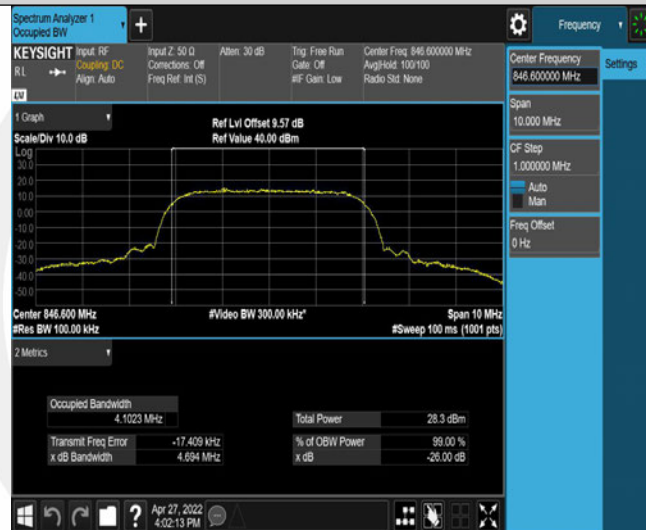
Band5-4233-3-4.694
