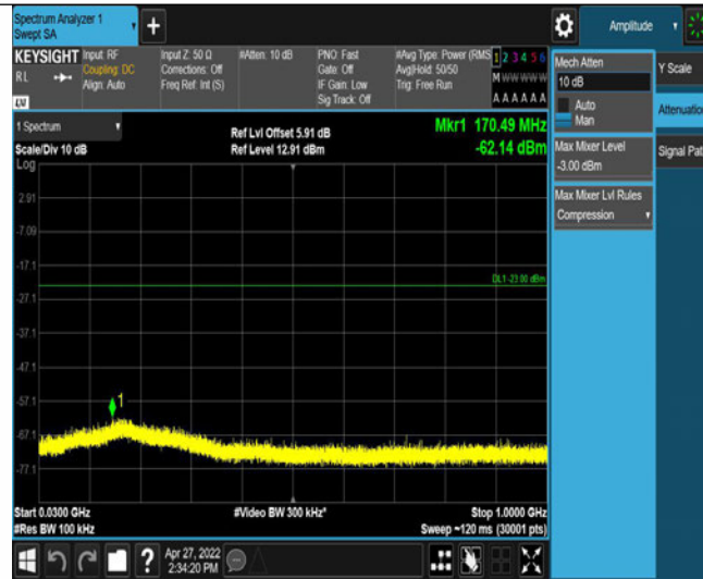
Band2-9538-5-30~1000MHz
