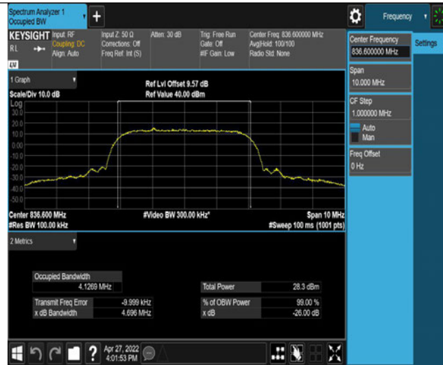
Band5-4183-3-4.696
