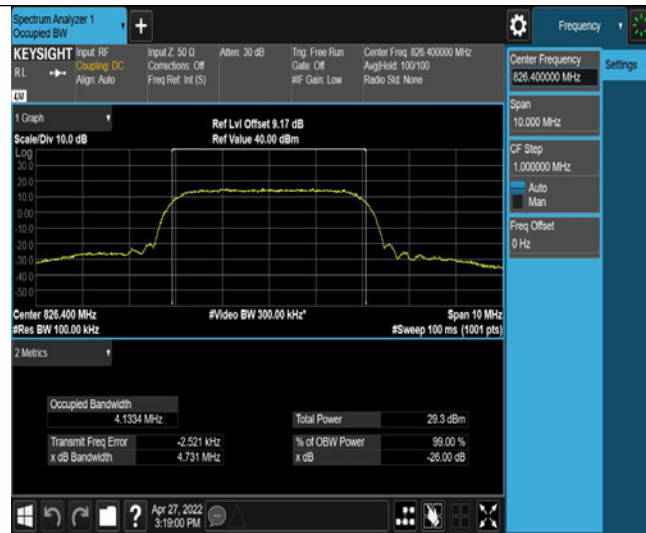
Band5-4132-4.731
