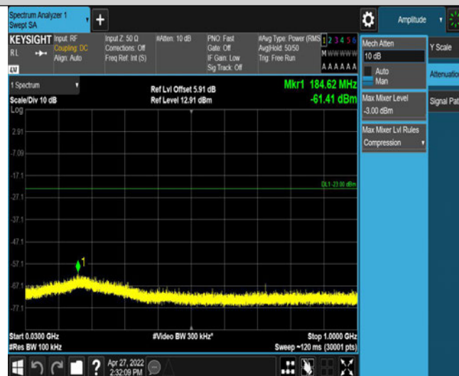
Band2-9400-5-30~1000MHz
