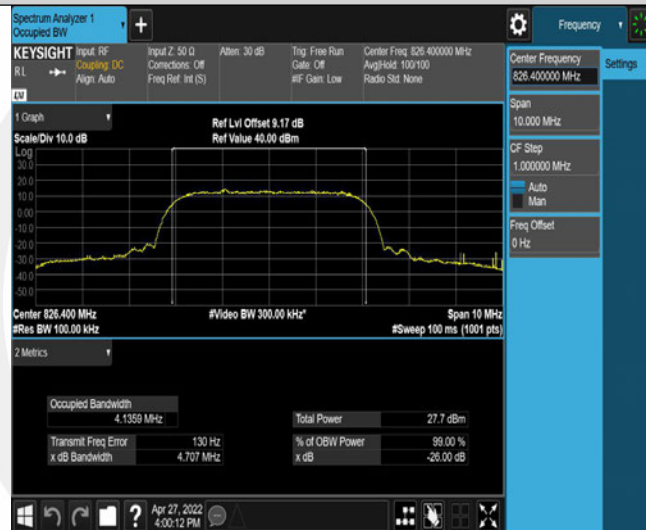
Band5-4132-2-4.707
