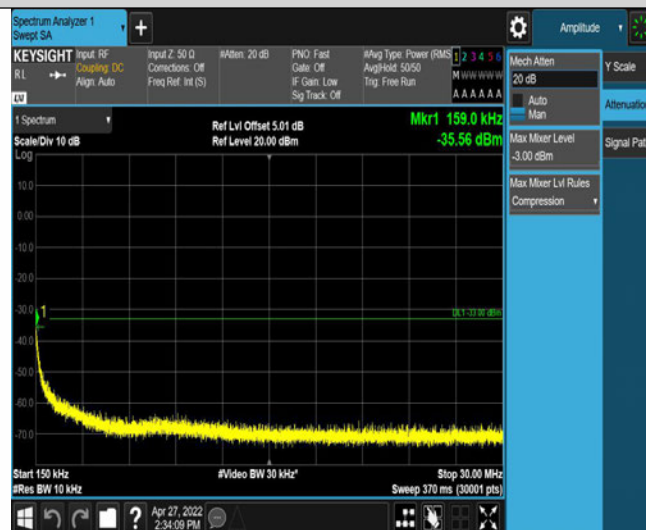
Band2-9538-5-0.15~30MHz
