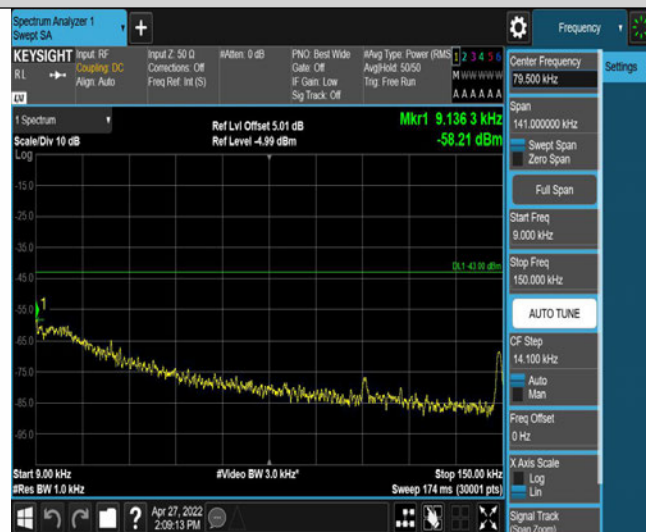
Band2-9538-2-0.009~0.15MHz
