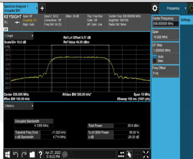
Band5-4183-4.714
