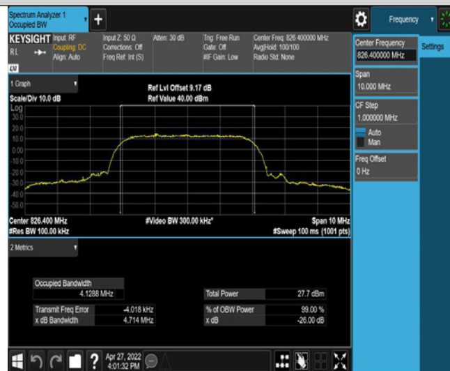
Band5-4132-3-4.714
