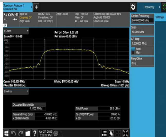
Band5-4233-1-4.696
