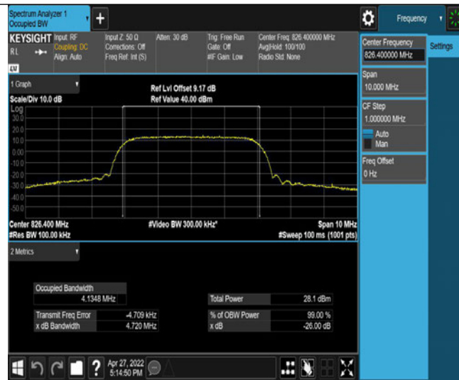
Band5-4132-1-4.720
