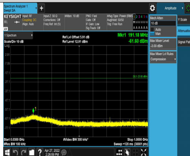
Band2-9538-4-30~1000MHz
