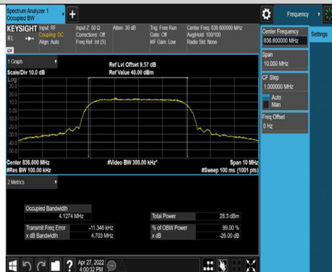
Band5-4183-2-4.703
