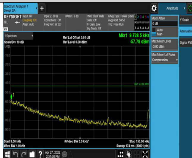
Band2-9400-5-0.009~0.15MHz
