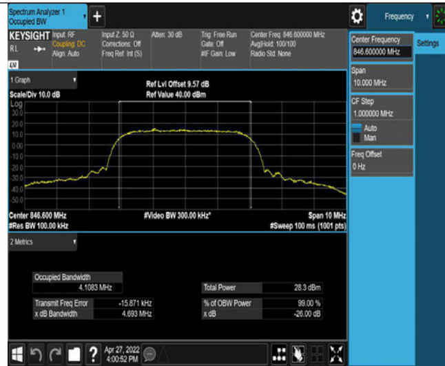
Band5-4233-2-4.693
