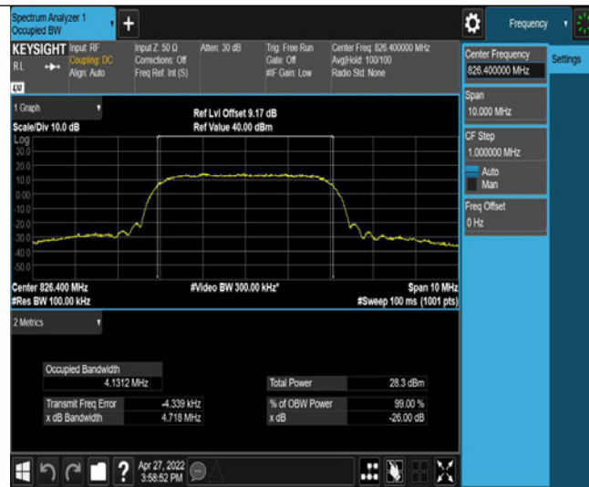
Band5-4132-1-4.718
