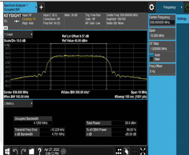
Band5-4183-1-4.701
