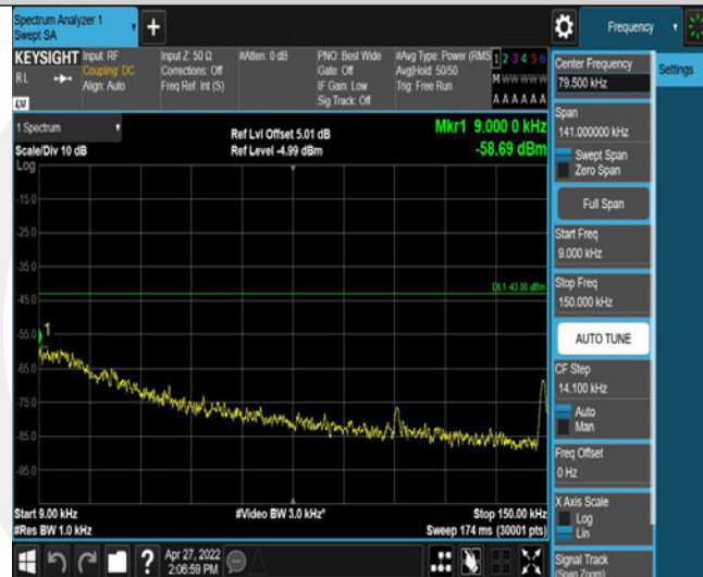
Band2-9400-2-0.009~0.15MHz
