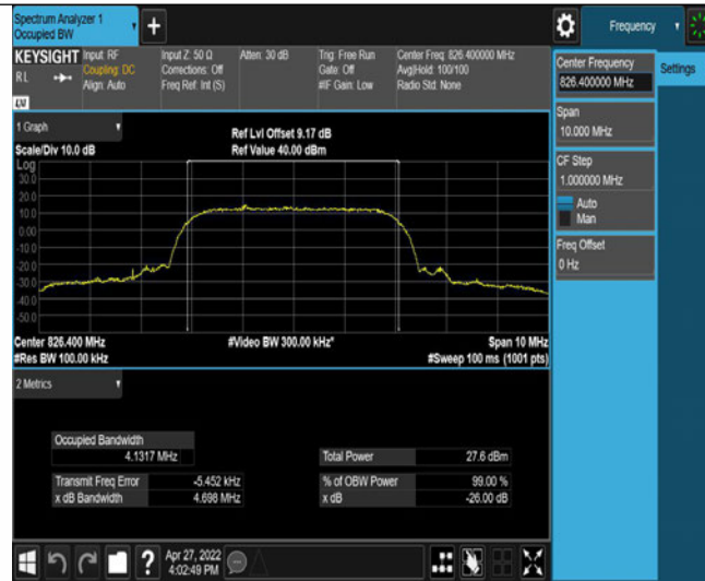
Band5-4132-4-4.698
