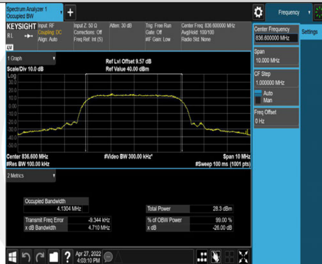
Band5-4183-4-4.710
