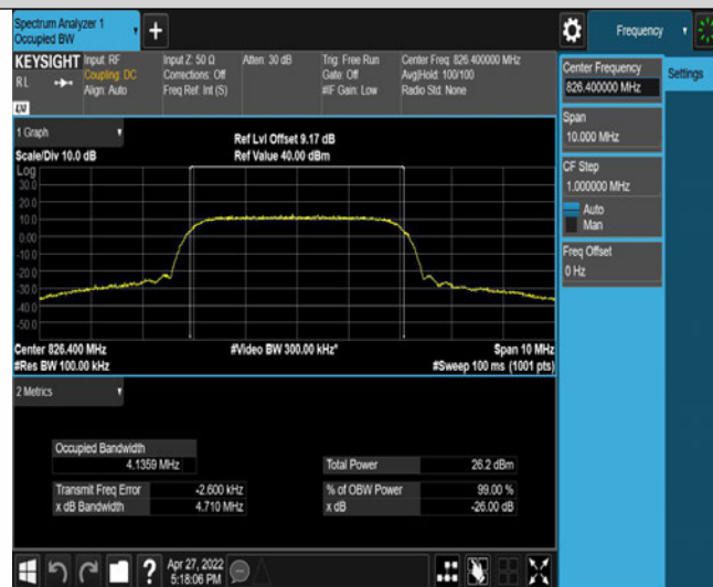
Band5-4132-3-4.710
