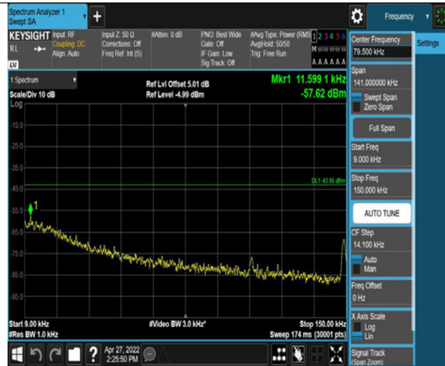
Band2-9538-4-0.009~0.15MHz
