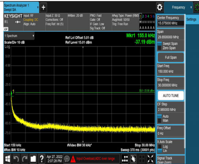
Band2-9400-2-0.15~30MHz
