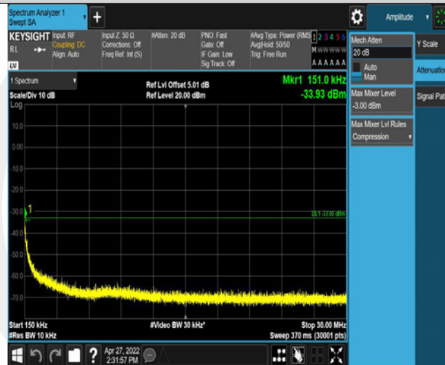
Band2-9400-5-0.15~30MHz
