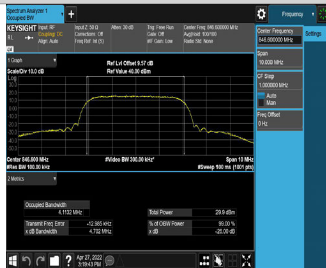
Band5-4233-4.702
