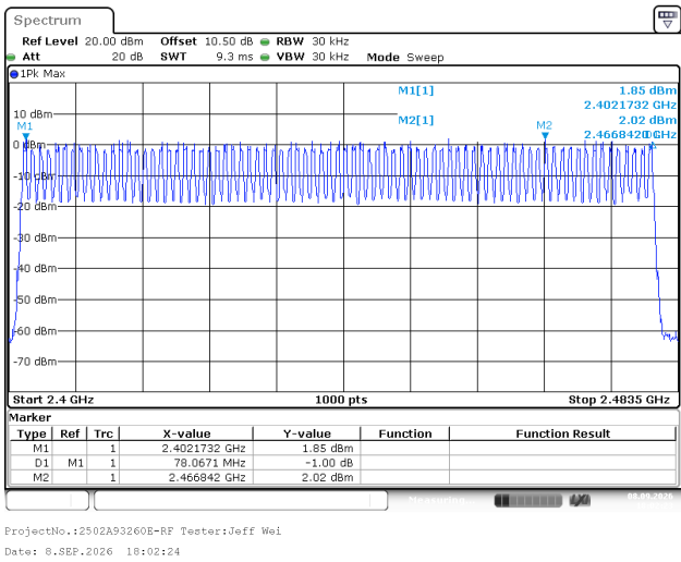
BDR_DH1_Hopping
