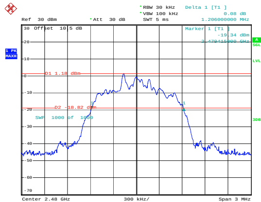
3EDR_DH1_High
