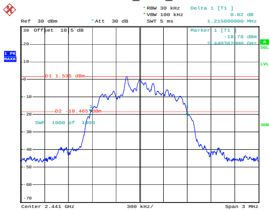
2EDR_DH1_Middle
