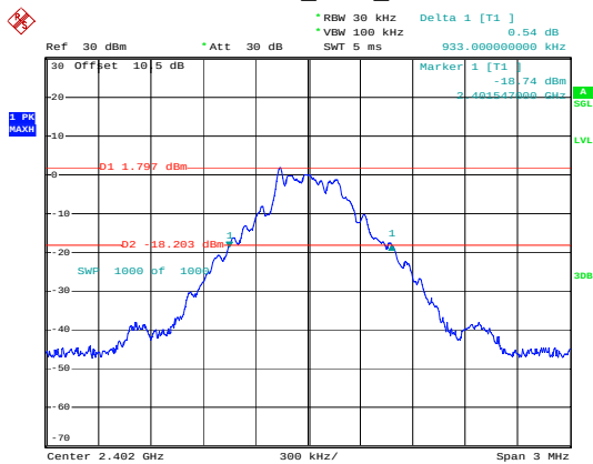
BDR_DH1_Low
