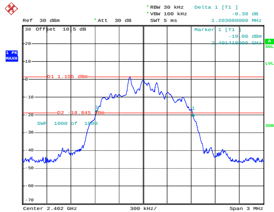
3EDR_DH1_Low
