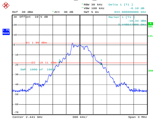
BDR_DH1_Middle
