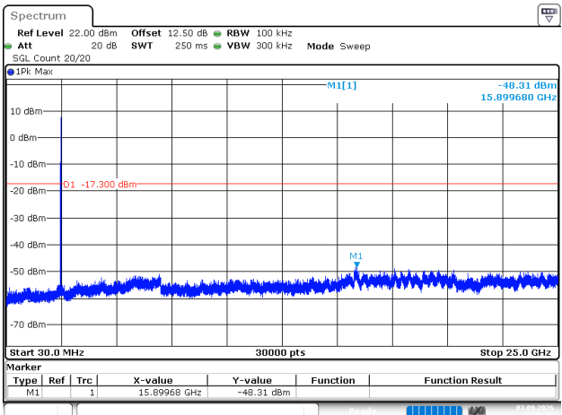
BDR_DH1_High
