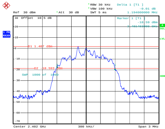
2EDR_DH1_Low
