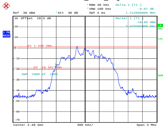
2EDR_DH1_High
