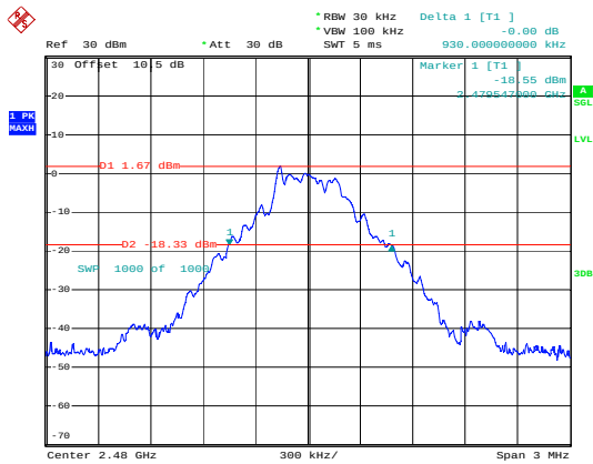
BDR_DH1_High
