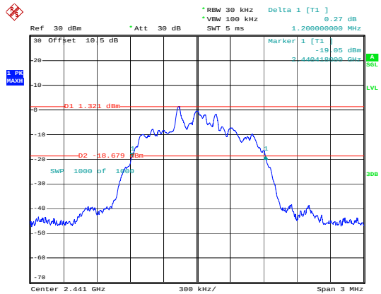
3EDR_DH1_Middle
