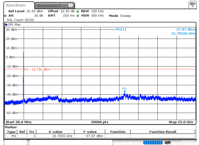
802.11g_2462MHz
