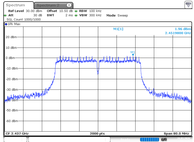
802.11n40_2437MHz
