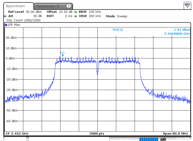
802.11n40_2452MHz
