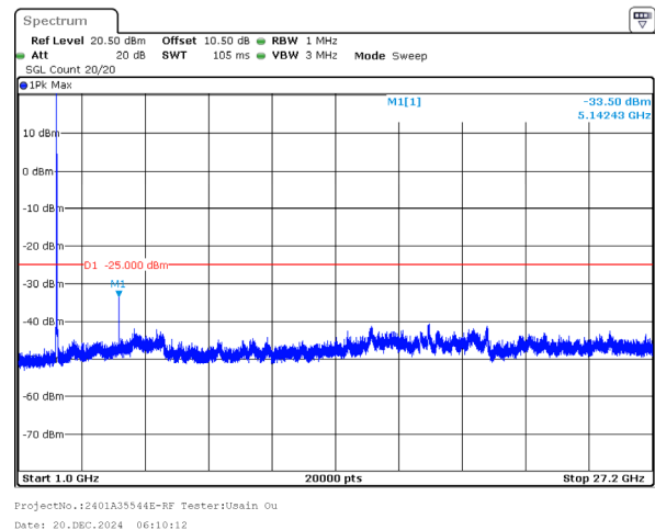
5MHz_Middle_QPSK_1@0(1GHz~27.2GHz)
