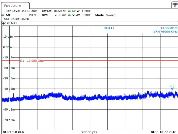
15MHz_High_QPSK_75@0(1GHz~18.55GHz)
