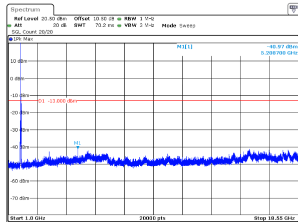
20MHz_High_QPSK_1@0(1GHz~18.55GHz)
