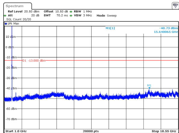
20MHz_High_QPSK_100@0(1GHz~18.55GHz)
