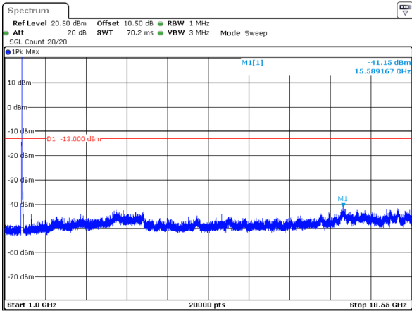
15MHz_Middle_QPSK_75@0(1GHz~18.55GHz)
