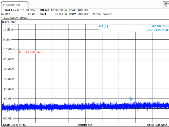
15MHz_High_QPSK_1@0(30MHz~1GHz)
