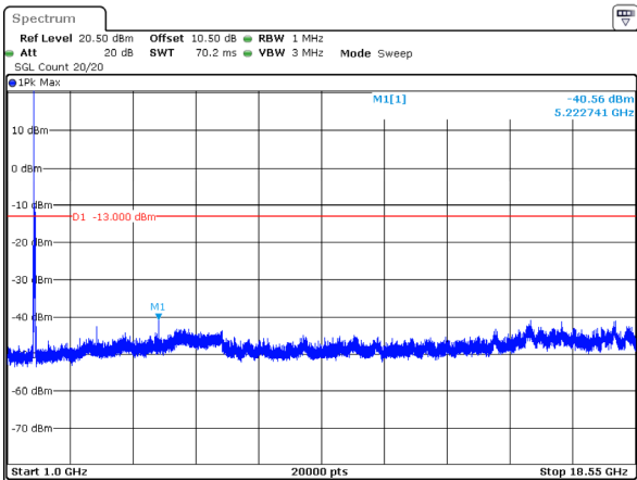
15MHz_High_QPSK_1@0(1GHz~18.55GHz)
