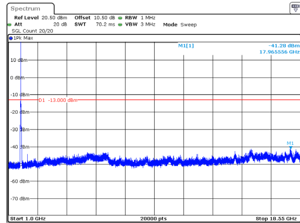
20MHz_Middle_QPSK_100@0(1GHz~18.55GHz)
