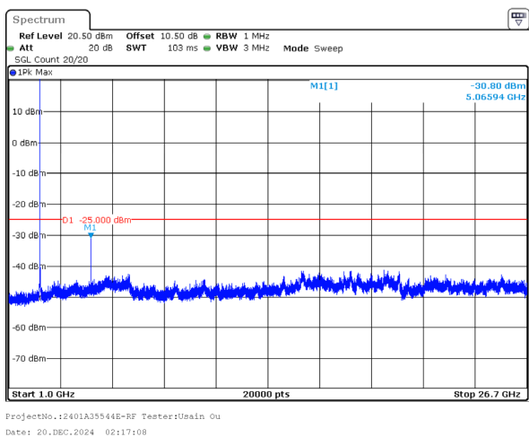
5MHz_Middle_QPSK_1@0(1GHz~26.7GHz)
