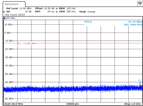
20MHz_Middle_QPSK_100@0(30MHz~1GHz)
