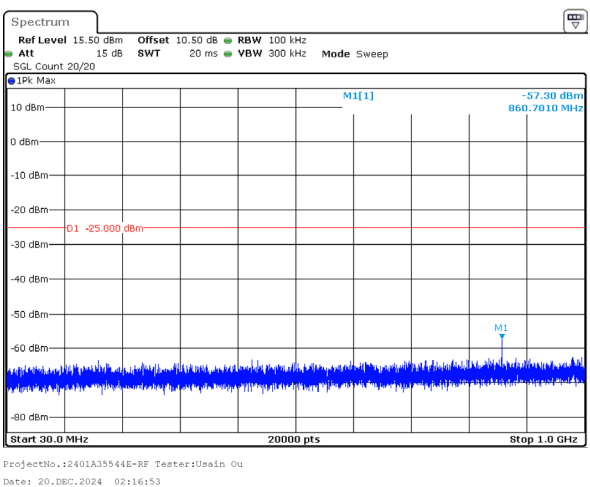
5MHz_Middle_QPSK_1@0(30MHz~1GHz)
