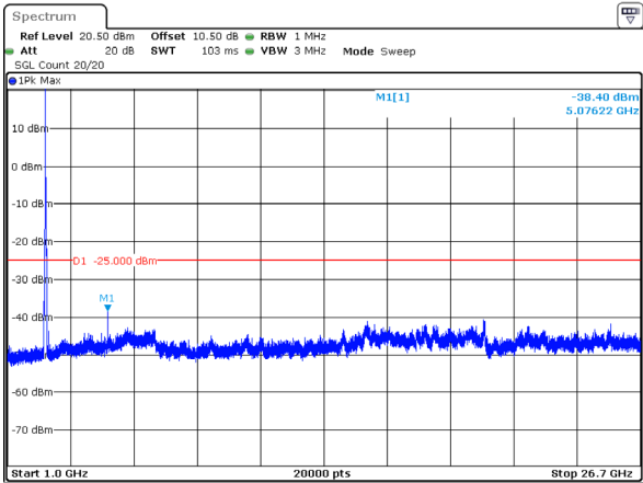
15MHz_Middle_QPSK_75@0(1GHz~26.7GHz)
