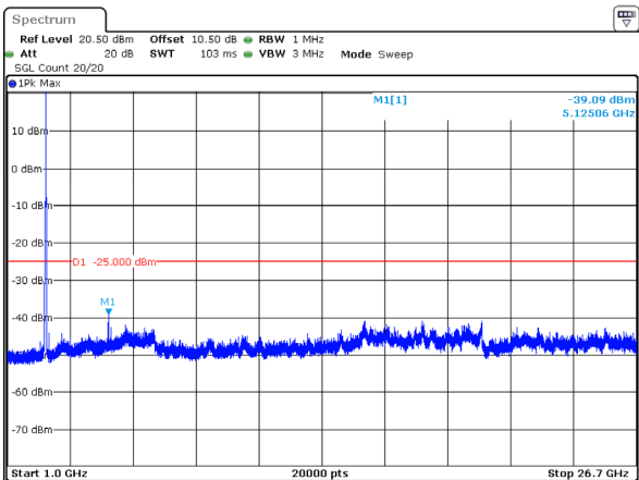
15MHz_High_QPSK_75@0(1GHz~26.7GHz)
