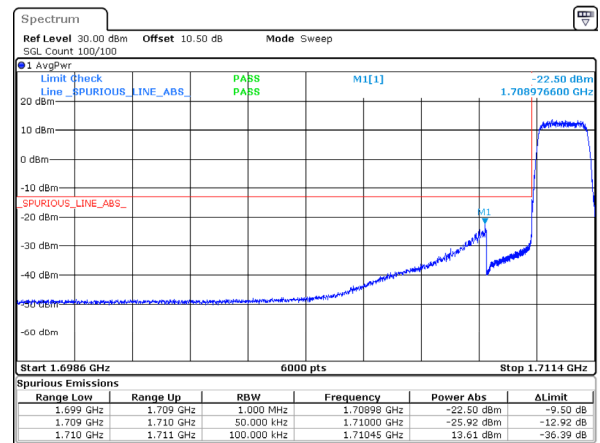
1.4MHz_Low_16QAM_6@0
