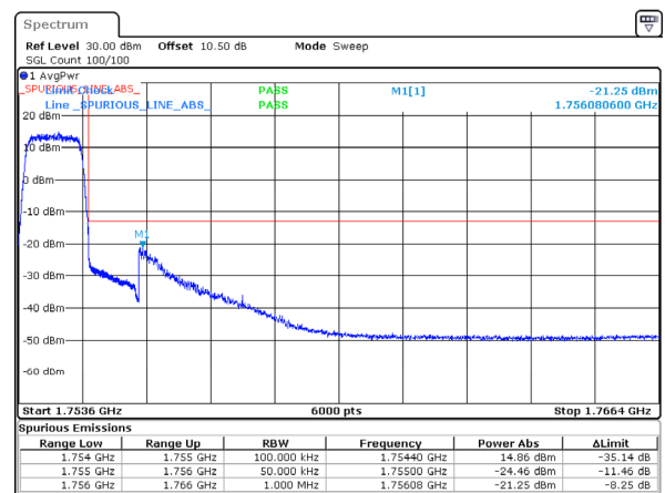
1.4MHz_High_QPSK_6@0
