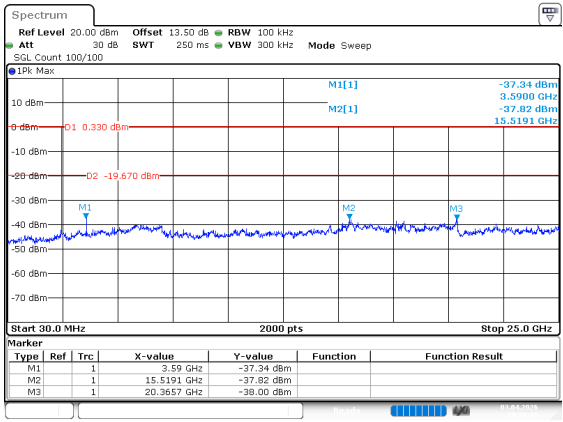
802.11g_2472MHz
