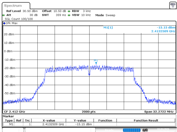
802.11g_2412MHz
