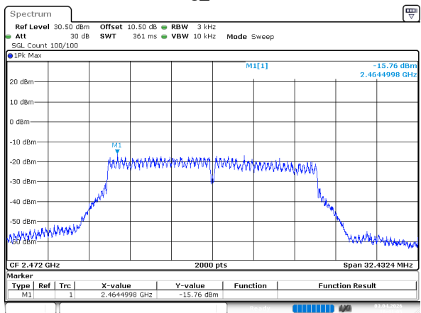
802.11g_2472MHz
