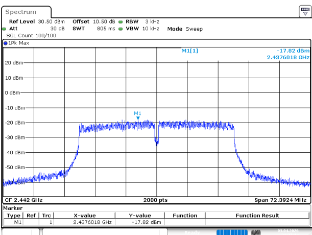
802.11n40_2442MHz
