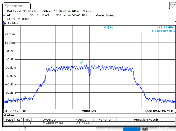
802.11g_2442MHz
