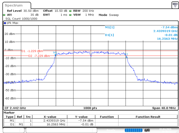
802.11g_2442MHz
