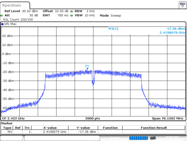
802.11n40_2422MHz
