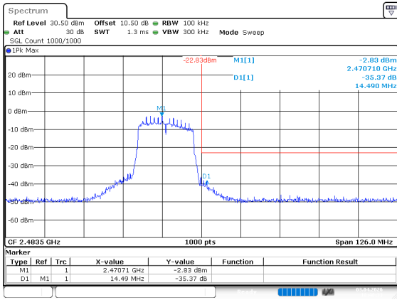
802.11n20_2472MHz
