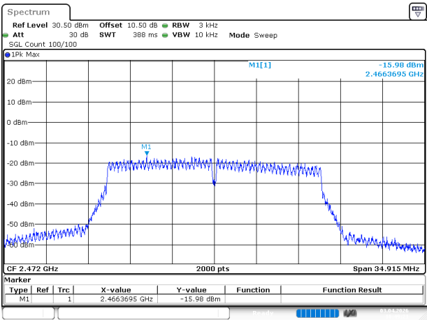
802.11n20_2472MHz
