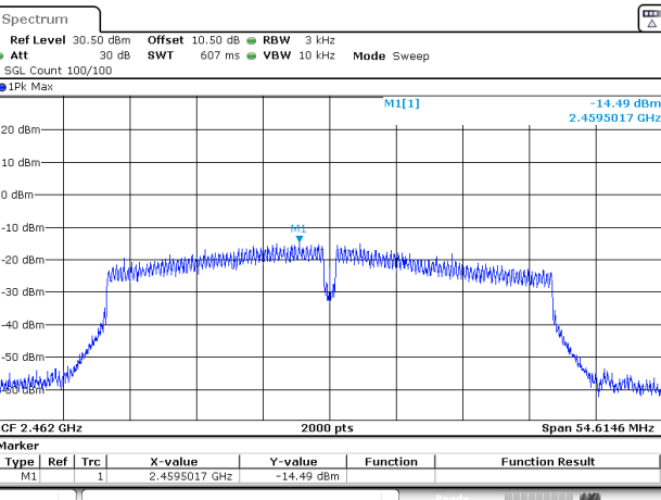
802.11n40_2462MHz
