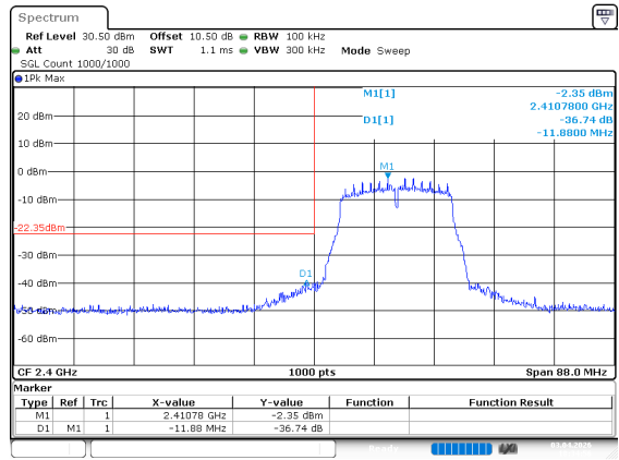
802.11g_2412MHz
