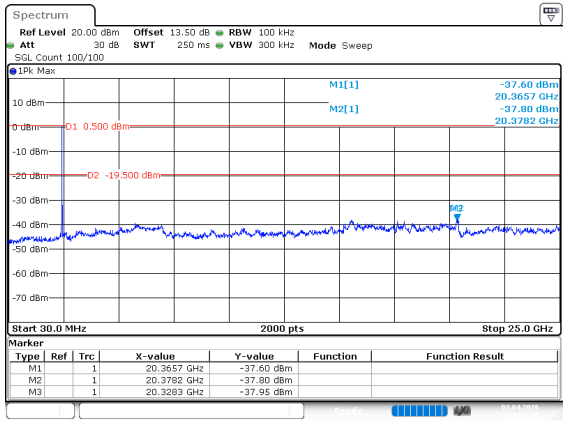
802.11g_2442MHz
